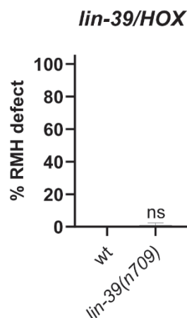
Figure 54. lin-39/HOX , like egl-5/HOX , is not required for G1-to-RMH. Histograms summarising the percentage of absence of RMH neurons based on cho-1 expression in lin-39(n709Ts) mutants scored at 25°C. N=3; mean and SD shown.
