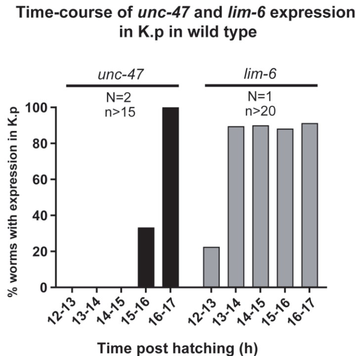
Figure 33. Time-course of unc-47/VGAT and lim-6/LMX expression in K.p. K divides 11.5 h post hatching and while unc-47 terminal differentiation gene is expressed after 15-16 h post hatching, lim-6 terminal selector transcription factors is already expressed 1 hour after K division.
