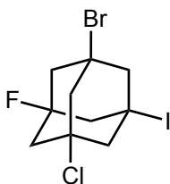
Figure 14: Polyhaloadamantane synthesized following PTC multi-steps.
