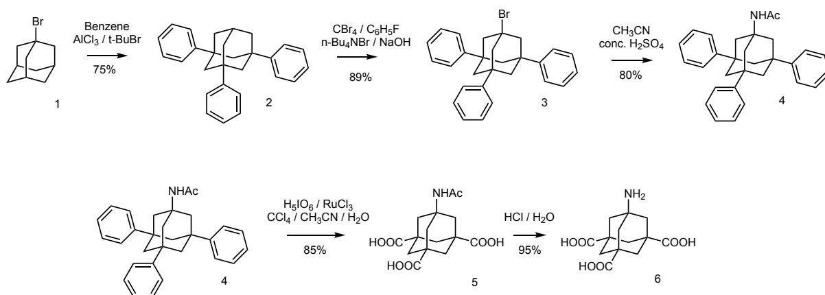
Scheme 1: Synthesis of adamantane (3+1) building block, the first generation dendron.
