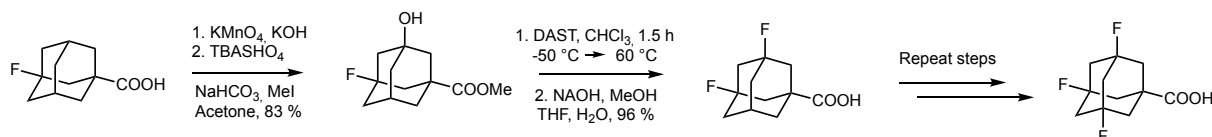
Figure 11: Adamantane fluorination using step-by-step strategy.
