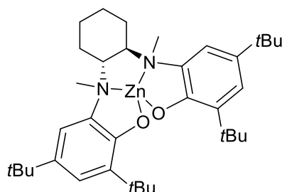
Figure 138: Complex 33-Zn
