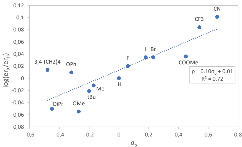
Figure 67: \sigma_p -Hammett plot of the enantioselectivity of the NBE-catalysed addition of \text{ZnMe}_2 to substituted benzaldehydes.
