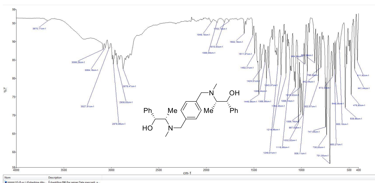
(4S,5R)-3-benzyl-2,2,4-trimethyl-5-phenyloxazolidine 2:
