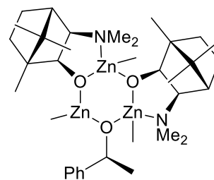
Figure 6: Presumed (DAIB-ZnMe) 2 -zinc alkoxide adduct.
