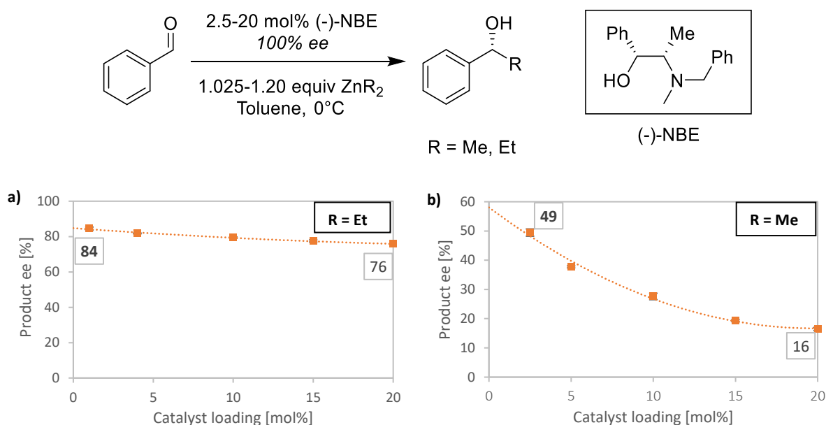
Figure 31: Catalyst loading screening of the (-)-NBE catalyzed addition of a) \text{ZnEt}_2 or b) \text{ZnMe}_2 to benzaldehyde. The trendlines (2 nd order polynomial) are intended for illustration purposes only.
