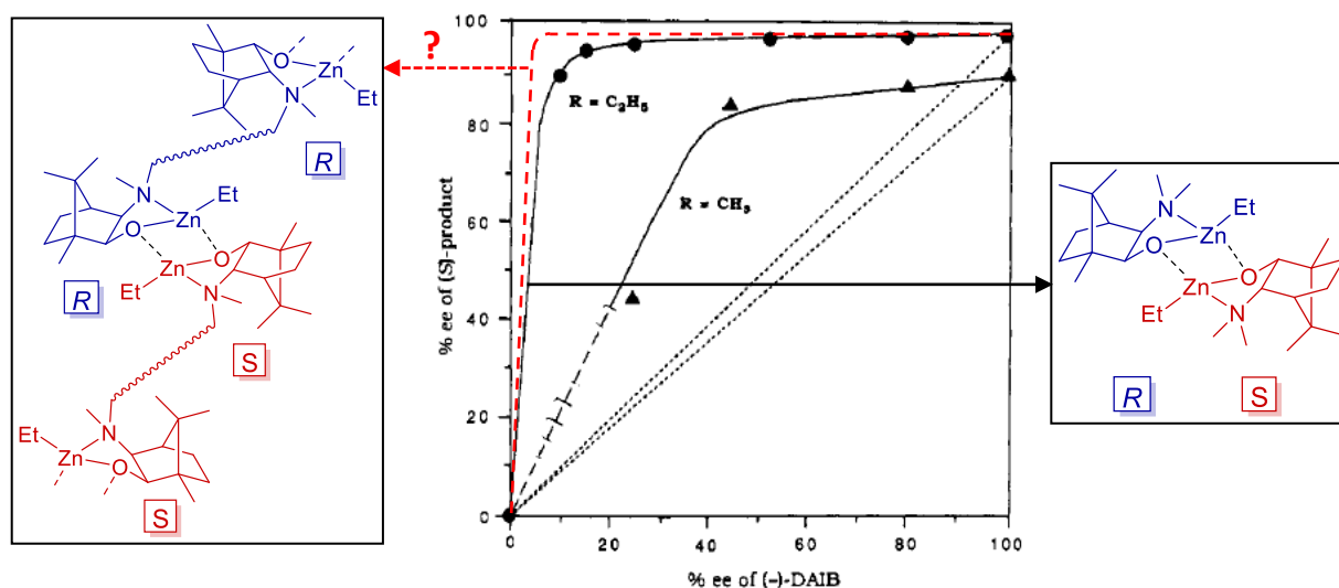
Figure 8: Scheme for the stipulated (+)-NLE [22] amplification by using a ditopic version of DAIB capable of forming heterochiral metallopolymer.
