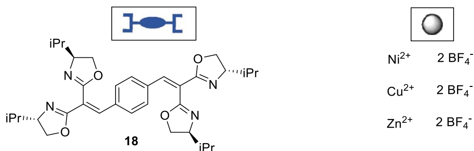
Figure 99: Scheme for ligand 18 and the metals salts used to form chiral metallopolymer.
