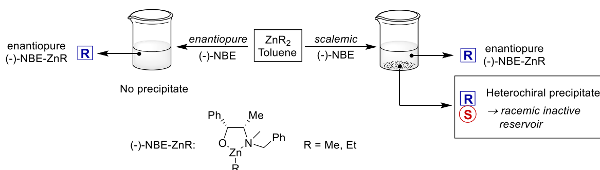
Figure 29: Presence or absence of a precipitate upon reaction of enantiopure or scalemic (-)\text{-NBE} with \text{ZnR}_2 in toluene. The precipitate with a scalemic ligand corresponds to a racemic, heterochiral aggregate while the supernatant contains only enantiopure \text{NBE-ZnR} .
