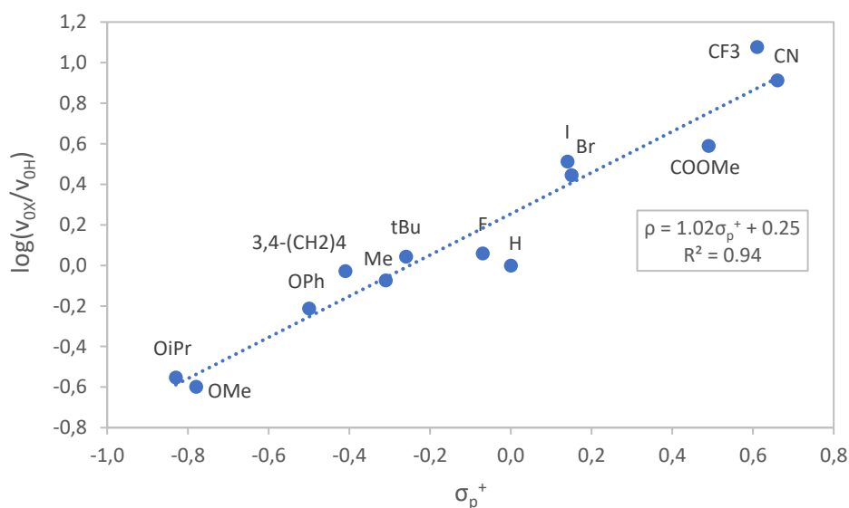
Figure 66: \sigma_p^+ -Hammett plot of the NBE-catalysed addition of \text{ZnMe}_2 to substituted benzaldehydes.
