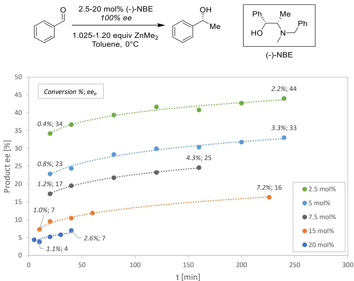
Figure 47: Time-dependent ee_p evolution of the (-)-NBE-catalysed addition of \text{ZnMe}_2 to benzaldehyde at various catalyst loadings. The italic percentages indicate the approx. benzaldehyde conversion. The trendlines are for illustration purposes only.
