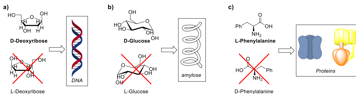
Figure 16: Scheme depicting the homochirality of biomolecules. a) DNA consists only of D-deoxyribose, b) polysaccharides, such as amylose, only of D-glucose, c) proteins only of L-amino acids.
