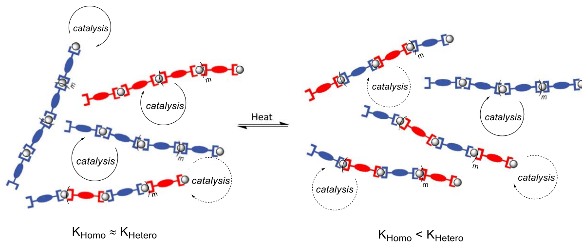
Figure 88: Scheme for the temperature-dependent formation of heterochiral metallopolymer out of homochiral R and S -metallopolymer. The heterochiral polymers must be less active than the homochiral polymers in order to allow the emergence of a (+)-NLE.
