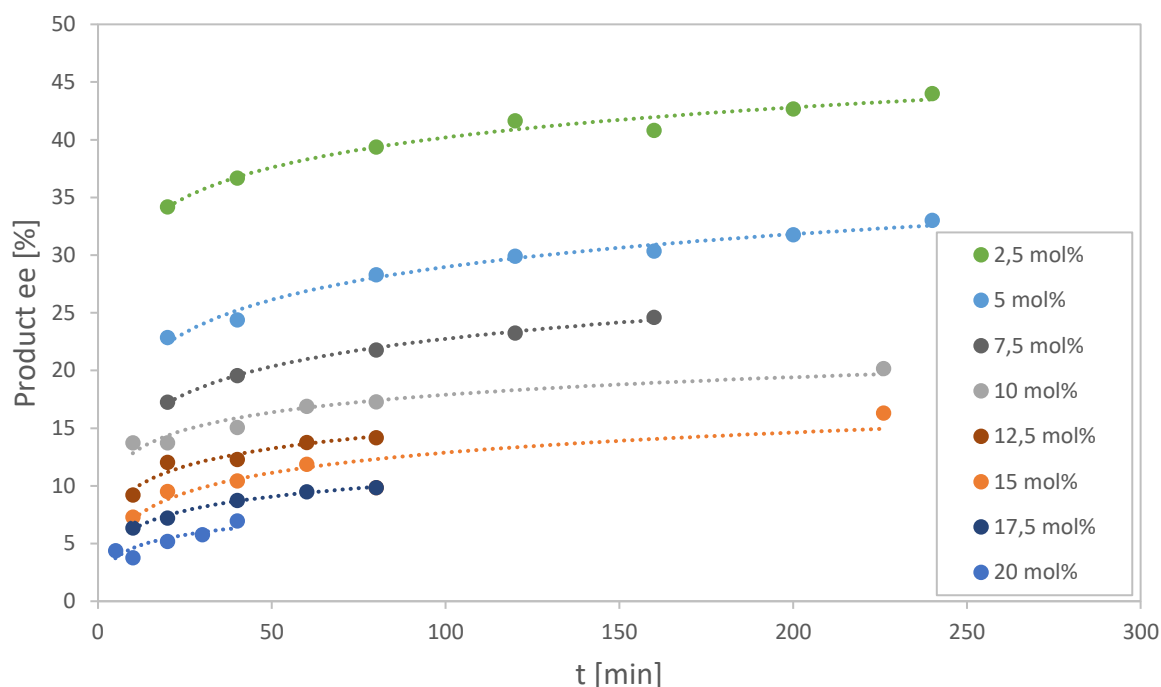
Figure 130: Complete time-dependent ee_p evolution of the (-)-NBE-catalysed addition of ZnMe_2 to benzaldehyde at various catalyst loadings.
