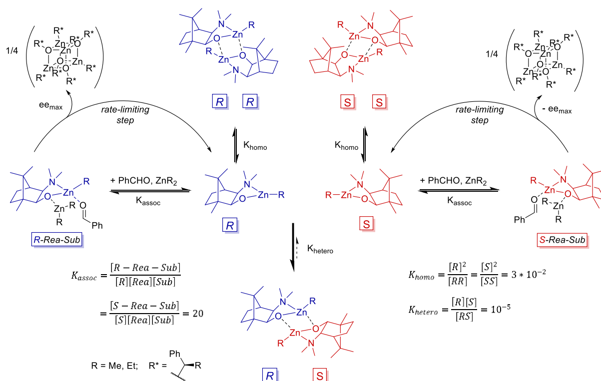
Figure 9: Mechanistic pathway for the (-)-DAIB-catalysed addition of dialkylzinc to benzaldehyde. The values given for K_{\text{assoc}} , K_{\text{Homo}} and K_{\text{Hetero}} are those for the (-)-DAIB-ZnMe complex at 40°C. [29]
