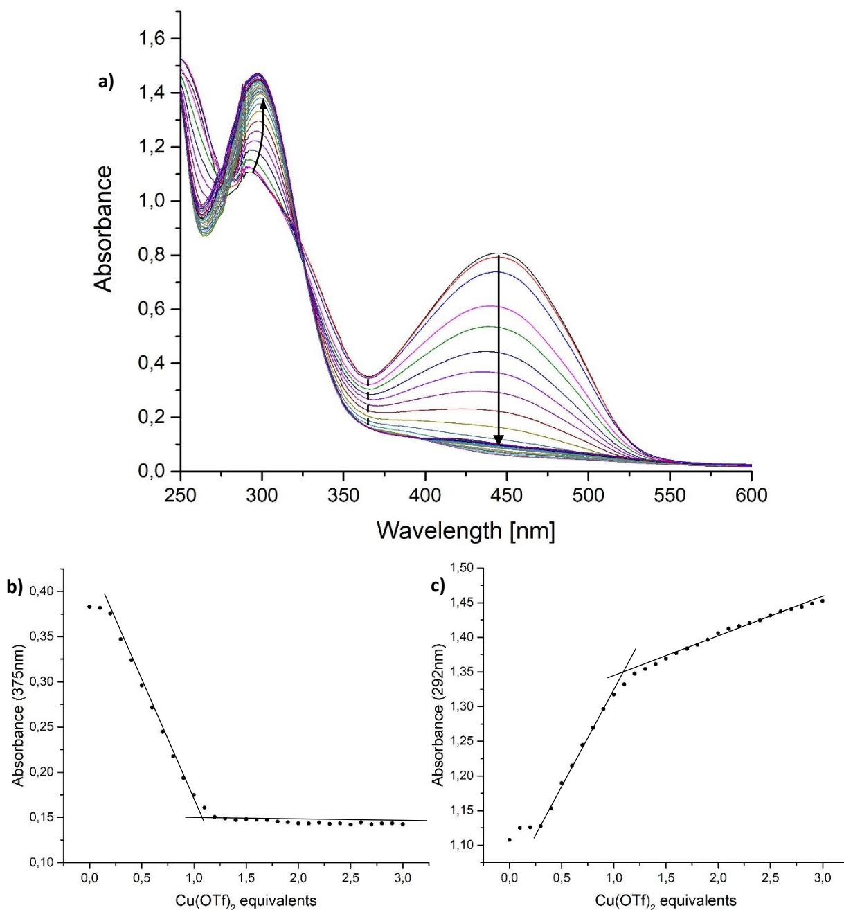
Figure 125: a) UV-vis titration of ligand 26 ( 5.74 \cdot 10^{-5} M in THF) with \text{Cu}(\text{OTf})_2 -aliquots (0.1 equiv. each); evolution of the absorbance at b) 375 nm and c) 292 nm over the course of the titration. The spectra differ slightly from those in Figure 119 in the UV-region as the titration was done in BHT-stabilised THF.
