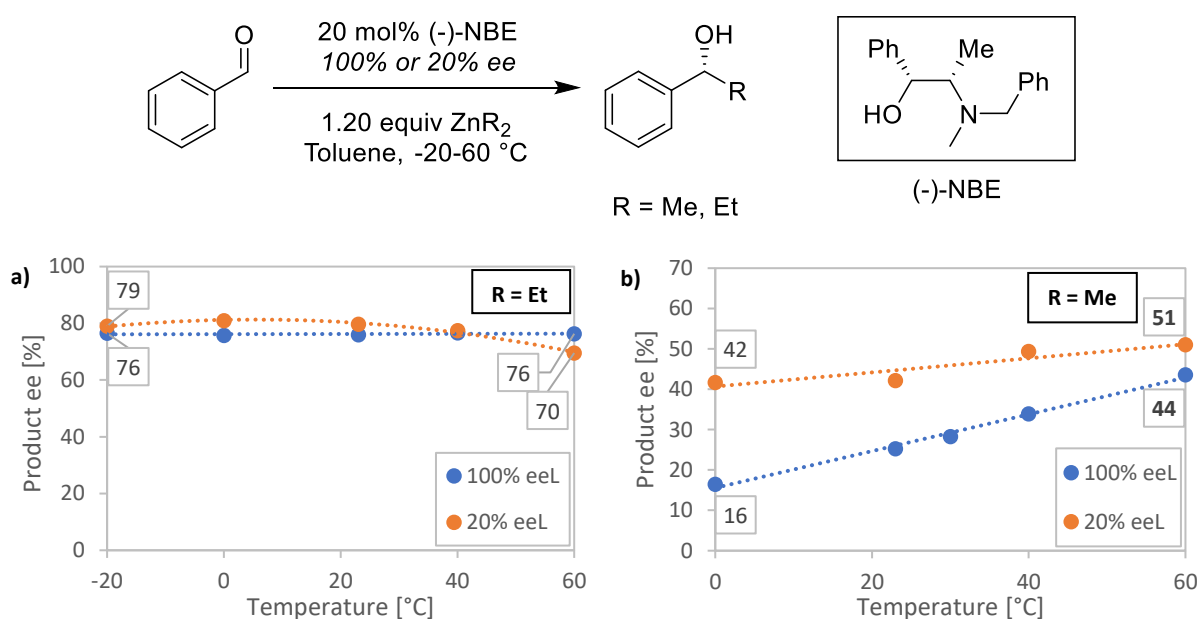
Figure 34: Temperature screening of the (-)-NBE (100% ee: blue dots, 20% ee: orange dots) catalysed addition of a) ZnEt_2 and b) ZnMe_2 to benzaldehyde. The trendlines (1 st and 2 nd order polynomial functions) are intended for illustration purposes only.
