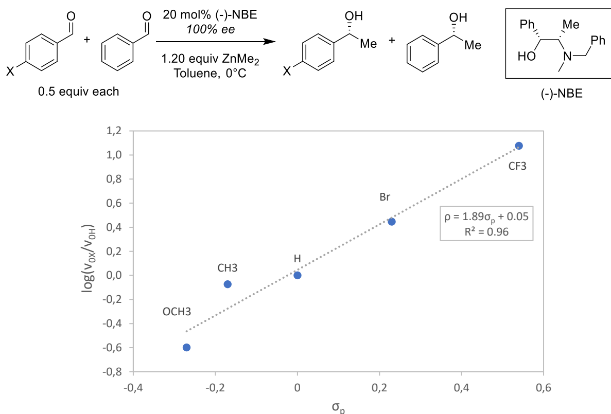
Figure 64: \sigma_p -Hammett plot of the NBE-catalysed addition of \text{ZnMe}_2 to substituted benzaldehydes.
