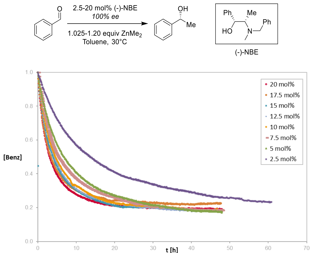
Figure 42: Kinetic profiles of the (-)-NBE-catalysed addition of \text{ZnMe}_2 to benzaldehyde with varying catalyst concentrations. The values of the benzaldehyde concentration were normalized to the initial concentration of 0.83\text{ mol/L} .
