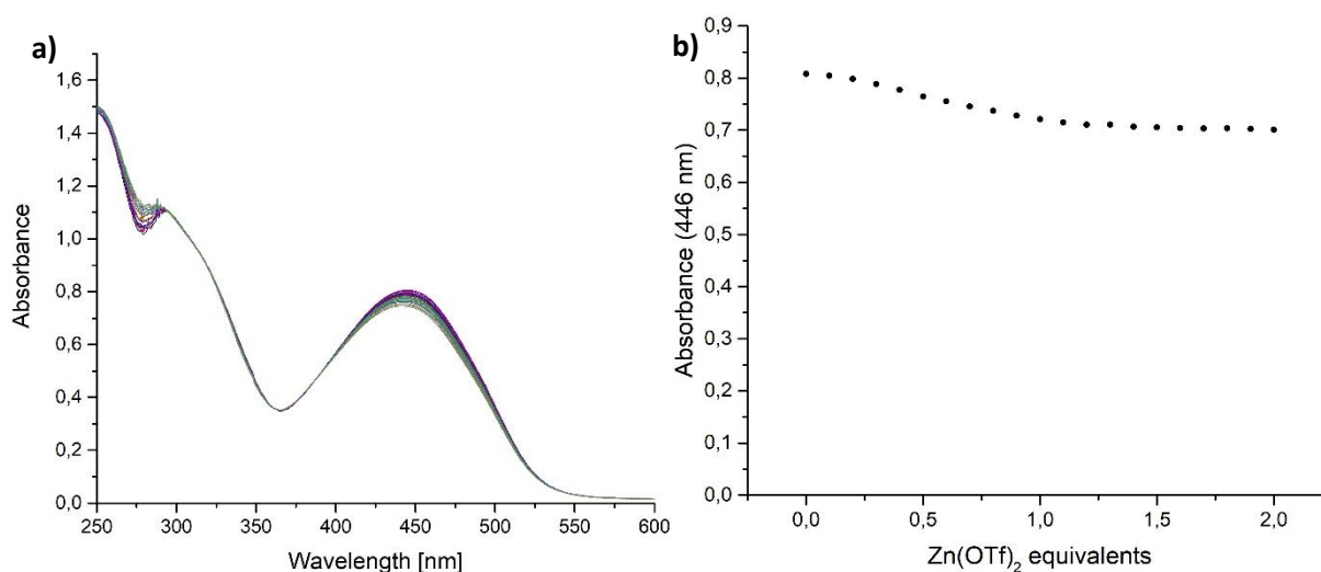
Figure 128: a) UV-vis titration of ligand 26 (5.74·10 -5 M in THF) with Zn(OTf) 2 -aliquots (0.1 equiv. each), b) evolution of the absorbance at 446 nm over the course of the titration.
