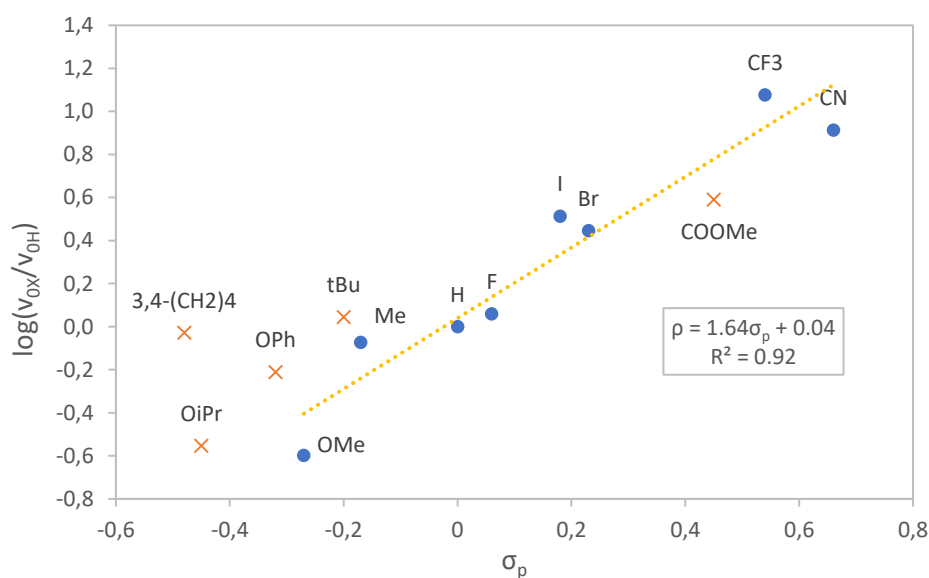
Figure 69: \sigma_p -Hammett plots of the NBE-catalysed addition of \text{ZnMe}_2 to substituted benzaldehydes. Bulky substituents (orange crosses) have been excluded from the linear fit to build the plot.
