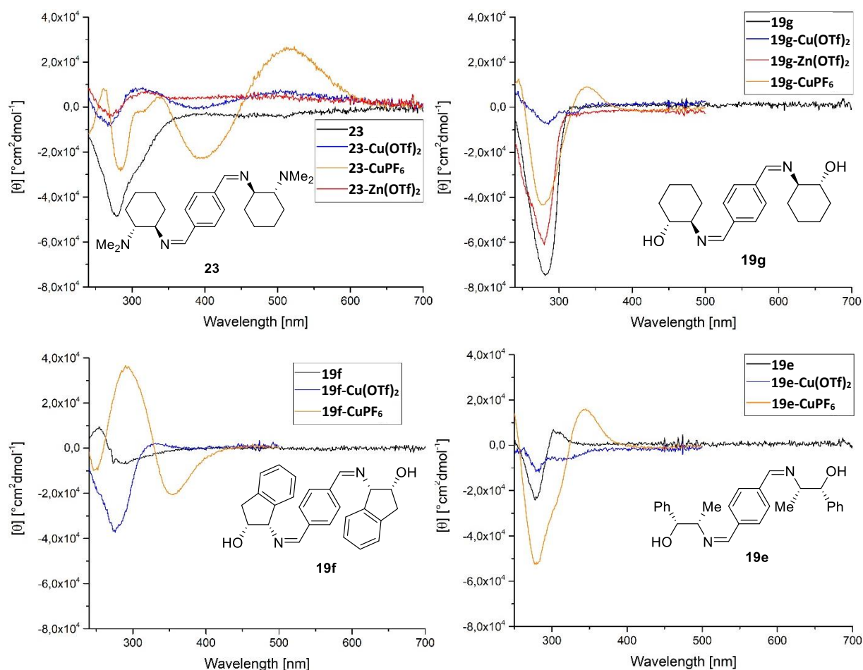
Figure 110: CD spectra of ligands a) 23 , b) 19g , c) 19f , d) 19e (black) and their respective \text{Cu}(\text{OTf})_2 (blue), \text{Zn}(\text{OTf})_2 (red) and \text{CuPF}_6 -complexes (orange). All spectra were made in THF, 3\text{--}6 \cdot 10^{-5} M, except 19f and 23-CuPF 6 (DCM), 23 , 19e and 19e-Cu(OTf) 2 (MeOH).
