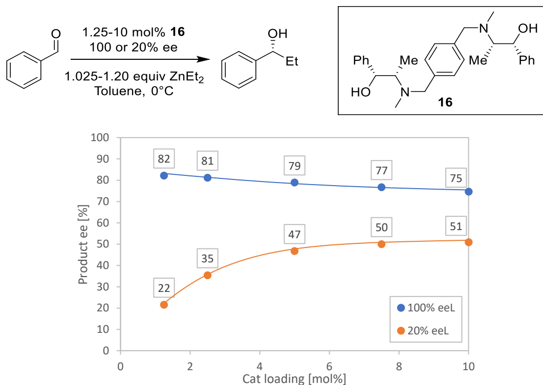
Figure 87: Catalyst loading screening in the 16 -catalysed addition of ZnEt_2 to benzaldehyde with enantiopure (blue dots) or 20% ee ligand.
