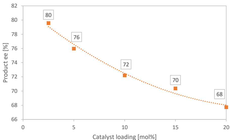
Figure 58: Catalyst loading screening in the (-)-NME-catalysed addition of \text{ZnEt}_2 to benzaldehyde.
