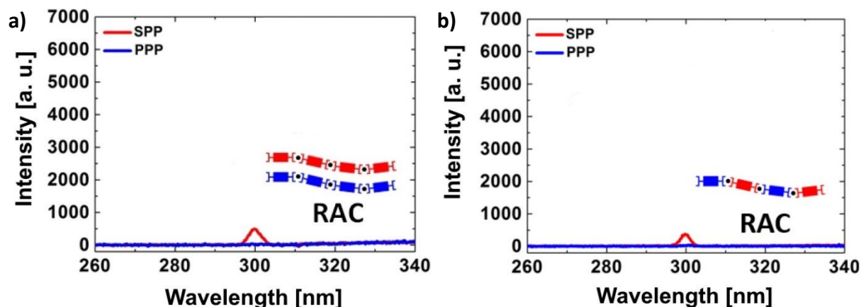
Figure 101: SFG spectra of a) racemic 18 -Cu(BF 4 ) 2 and b) racemic 18 -Zn(BF 4 ) 2 .
