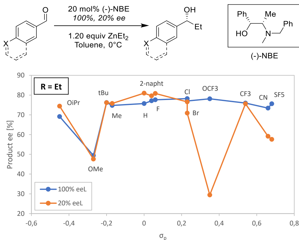
Figure 59: Screening of para -substituted benzaldehydes in the (-)-NBE-catalysed addition of ZnEt 2 . Each substrate was used in a reaction with enantiopure (blue dots) and 20% ee_L ligand (orange dots).
