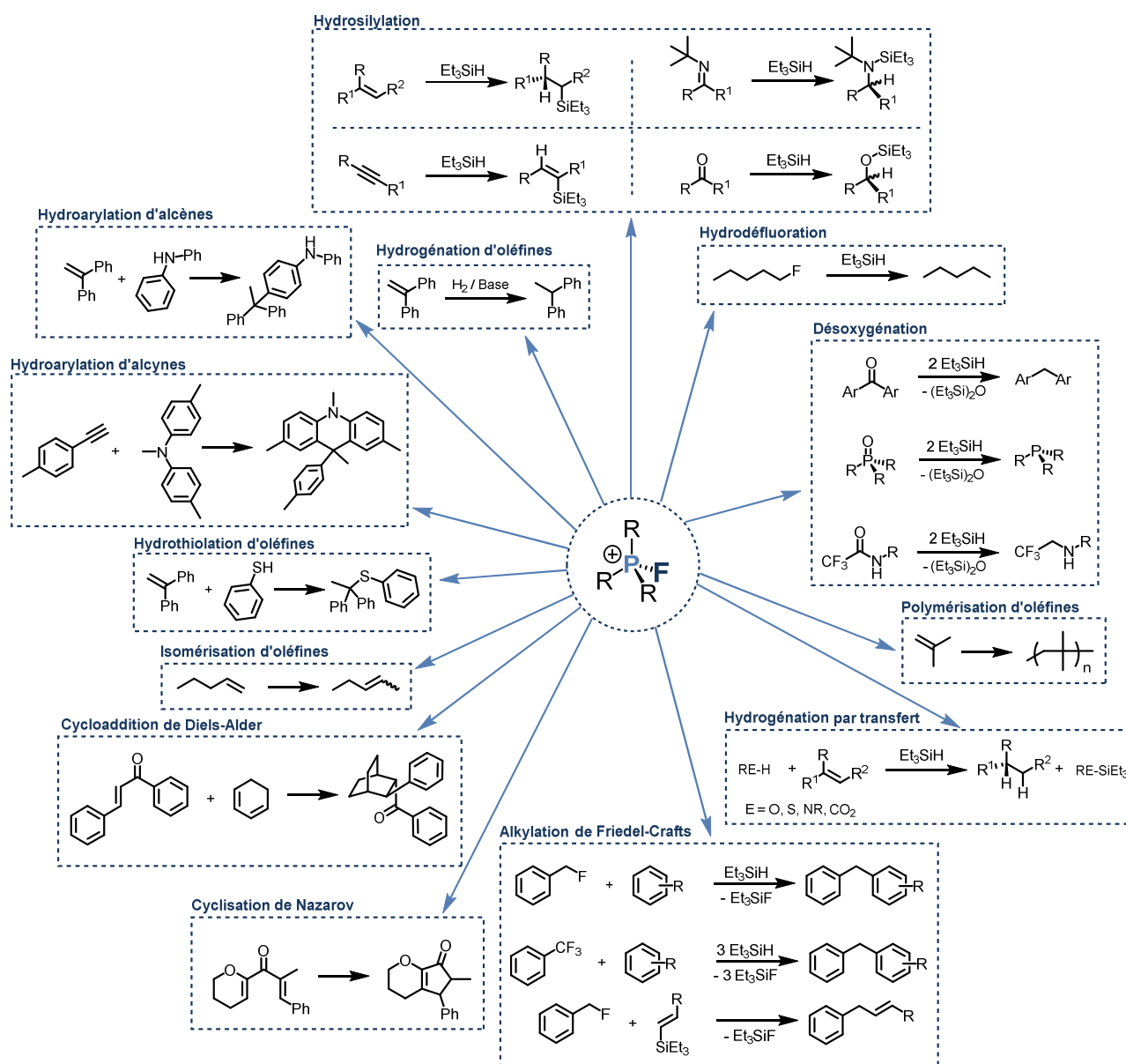
Figure 13 Applications catalytiques possibles des cations fluorophosphonium
