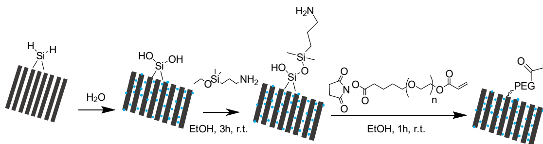
Scheme 5.2: Schematic representation of the surface modification of pSi particles.
