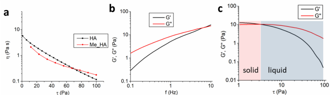
Figure 3.8: a) Shear thinning behavior of pristine HA (black) and Me_HA (red), 1700 kDa, 1% weight solutions in PBS. Plate to plate geometry (35 mm), T=25 °C; b) frequency sweep of Me_HA, elastic modulus (black) and loss modulus (red). Plate to plate geometry (35 mm), T=37 °C, \tau = 10 Pa; c) Stress-sweep of Me_HA, elastic modulus (black) and loss modulus (red). Plate to plate geometry (35 mm), T= 37 °C, f= 1 Hz.
