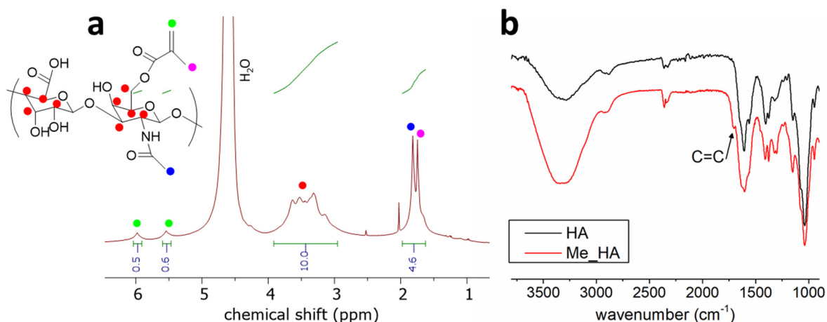
Figure 3.7: a) 1 H-NMR of methacrylated hyaluronic acid, 1700 kDa; b) FTIR-ATR of hyaluronic acid (black) and methacrylated hyaluronic acid (red).
