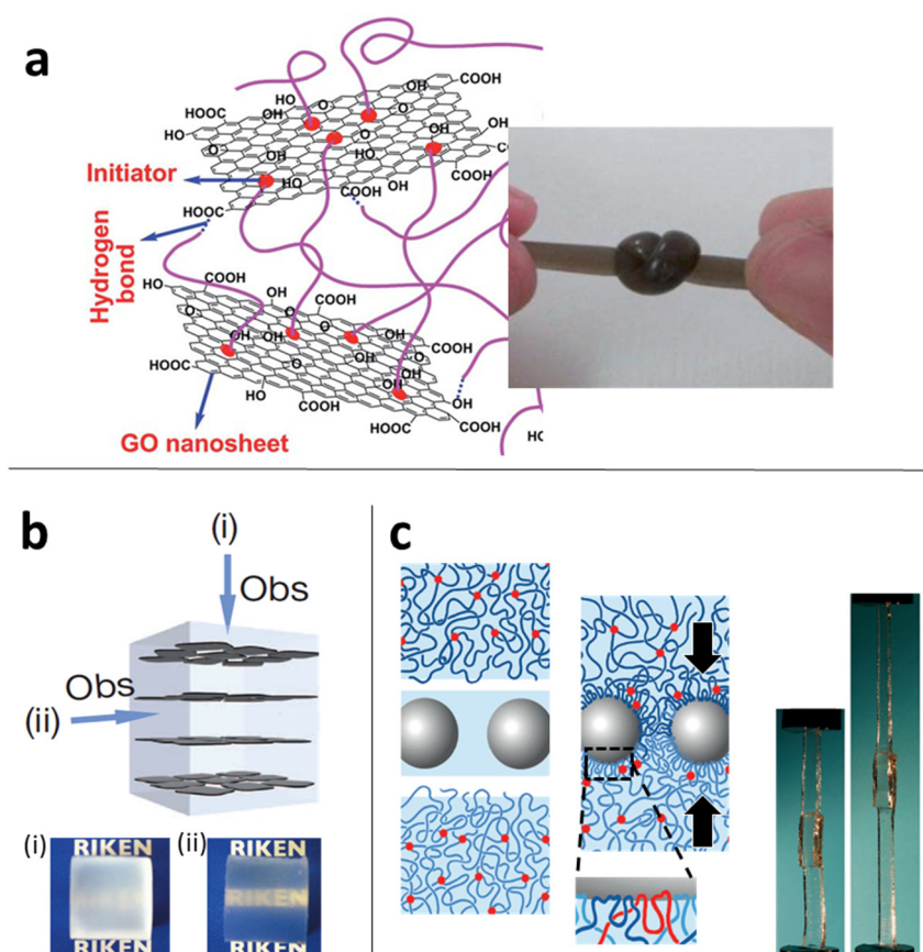
Figure 1.13: Emerging properties from the incorporation of nanofillers in hydrogels. a) The non-covalent interactions between the polymeric chain and the GO impart stretchability to the material. Adapted with permission from J. Mater. Chem. 2012 22, 14160. Copyright 2012, The Royal Society of Chemistry b) Co-facially oriented Ti nanosheets in a hydrogel prepared in presence of a 10 T magnetic field. Optical features of the material viewed along the orthogonal (i) and parallel (ii) direction to the aligned Ti nanosheets. Adapted with permission from Nature , 2015 , 517, 68. Copyright 2014, Springer Nature. c) Hydrogel adhesiveness given by the adsorption of polymeric chains on nanoparticles. Glued hydrogels can sustain large deformation. Adapted with permission from Nature 2014 , 505, 382. Copyright 2013, Springer Nature.
