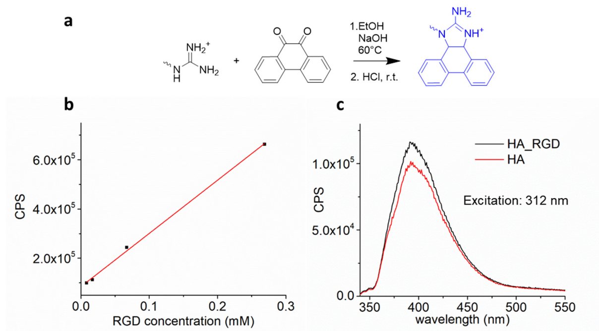
Figure 4.4: a) Reaction between the arginine lateral chain of the RGD peptide and the phenantroquinone to give the luminescent product. b) Calibration curve of the emission intensity at 392 nm of HA solutions containing different amount of RGD after reaction with the phenantroquinone. c) Emission spectra of the RGD functionalized HA (black) and bear HA (red) after reaction with the phenantroquinone. The spectra are recorded at room temperature, in water with excitation at 312 nm.
