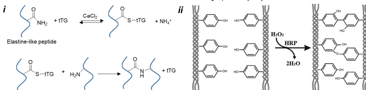
Figure 1.9: a) Use of photopolymerization for the preparation of a micropatterned hydrogel by photo-lithography.; The application of a photomask while irradiating the polymer mixed with the photoinitiator allows to impart the desired pattern to the final material. Adapted with permission from Nat. Biomed Eng. 2019 , 3, 58. Copyright 2019, Springer Nature. b) Enzyme mediated cross-linking. i) Elastine-like cross-linking mediated by transglutaminase (tTG) in presence of calcium ions. ii) Collagen functionalized with phenolic-hydroxyl groups and cross-linked by horseradish peroxidase (HRP) in presence of \text{H}_2\text{O}_2 . Adapted with permission from Acta Biomater. 2015 , 27, 151. Copyright 2015, Elsevier Ltd.
