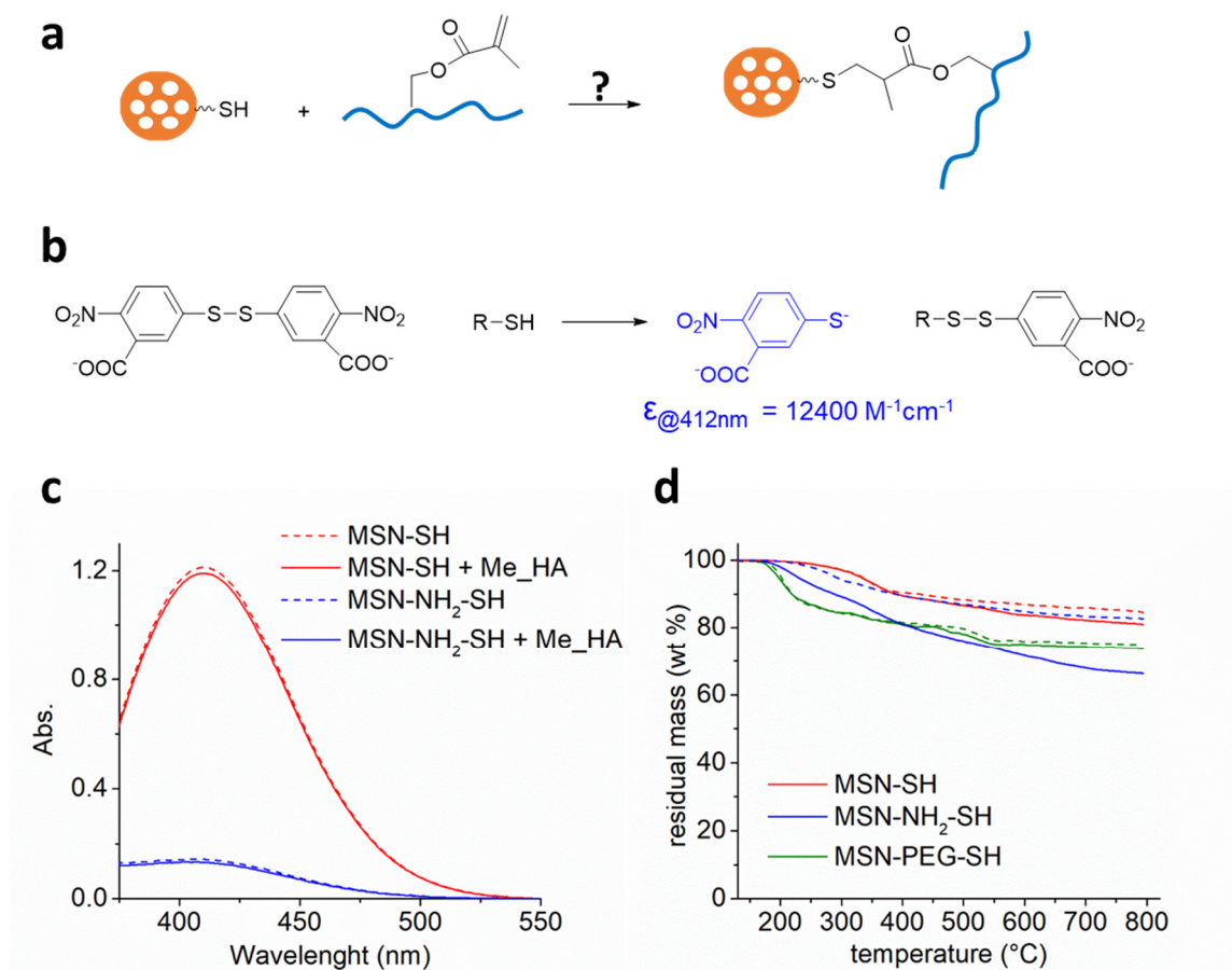
Figure 3.21: Evaluation of the formation of covalent bonds between the thiol functionalized MSN and the Me_HA. a) Scheme of the thiol-Michael reaction. b) Ellman's test for the quantification of thiols. c) Absorption spectra, after reaction with the Ellman's reagent, of MSN-SH (red) and MSN-NH 2 -SH (blue) water suspension before (dashed line) and after (solid line) incubation with Me_HA. d) TGA of the MSN-SH (red), the MSN-NH 2 -SH (blue) and MSN-PEG-SH (green) before (dashed line) and after (solid line) incubation with Me_HA.
