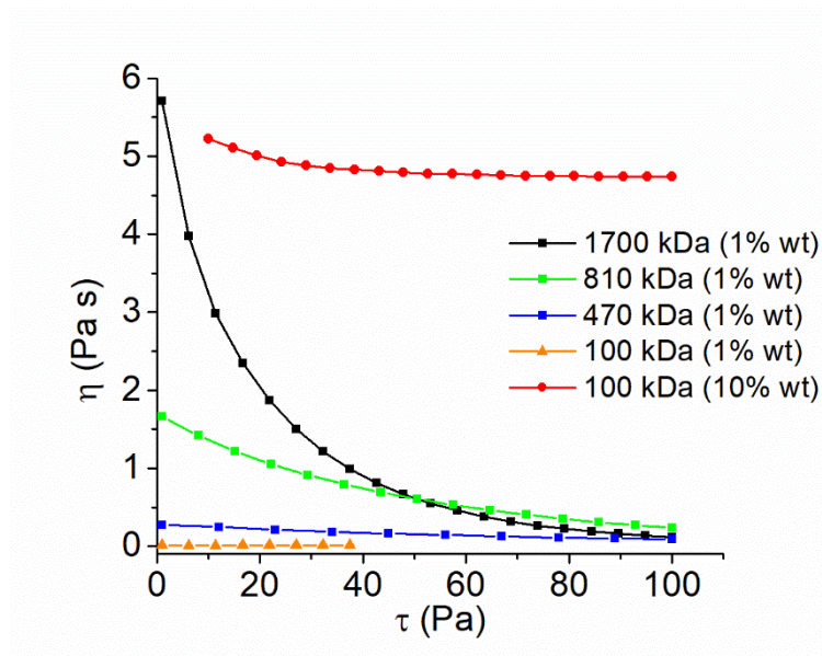
Figure 3.5: Viscosity as a function of the shear stress applied to HA solutions with different MW: 1700 kDa (black), 810 kDa (green), 470 kDa (blue), 100 kDa (orange) and 100 kDa, 10% (red). Rotational measurement done with coaxial cylinder geometry (25 mm) , T= 25\text{ }^{\circ}\text{C} .
