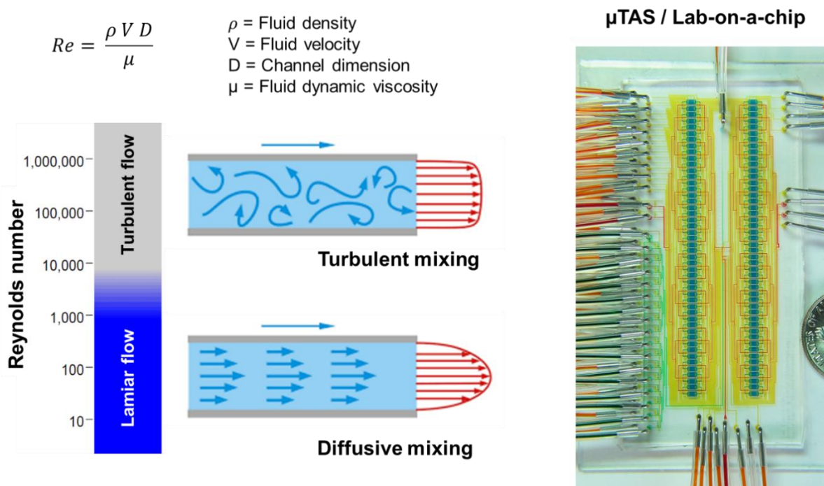
Figure 1.1 Concepts in microfluidics. (Left) Reynolds number (Re) describes the ratio of inertial forces to viscous forces in a fluid flow. At high Reynolds numbers ( Re > 3500 ) turbulent mixing occurs characterized by irregular movements of fluid particles. At low Reynolds numbers ( Re < 2000 ) fluid flows are laminar, flow particles move in straight lines. As a result, mixing occurs only by diffusion. Laminar flows have a parabolic flow velocity profile with a maximum in the centre of the pipe. (Right) A microfluidic chip and its interconnections. Adapted from Gomez-Sjöberg et al. 5 with permission from American Chemical Society.
