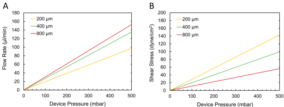
Figure 4.6. (a) Flow-pressure correlation in FlexDym™-PC devices from tests measuring the flow rate in a straight microfluidic channel (of width 200, 400 or 800 μm) and corresponding pressure at the channel inlet. Within 500 mBar of pressure applied at the device, flow rates of up to approximately 150 μL/min can be reached. (b) wall shear stresses that can be achieved in each of the example devices, as calculated from the flow rate data in (a), depending on the pressure applied. Shear stresses of up to approximately 140 dyne/cm 2 can be generated with pressures of 500 mBar and below. Reproduced from ref.* (see page 1) with permission from MDPI.
