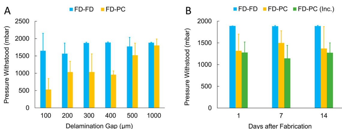
Figure 4.4. Pressure delamination testing. (a) FlexDym™-polycarbonate (FD-PC) and FlexDym™- FlexDym™ (FD-FD) bonding evaluation through pressure delamination testing of devices with gap distances from 100 to 1000 μm. FD-PC devices show reduced bonding strength compared to FD-FD bonding, but reliably withstand pressures of 500 mbar at gap distances of 200 μm and above. (b) Pressure delamination testing of FD-FD and FD-PC devices (fixed 400 μm gap distance) at 1, 7 and 14 days after fabrication. An additional set of FD-PC devices was aged in high humidity, 37 °C incubation conditions (Inc.), which revealed no significant impact on the device sealing due to time post-fabrication or incubation conditions (n=5 devices per dataset; error bars represent one standard deviation). Reproduced from ref.* (see page 1) with permission from MDPI.
