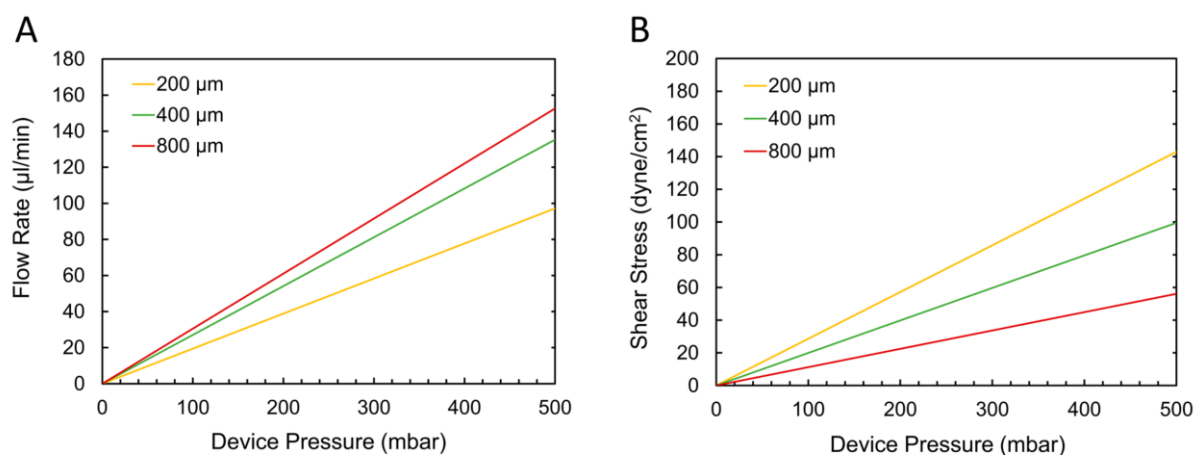
Figure 4.6. (a) Flow-pressure correlation in FlexDym TM -PC devices from tests measuring the flow rate in a straight microfluidic channel (of width 200, 400 or 800 \mu\text{m} ) and corresponding pressure at the channel inlet. Within 500 mBar of pressure applied at the device, flow rates of up to approximately 150 \mu\text{L}/\text{min} can be reached. (b) wall shear stresses that can be achieved in each of the example devices, as calculated from the flow rate data in (a), depending on the pressure applied. Shear stresses of up to approximately 140 \text{dyne}/\text{cm}^2 can be generated with pressures of 500 mBar and below. Reproduced from ref.* (see page 1) with permission from MDPI.
