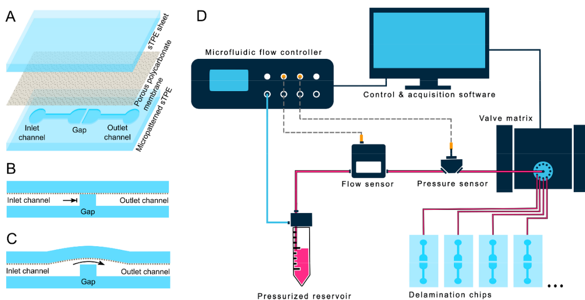
Figure 4.2. (a) Expanded view of the microfluidic chip design for delamination tests, consisting of two disconnected channels separated by a gap of varying distances. The inlet channel is increasingly pressurized, with no flow occurring until the delamination of test substrate from the FD gap structure occurs, at which point fluid crosses the gap into the outlet channel. (b) And (c) respectively show cross sections of the gap portion of the device before and after delamination. (d) Schematic of the automated delamination testing setup utilizing flow and pressure sensors and a valve matrix in series with a water-filled reservoir pressurized by a pressure controller. Continuous data logging and sensor feedback allowed the sequential testing of the pressure capacities of up to 10 microfluidic devices with no user monitoring. Reproduced from ref.* (see page 1) with permission from MDPI.
