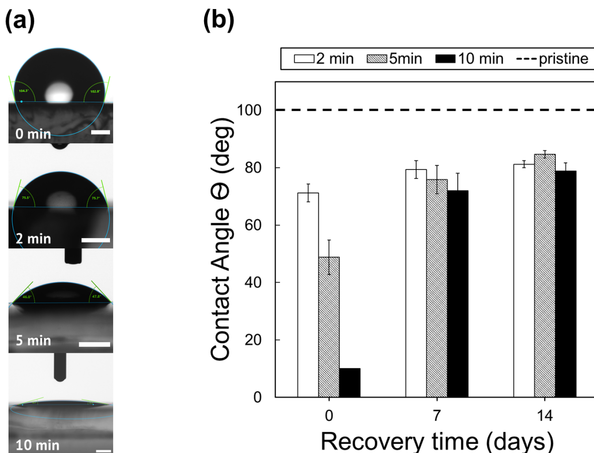
Figure 2.4. Static contact angle of DI water on FlexDym™ (a) and FlexDym™ treated with oxygen plasma (20 sccm, 50 mT and 100 W) for 2, 5 or 10 minutes. Scale bars 1 mm. (b) shows the evolution of the static contact angle of DI water on FlexDym™ surfaces treated with oxygen plasma for 2, 5 or 10 minutes. The dashed line represents the value of pristine FlexDym™ without plasma treatment. Average values of 5 measurements are shown and error bars represent one standard deviation.
