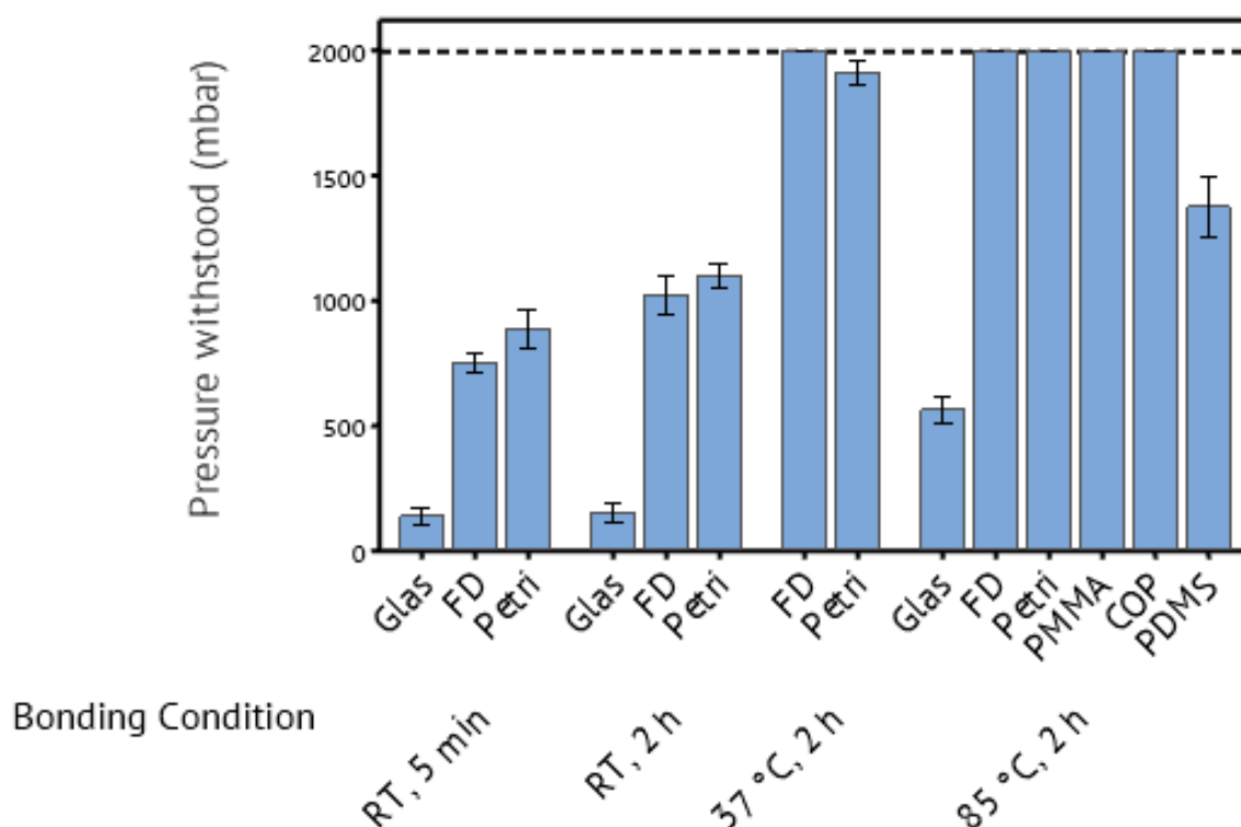
Figure 4.5. Evaluation of FlexDym™ bonding to glass, FlexDym™ (FD), petri dish, PMMA, COP and PDMS through pressure delamination testing of devices with gap distances 1000 \mu\text{m} . The dashed line represents the maximum test pressure (2000 mbar). The reported values are average values of 5 devices per dataset, and error bars represent the standard error.
