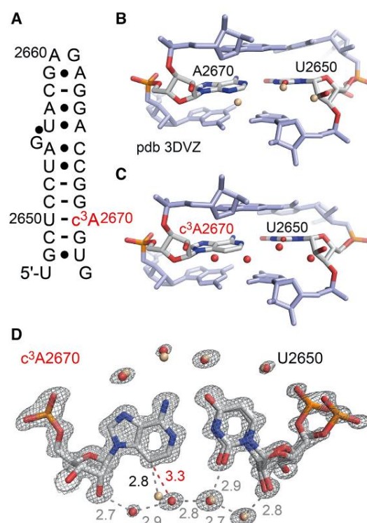
Figure 4. X-ray structure of 3-deazaadenosine modified RNA at atomic resolution. (A) Secondary structure of the E. coli Sarcin-ricin stem-loop (SRL) RNA used for crystallization. The c 3 A nucleotide is labeled in red. (B) Side view on the U2650/A2670 base pair in the unmodified duplex with ordered water molecules in the minor groove highlighted in beige color (PDB ID 3DVZ). (C) Side view on the U2650/c 3 A2670 base pair with ordered water molecules in the minor groove highlighted in red color (PDB ID 7L3R). (D) 2F o - F calc electron density map contoured at 1.5 σ level showing the U2650/c 3 A2670 base pair. Water molecules are shown as red spheres (PDB ID 7L3R) and are superposed to the water molecules observed in the unmodified RNA (PDB ID 3DVZ). Numbers are distances in Å. We note that the alternative conformations of U2650 (and C2649, G2648) are also observed in the unmodified SRL RNA scaffold (PDB ID 3DVZ).
