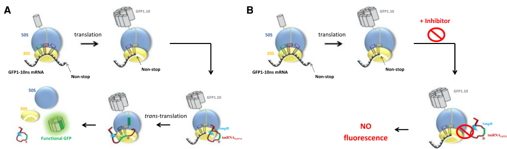
FIGURE 1. (A) Trans -translation of sfGFP1-10 mRNA lacking a stop codon. The tmRNA GFP11 -SmpB complex binds to the stalled ribosome, and translation resumes thanks to the tmRNA GFP11 mRNA-like domain (MLD). The MLD encodes the missing eleventh beta-strand of the sfGFP, and the complete sfGFP is released and becomes fluorescent. (B) Impairment of the process in the presence of trans -translation inhibitors. The ribosomes stay stalled on the problematic mRNA and fluorescence is impaired.
