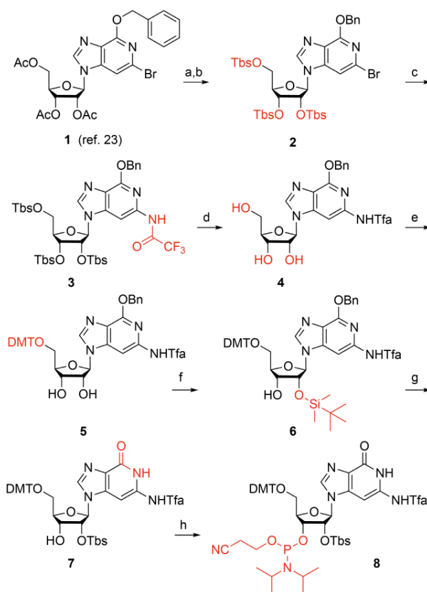
Scheme 1. Synthesis of the novel c^3G phosphoramidite building block 8 . Reagents and conditions: (a) MeNH_2 in ethanol, room temperature, 1 h, 99%; (b) 6 equiv tert -butyldimethylsilyl chloride (TbsCl), 7 equiv imidazole in DMF, room temperature, 72 h, 90%; (c) 1.2 equiv trifluoroacetamide, 1.4 equiv Cs_2CO_3 , 0.05 equiv Pd_2(dba)_3 , 0.15 equiv Xantphos in 1,4-dioxane, 110°C, 5 h, 90%; (d) 4.1 equiv tetra- n -butylammonium fluoride trihydrate in tetrahydrofuran, room temperature, 2 h, 87%; (e) 1.15 equiv 4,4'-dimethoxytriphenylmethyl chloride, 0.05 equiv 4-( N,N -dimethylamino)pyridine in pyridine, room temperature, 16 h, 74%; (f) 1.9 equiv TbsCl, 1.9 equiv AgNO_3 , in tetrahydrofuran, room temperature, 16 h, 39% (after two rounds of 2',3' equilibration); (g) 0.33 equiv Pd/C 10%, H_2 in tetrahydrofuran/ethanol 4:1, room temperature, 4 h, 79%; (h) 3.0 equiv 2-cyanoethyl- N,N,N',N' -tetraisopropylphosphorodiamidite, 0.5 equiv 5-(benzylthio)-1 H -tetrazole in dichloromethane, room temperature, 18 h, 79%.
