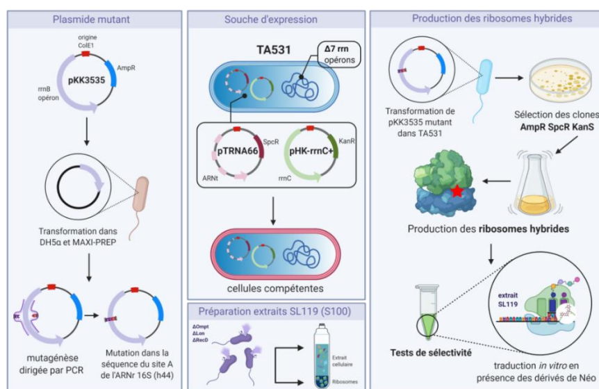
Figure 44 - Protocole de production de ribosomes hybrides
