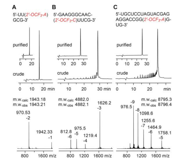
Fig. 1 Characterization of 2'- \text{OCF}_3 modified RNA. Anion-exchange HPLC traces (top) of 6 nt RNA (A), 15 nt RNA (B), and 27 nt RNA (C), and corresponding LC-ESI mass spectra (bottom). HPLC conditions: Dionex DNAPac column ( 4 \times 250 mm), 80^{\circ}\text{C} , 1\text{ mL min}^{-1} , 0–60% buffer B in 45 min; buffer A: Tris–HCl (25 mM), urea (6 M), pH 8.0; buffer B: Tris–HCl (25 mM), urea (6 M), \text{NaClO}_4 (0.5 M), pH 8.0. For LC-ESI MS conditions, see the ESI. ^{\dagger}
