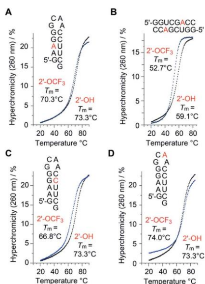
Fig. 2 Thermal stabilities of unmodified versus 2'-OCF 3 modified oligoribonucleotides. UV-melting profiles of hairpin and self-complementary duplex RNAs with the modification (either at adenosine or cytidine) located in the base-pairing region (A–C), and UV-melting profile of the same hairpin sequence with the modification in the GNRA loop motif (D). Conditions: c(RNA) = 12 μM; 10 mM Na 2 HPO 4 , 150 mM NaCl, pH 7.0. Nucleotides in red color indicate the positions for 2'-OCF 3 modification.
