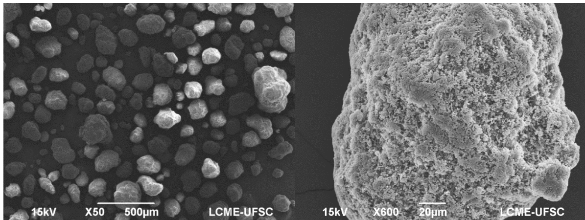
Figure 3: SEM images from Sample A. Various particles, scale bar: 500 µm (left) and individual particle, scale bar: 20 µm (right).
