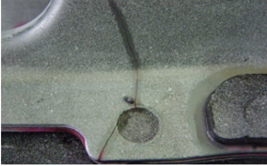
Figure 4.1: Example of critical zone on a cradle model under longitudinal sollicitations. The picture on the left represents the zone on the sixth specimen tested. The figure on the right represents the severity (multiplicative coefficient of the client objective F_n ) of the seven tests performed. Only two (the red ones) resulted into a crack initiation.
