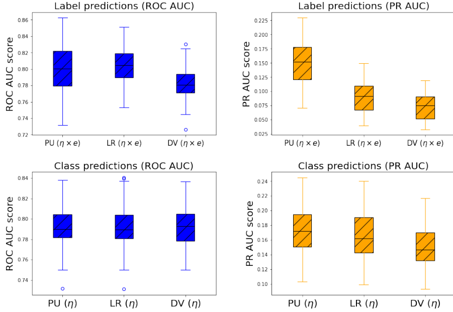
Figure 4.15: Quantitative performances of models with the simplified propensity (cf. Eq. 4.21): prediction performances on the labels (top, \eta \times e ) and on the classes (bottom, \eta ). The metrics used are ROC AUC (left) and PR AUC (right). Each boxplot represents the distribution of the prediction performances. Each series of three boxplots corresponds to (from left to right): PU-LR, non-traditional Logistic Regression and mechanical Dang Van criterion.
