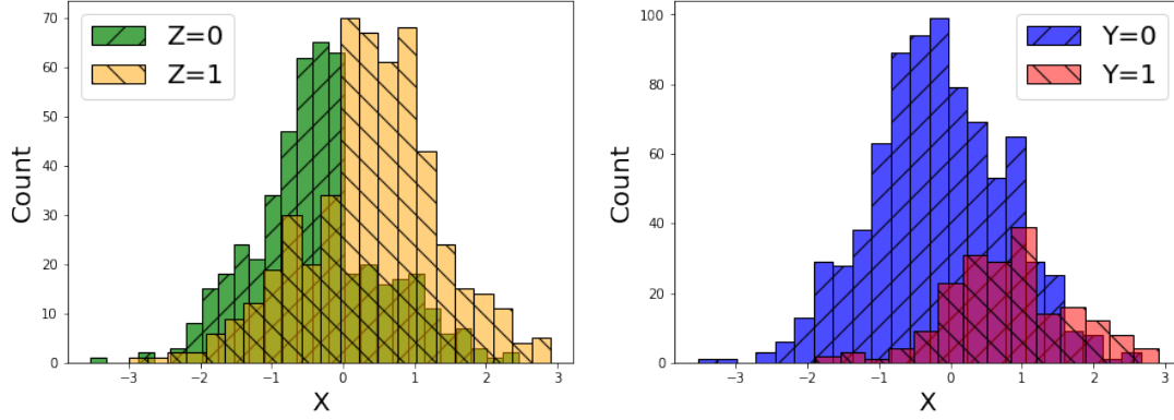
Figure 3.1: Example of simulation with n = 1000 , h = 0.5 and logistic propensity (with e_m = 0.05 ). On the left, the histograms of the positive and negative instances (true labels); on the right, the histograms of labeled and unlabeled instances (noisy labels). We can note a significant overlap between the distributions in both figures.
