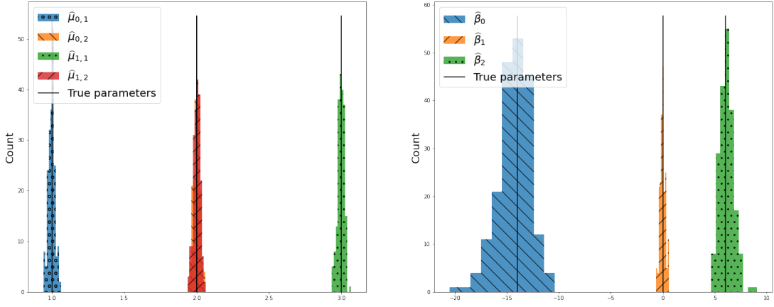
Figure 4.10: Empirical distribution of maximum likelihood estimate in PU-DA setting ( B = 200 experiments on data sets of size n = 1000 ): on the left, some of the parameters of the classifier \hat{\mu}_0 = (\hat{\mu}_{0,1}, \hat{\mu}_{0,2}) and \hat{\mu}_1 = (\hat{\mu}_{1,1}, \hat{\mu}_{1,2}) ; on the right, the parameters of the logistic propensity \hat{\phi} = (\hat{\beta}_0, \hat{\beta}) . The histograms on \hat{\mu}_{0,2} and \hat{\mu}_{1,2} are almost confounded, which is logical because the theoretical parameters are identical.
