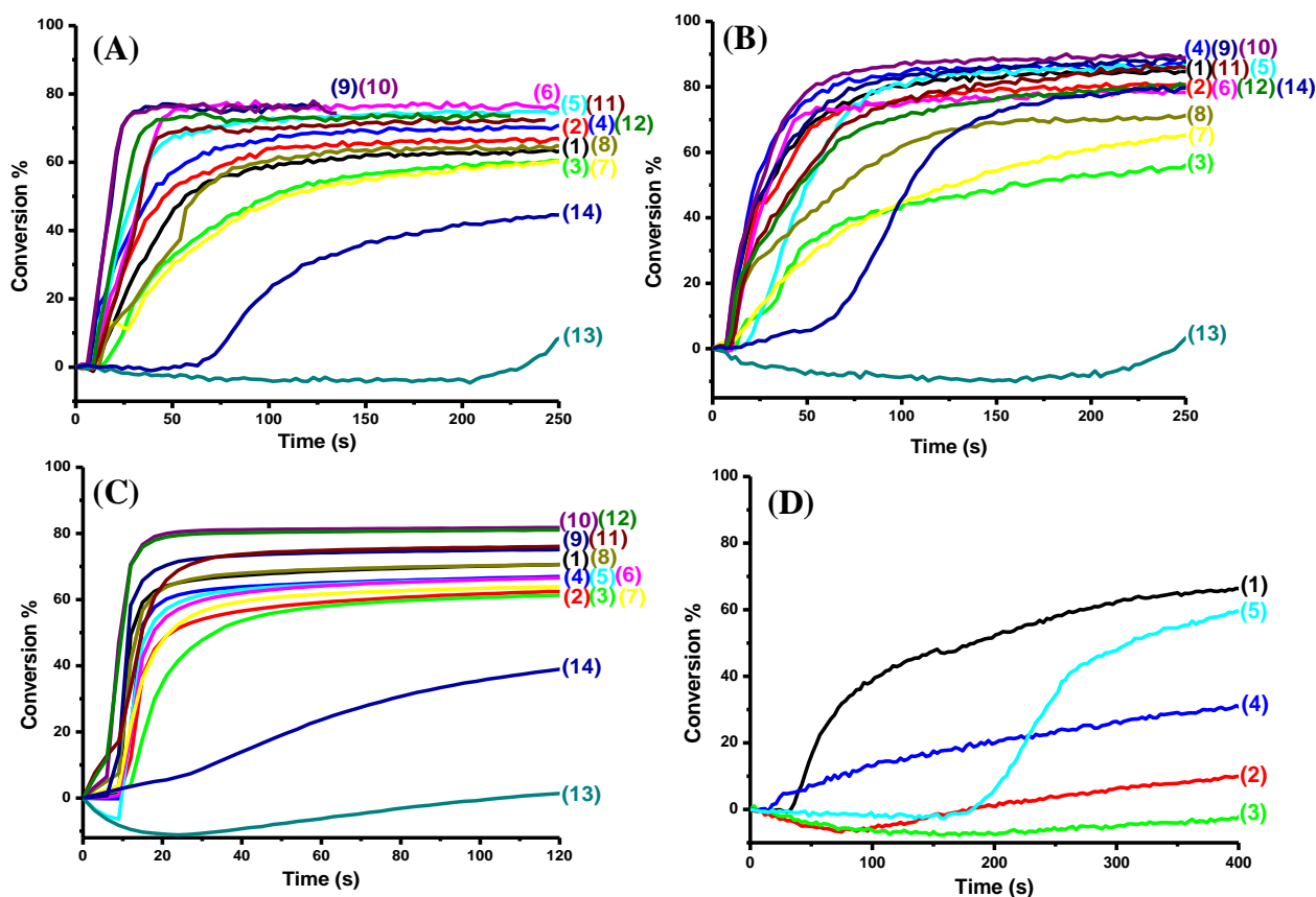
Figure 3. Polymerization profiles (Acrylate function conversion vs. irradiation time) for (A) TMPTA (thickness = 1.4 mm), (B) Ebecryl 40 (thickness = 1.4 mm), (C) Ebecryl 40 (thickness = 25 \mu m) upon exposure to the LED @405 nm in the presence of the two or three photoinitiating systems: (1) PT2/Iod (0.1%/1% w/w), (2) PT4/Iod (0.1%/1% w/w), (3) PT3/Iod (0.1%/1% w/w), (4) PT1/Iod (0.1%/1% w/w), (5) PT2/Iod/EDB (0.1%/1%/1% w/w/w), (6) PT4/Iod/EDB (0.1%/1%/1% w/w/w), (7) PT3/Iod/EDB (0.1%/1%/1% w/w/w), (8) PT1/Iod/EDB (0.1%/1%/1% w/w/w), (9) PT2/Iod/NPG (0.1%/1%/1% w/w/w), (10) PT4/Iod/NPG (0.1%/1%/1% w/w/w), (11) PT3/Iod/NPG (0.1%/1%/1% w/w/w), (12) PT1/Iod/NPG (0.1%/1% /1% w/w/w), (13) Iod/EDB (1%/1% w/w), (14) Iod/NPG (1%/1% w/w). Irradiation starts at t=10s. (D) Polymerization profiles (Acrylate function conversion vs. irradiation time) for a Ebecryl 40 resin (thickness =1.4 mm) upon exposure to the LED @405nm in the presence of the two-photoinitiating systems: (1) PT2/EDB (0.1%/1% w/w), (2) PT4/EDB (0.1%/1% w/w), (3) PT3/EDB (0.1%/1% w/w), (4) PT1/EDB (0.1%/1% w/w), (5) Benzophenone/EDB (0.1%/1% w/w).
