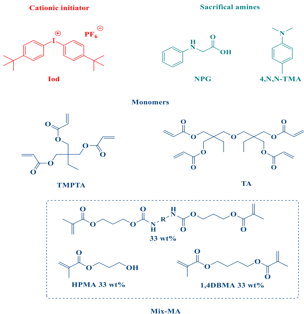
Figure 1. Other chemical compounds used in this paper.
