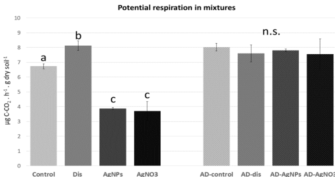
Figure 2: Potential carbon respiration of microbial communities in mixtures (µg C-CO 2 · h -1 · g -1 of dry soil). The letters indicate significant differences in respiration between the 4 treatments without sewage sludge. "n.s." indicates that there were no significant differences between the 4 treatments with sewage sludge.
