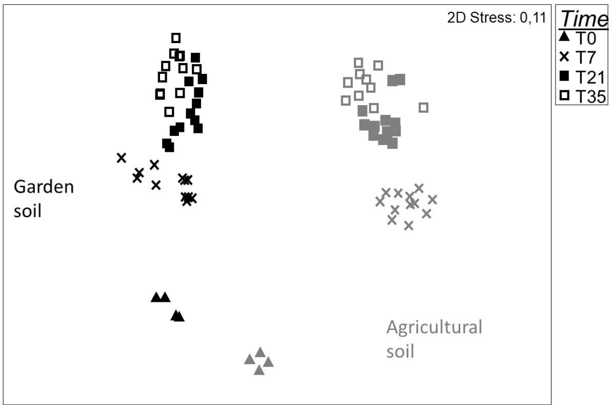
Figure 3: nMDS plot illustrating distances in BrayCurtis similarity index between diversity of the active microbial communities of all treatments (except for AD-dis) and all sampling dates. T0 (triangle), T7 (cross), T21 (full square) and T35 (hollow square) corresponds to the sampling time in days. The agricultural soil is represented by gray symbols and the garden soil is represented by black symbols.
