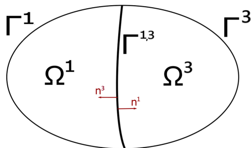
Figure 1.8: Example of spatial domain \Omega with an inner transverse membrane \Gamma^{1,3} which decomposes \Omega in open sets \Omega^1 and \Omega^3 . The figure also shows the outward normals to the membrane.
