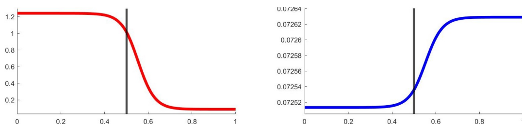
Figure 4.27: The jump between the right and left side solutions in Figure 4.22 is now filled and we can observe continuous solutions.
