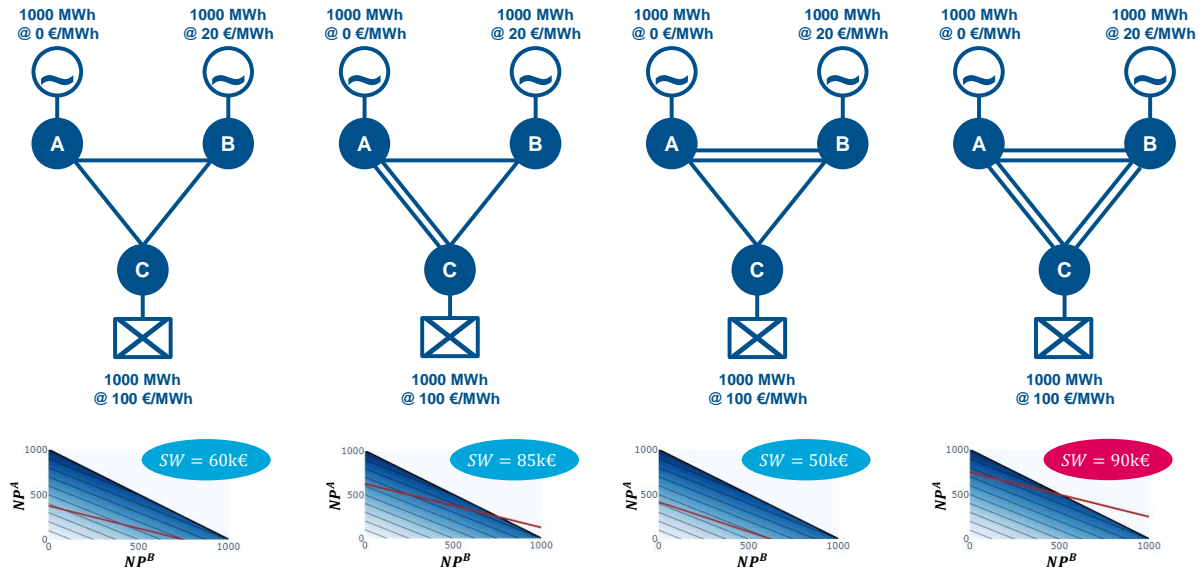
Figure 4.10: Four Topologies with Associated Market Welfare Values
