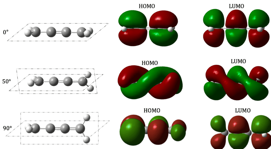
Figure 6.1: Representation of helical MOs of a [3]-cumulene at different states of rotation ( 0^\circ , 50^\circ , 90^\circ carried out by DFT computations) in the ground state
