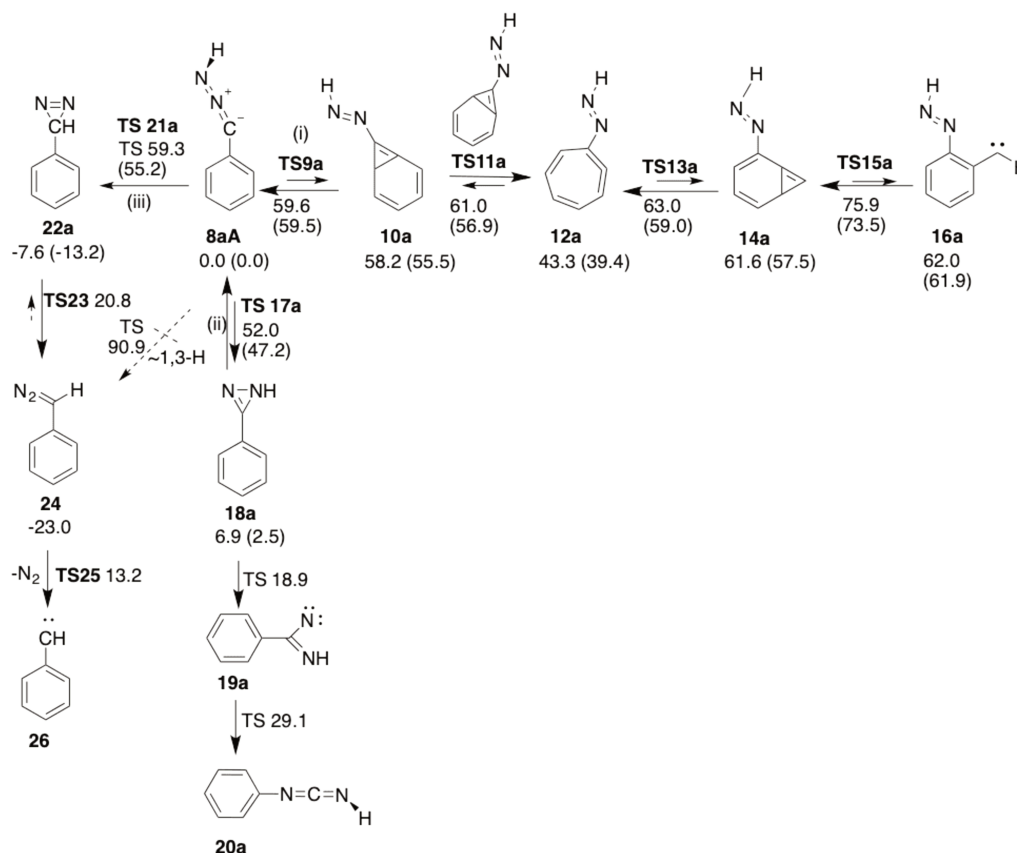
Figure 2.59: Rearrangment routes of aromatic nitrile imines [32]
