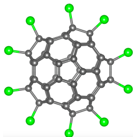
Figure 2.39: Representation of the fullerene molecule C_{50}Cl_{10}-D_{5h}
