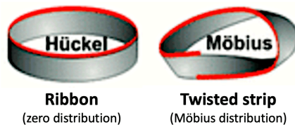
Figure 4.3: Illustration of the 2 distributions: Hückel and Möbius-types [49]
