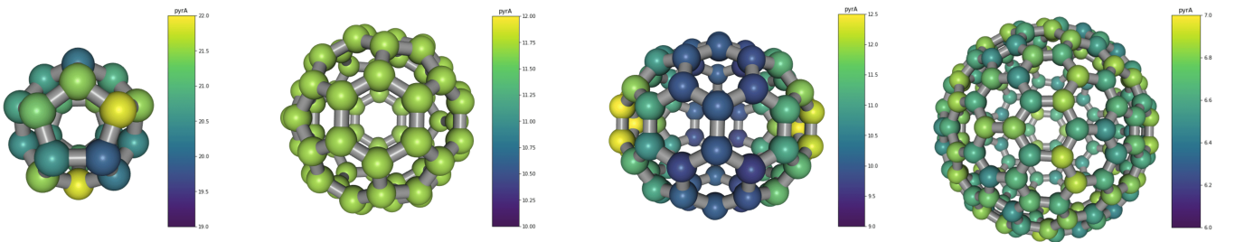
Figure 2.3: Cartographies of the pyramidalization angle for the fullerenes C_{20} , C_{60} , C_{70} , C_{180}
