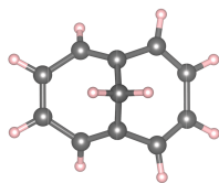
Figure 2.7: Representation of the molecule 1,6-methano-[10]-annulene ( C_{11}H_{10} )
