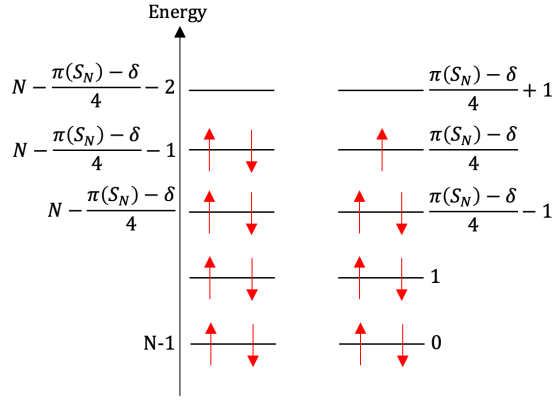
Figure 4.11: Distribution of the energy levels of S_N^1(\phi_M) in the case of \pi(S_N^1) \not\equiv 0 \pmod{4}
