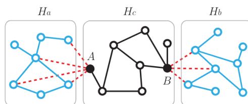
Figure 5.6: Schematic illustration of a molecule to define a Hamiltonian square matrix in the Löwdin partitioning technique [57] (the graph consists of two branch graphs a and b in cyan and a center graph c in black - the dashed edges in red represents the connections between them, with A and B being the branch-root nodes).
