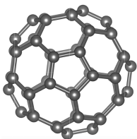
Figure 2.35: Representation of the molecule fullerene C_{50}-D_{5h}
