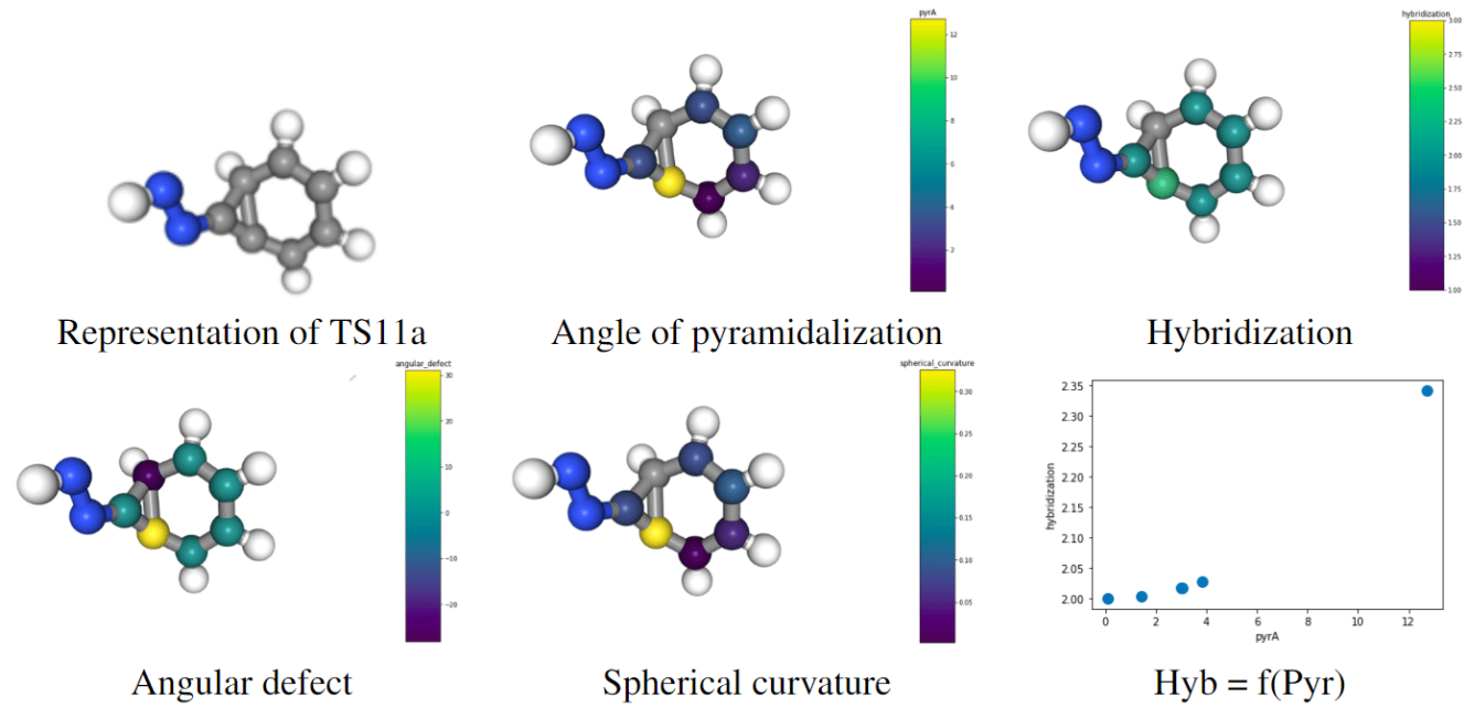
Figure 2.77: Cartographies and representation of the parameters of conformation TS11a
