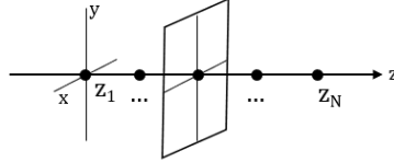
Figure 5.7: Schematic representation of a linear chain depending on the z axis
