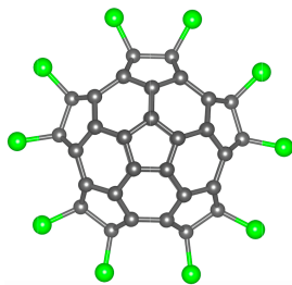
Figure 2.37: Representation of the fullerene molecule C_{50}Cl_{10}-D_3
