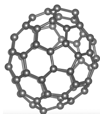
Figure 2.45: Representation of the molecule C_{64}-D_2
