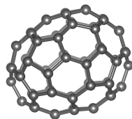
Figure 2.47: Representation of the molecule C_{64}-C_s
