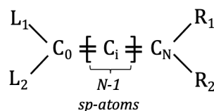
Figure 5.2: Representation of a [n]-cumulene
