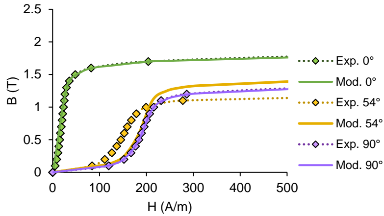
Figure I.30. Results of the elliptic model in terms of B-H curves for the three main directions.
