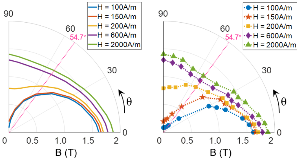
Figure I.36. Trace of the modules of \mathbf{B} as a function of the angle \theta at different magnetic field levels Results of the modified elliptic model (left) vs measured behavior of a CGO steel (right).
