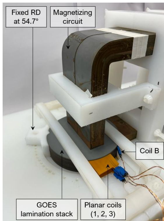
Figure III.19. Close look to the stacked sample positioning.
