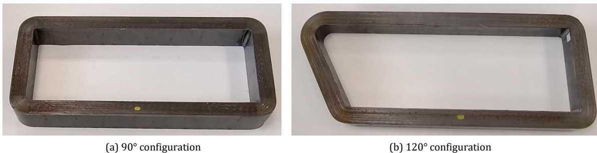
Figure III.12. Magnetizing circuits corresponding to the configurations 90 and 120° of the demonstrator.
