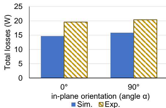
Figure IV.30. Computed total iron losses (non-linear isotropic magnetodynamic simulation) vs experimental losses in the GOES lamination stack for a magnetizing current I = 2.6 A r.m.s.
