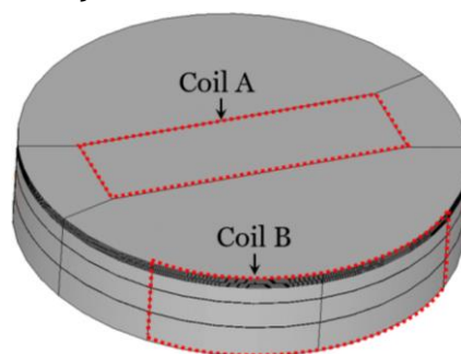
Figure IV.2. Closed surfaces for computing the magnetic flux.
