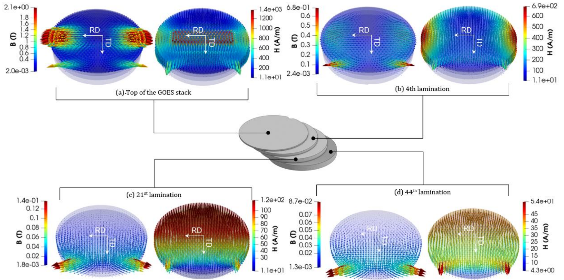
Figure IV.13. Magnetodynamic simulation of the evolution of the H (A/m) and B (T) field distributions within the GOES lamination for the 90^\circ in-plane orientation and a magnetizing current of I = 0.43 A r.m.s.
