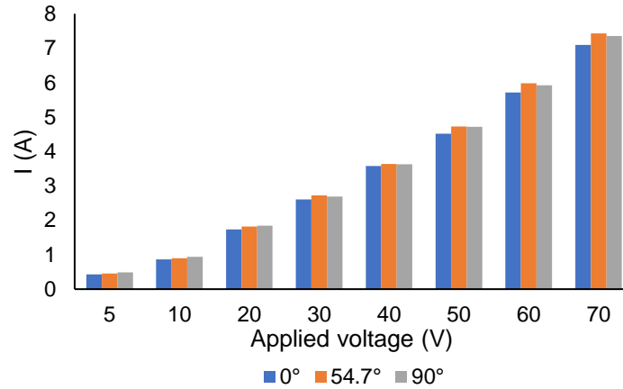
Figure III.30. Magnetizing current vs applied voltage for three in-plane orientations of the GOES stack under test: 0°, 90° and 54.7° (90° configuration of the demonstrator).
