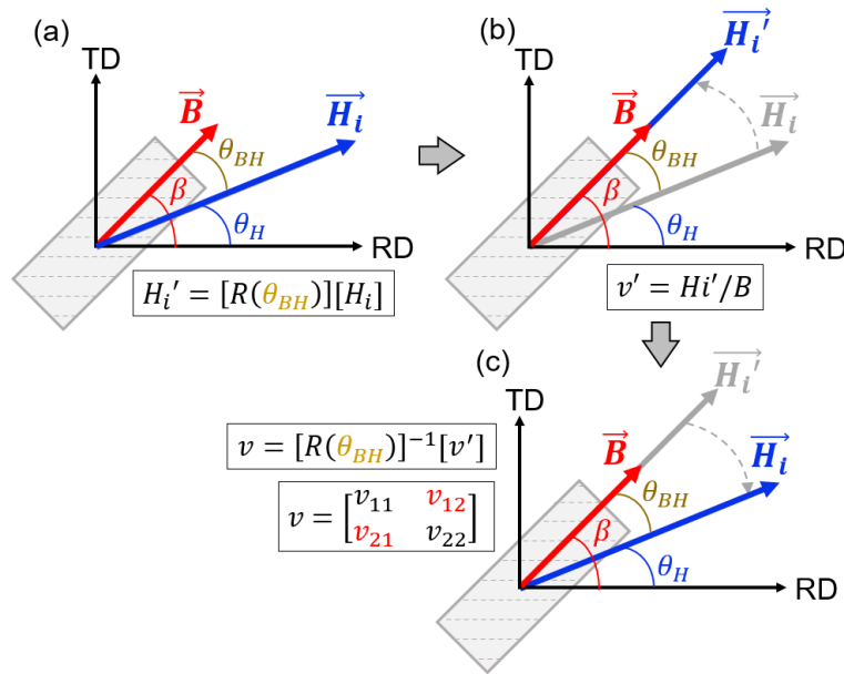
Figure I.39. Principle of the Enokizono model. (a) initial magnetization state, (b) rotation of the applied magnetic field H_i to the position of B , (c) calculation of the reluctivity tensor [v'] and inverse rotation into the original position.
