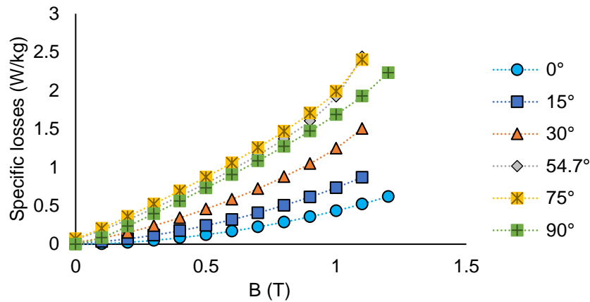
Figure I.26. Specific iron loss evolution as a function of B and \theta from GOES measurements.
