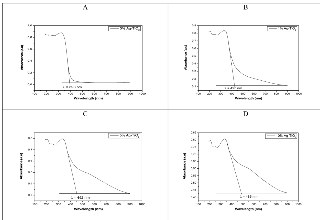
Fig. 6. UV-Vis absorption spectra of annealed \text{TiO}_2 and Ag-doped \text{TiO}_2 nanopowders.
