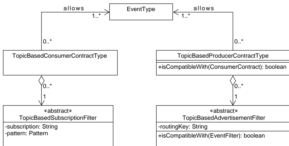
(b) Topic-based
