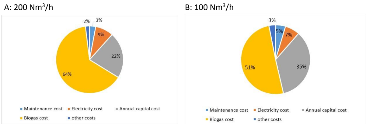
Figure 3-11: Share of cost items in the specific cost of biomethane production with water scrubbing at biogas flow rate A: 200 Nm 3 /h and B: 100 Nm 3 /h
