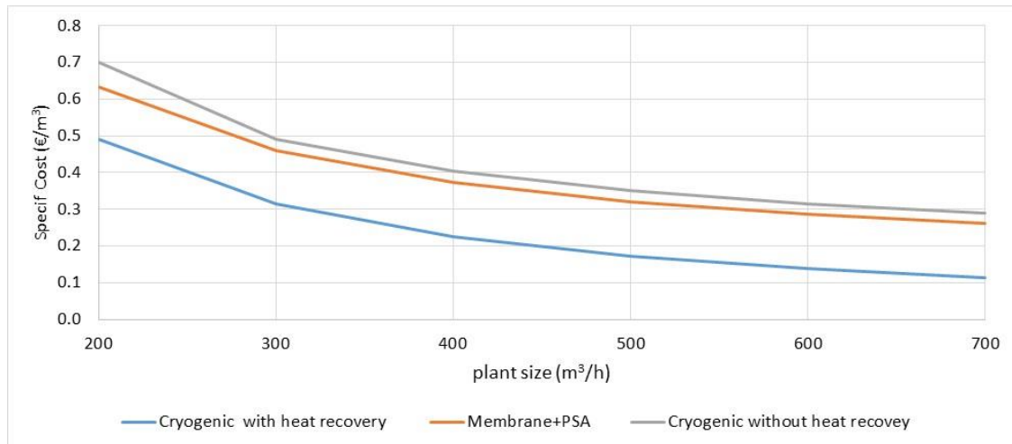
Figure 3-10: Specific cost of biomethane production as a function of plant size (Nm³/h)
