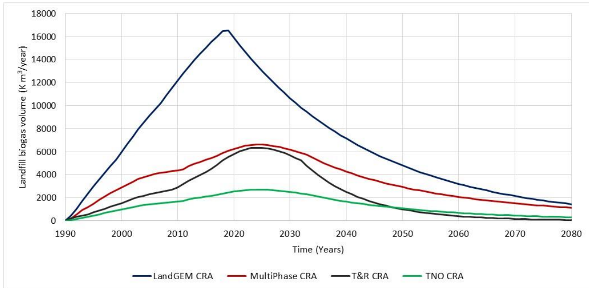
Figure 2-4: LFG generation obtained by CRA method with different models at L_0 = 115.7 and k = 0.04
