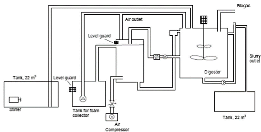
Figure 1-11: Process diagram of methane enrichment process adopted from [52],[9]
