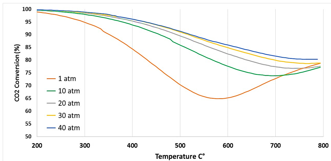
Figure 4-6: CO_2 Conversion with Different pressures versus Temperature-Present Simulation Results
