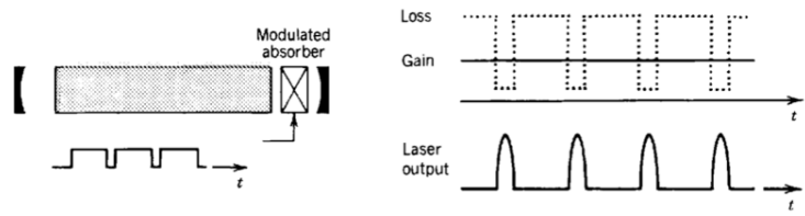
Figure 1.18: Schematic representations of Q switching with the time-dependence of the gain and losses inside the cavity and the associated laser output. Images taken from [10] .
