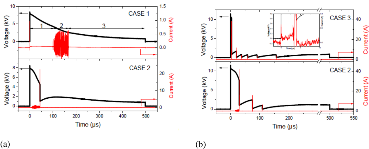
Figure 4.2 Voltage and current signals of a single pin-to-pin discharge in water ( \sigma=100\mu\text{S}/\text{cm} ) monitored for applied voltages of 500 \mu\text{s} (a) 9 kV and (b) 12 kV 175
