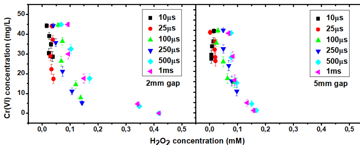
Figure 7.7 Cr(VI) concentration as a function of H 2 O 2 formation by pin-to-pin discharge in Cr(VI) solution (47 mg/L, \sigma = 4 mS/cm, pH = 2.4) for different pulse durations and gaps. U = 9 kV, V = 100 mL, electrodes length = 0 \pm 10 \mu m, f = 50 Hz - measurements performed at 15, 45, 90 and 120 minutes are reported
