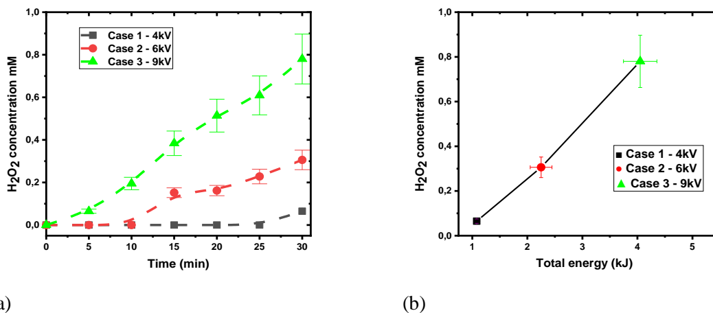
Figure 5.3 Hydrogen peroxide concentration for three different cases (applied voltages). (a) Concentration of H 2 O 2 as a function of time. (b) Final concentration of H 2 O 2 as a function of total injected energy (measured after 30 min) (V = 200 mL, f = 50 Hz, Δt = 500 μs, 2 mm of gap, σ = 200 μS/cm). Uncertainties of [H 2 O 2 ] and energy are 15 % and 10%, respectively
