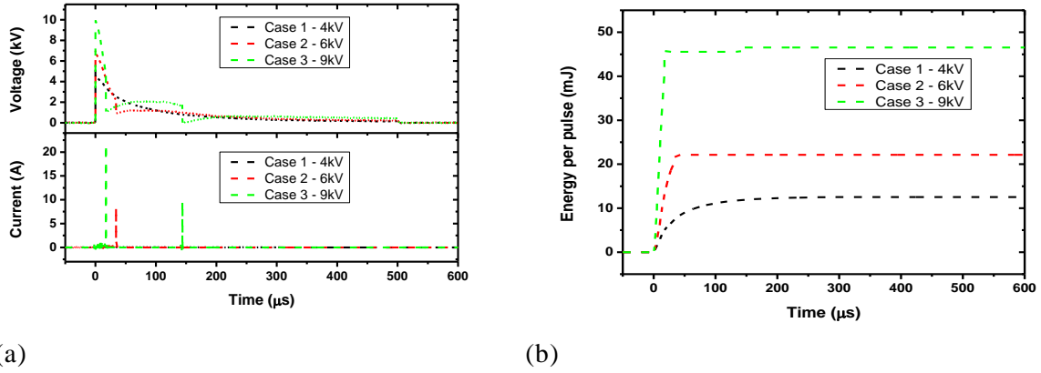
Figure 5.2 Typical electrical waveforms of pin-to-pin discharge generated in water V = 200 mL, f = 50 Hz, \Delta t = 500 \mu s, 2 mm of gap, and \sigma = 200 \mu S/cm); (a) Voltage and Current signals and (b) Time evolution of the energy per pulse 202
