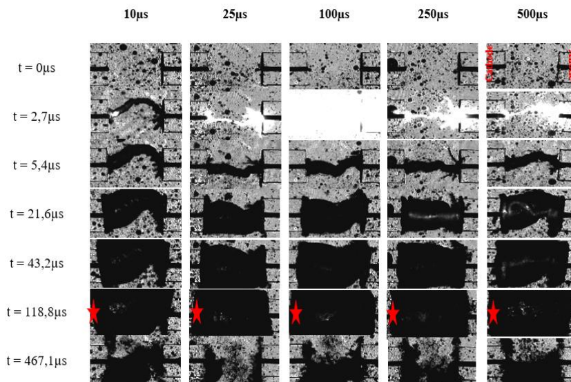
Figure 4.17 The time-resolved shadowgraphy measurements of a pin-to-pin discharge obtained in Cr(VI) solution ( 47 \text{ mg/L}, \sigma=4 \text{ mS/cm}, \text{pH}=2.4 ) for different pulse duration with U = 11 \text{ kV} , V = 100 \text{ mL} , \text{gap} = 2 \text{ mm} , electrodes length = 0 \pm 10 \text{ } \mu\text{m} , f = 50 \text{ Hz} . Red stars show the maximum radius
