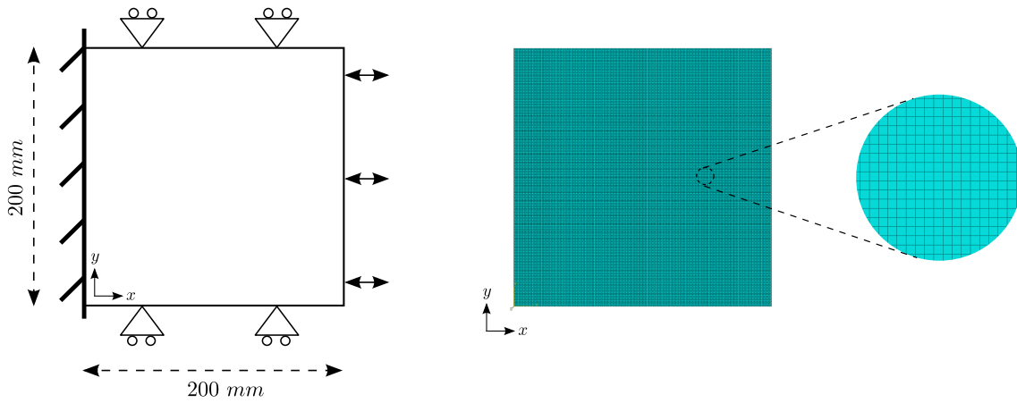
Figure 3.13: Illustration of dimension and boundary conditions (left) and mesh (right) of the 2D XFEM model in numerical examples.
