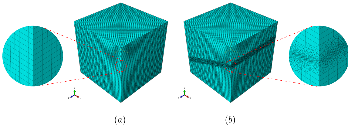
Figure 3.20: Illustration of mesh of the 3D model by XFEM (a) and by FEM (b).
