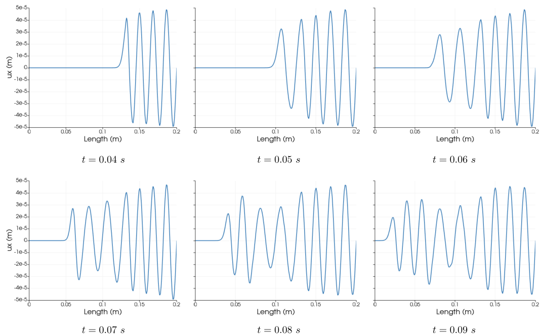
Figure 3.16: Displacements u_x along the horizontal median line of the circular inclusion model.
