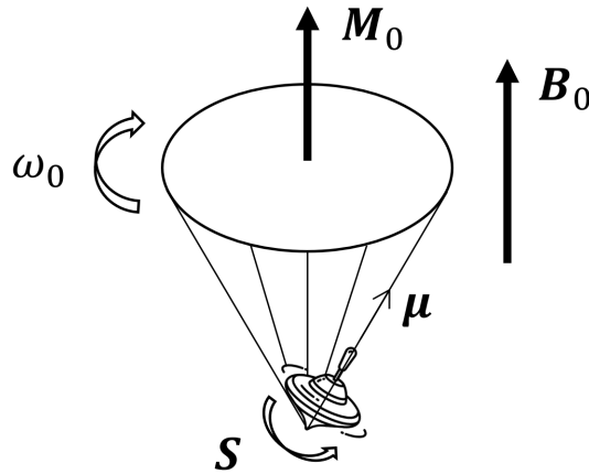
Figure 1.6: Larmor precession of proton. Proton spin is illustrated by a spinning-top. Magnetic moment \boldsymbol{\mu} is caused by spin \boldsymbol{S} . Precession of \boldsymbol{\mu} at Larmor frequency \omega_0 results from the existence of static magnetic field \boldsymbol{B}_0 . The population difference of two proton energy-states leads to a macroscopic magnetization \boldsymbol{M}_0 aligned with \boldsymbol{B}_0 .
