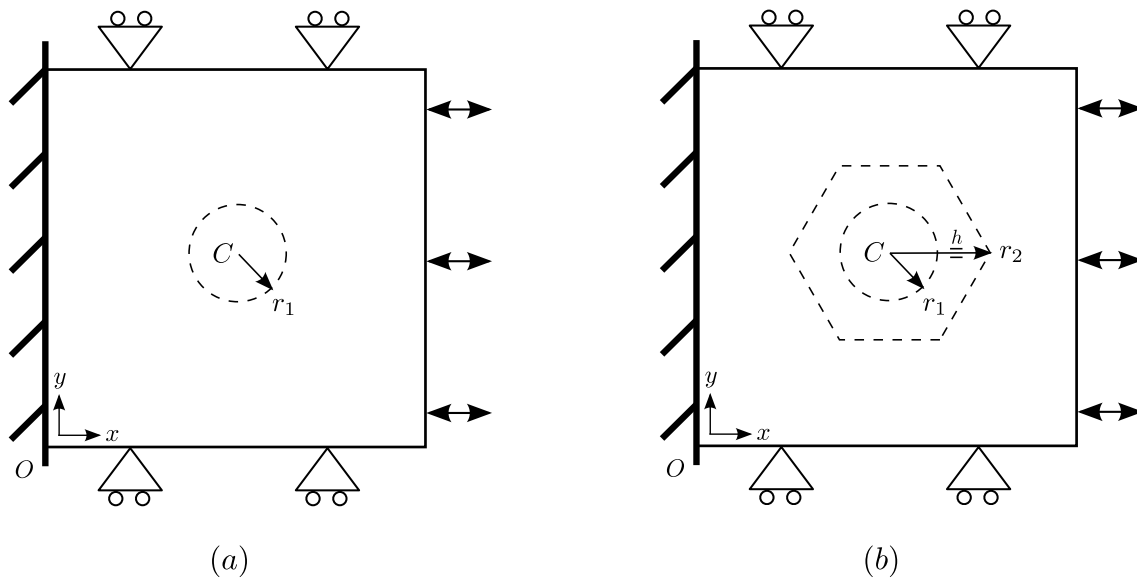
Figure 3.14: Illustration of the circular inclusion (a) and the nested inclusions (b).
