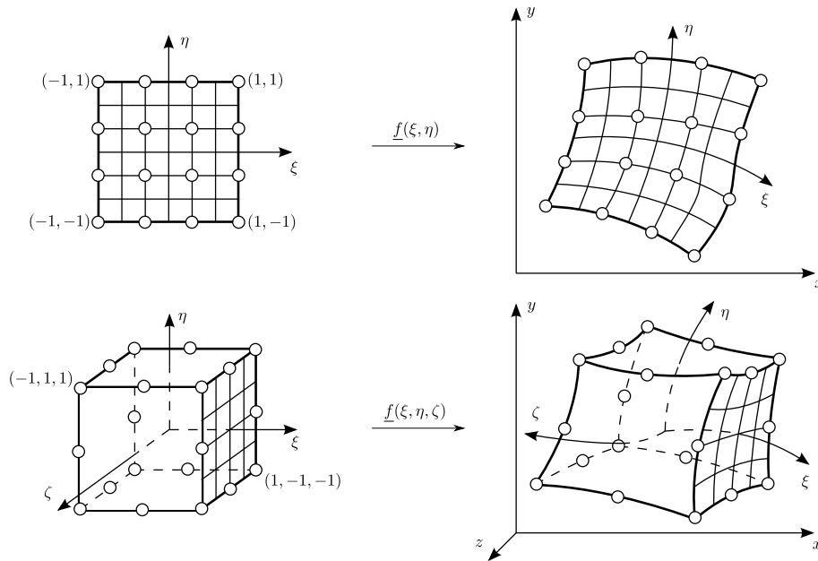
Figure 2.1: Mapping from local parametric coordinates into global Cartesian coordinates.
