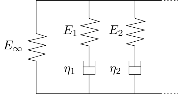
Figure 2.2: Generalized Maxwell-element
