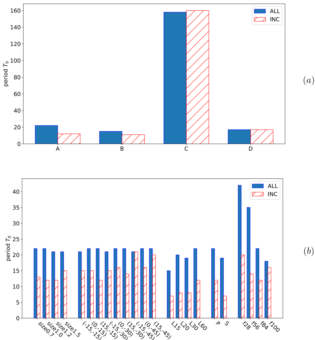
Figure 5.10: Results of the stability analysis of the four breast models (a), and the parametric study (b) presenting the influence of inclusion and driver on system stability.
