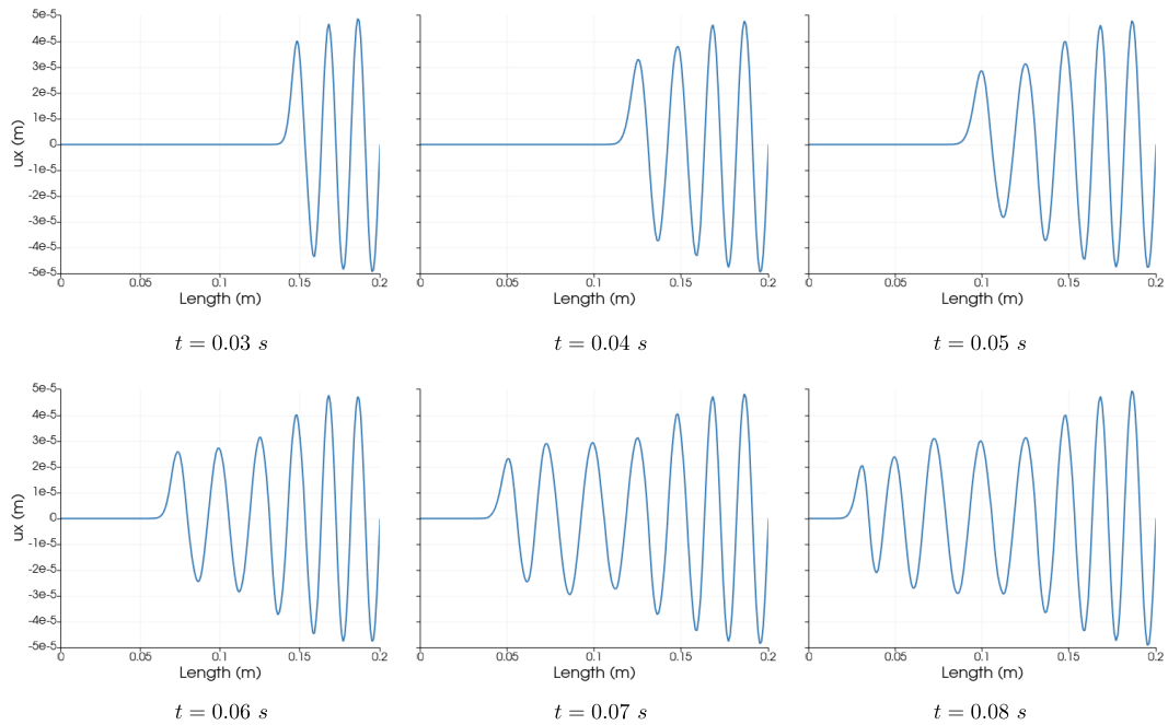
Figure 3.18: Displacements u_x along the horizontal median line of the nested inclusions model.
