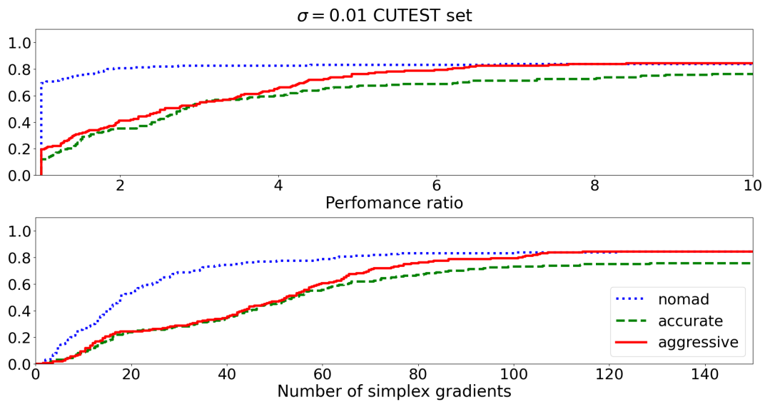
FIGURE 6.3: Performance and Data profiles on CUTESt instances, \sigma = 0.01
