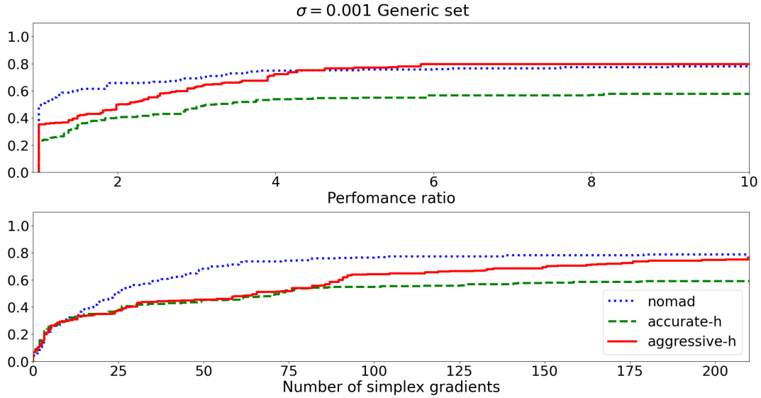
FIGURE 6.8: Performance and Data profiles on Generic instances in instances on heuristic versions of Algorithm 4.1, \sigma = 0.001
