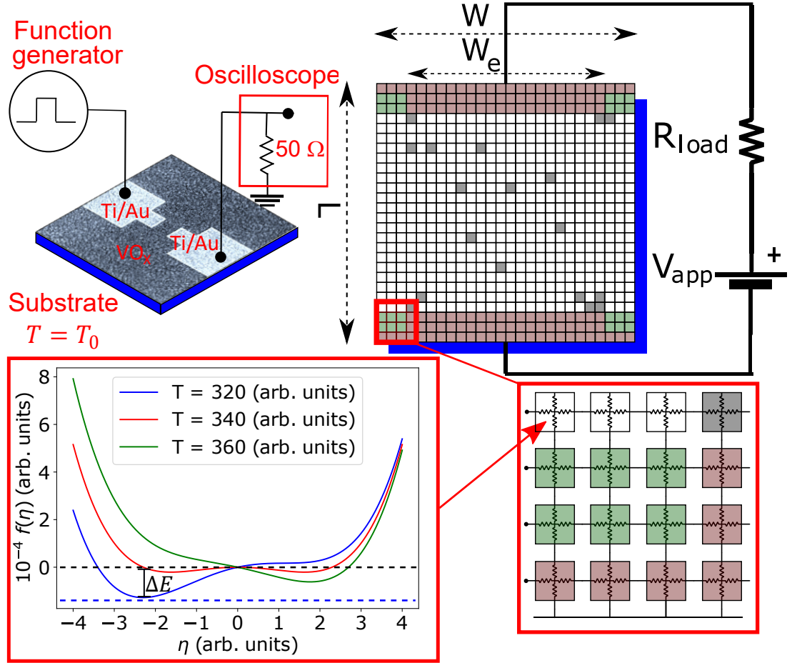
FIGURE 2.3 – Schematic diagram of the Mott Resistor Network model and the experimental setup [Val+19]. Cells in red are ideal metal with zero resistivity and represent the electrodes. Cells in white and grey represent the thin film Mott material, which is assumed in thermal contact with a perfectly insulating substrate that is at T_0 = 300 arb. units (in blue). These cells can be either in the insulating or metal states. Green cells are ideally insulating. Each cell is characterized by a Landau-type free energy that evolves with the temperature of the cell, as shown in the bottom inset figure. The two minima of the function correspond to the metal and insulating phase. The energy barrier \Delta E of the insulating phase at three different temperatures is shown.
