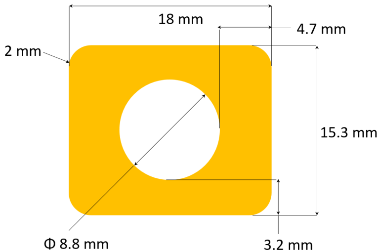
Figure 2.5: Aurubis M3HE0014 copper profile.
