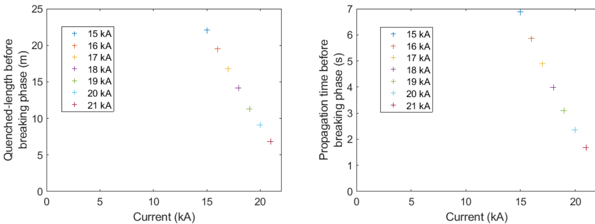
Figure 5.22: Quenched-length and propagation time before the breaking phase in function of the current, obtained with THEA ® .
