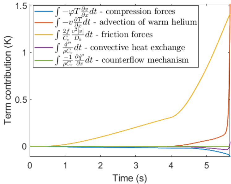
Figure 5.13: Time evolution of the integrals of the terms from the fluid temperature equation at X = 15 m.
