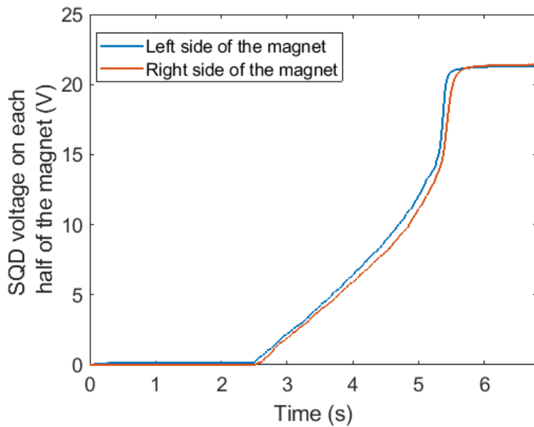
Figure 4.7: Comparison of the measured SQD voltage on each half of the magnet.
