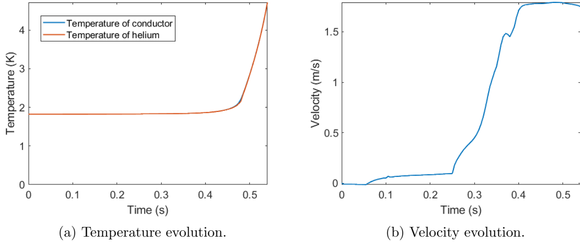
Figure 5.6: Time evolution of the temperature and velocity at X = 0.5 m. The temperature starts increasing at 0.4 s while the velocity, after a plateau until 0.25 s, increases strongly to a plateau around 1.8 m/s.
