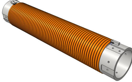
Figure 2.13: Scheme of the 58-turns MACQU solenoid wound on its supporting mandrel.
