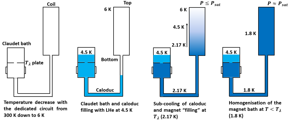
Figure B.2: Cooling down scheme of MACQU, inspired from SETH. The light blue is for liquid helium and dark blue is for superfluid helium.
