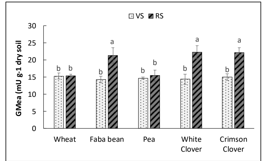
Figure 3. Patterns of the geometric means (GMea) of BG, NAG and ACP activities at the two development stages. BG: β-glucosidase; NAG: N-acetylglucosaminidase; ACP: acid phosphatase; VS: vegetative stage; RS: reproductive stage. GMea was calculated by using only the three enzyme activities that varied according to the plant's species. GMea = \sqrt[3]{(BG \times NAG \times ACP)} . Data are mean ± SD (n = 5). Letters indicate statistically significant difference between plants species and development stages at p < 0.05 according to Tukey's test.
