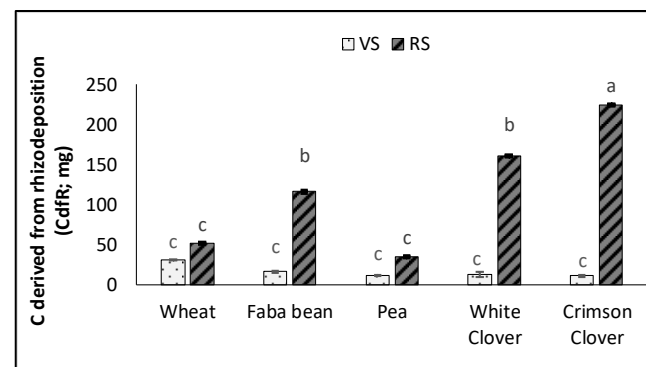
Figure 6. Soil C derived from rhizodeposition (CdFR) under all plants species at the two stages of development (mg.pot -1 ). VS: vegetative stage; RS: reproductive stage. Data are mean \pm SD ( n = 5 ). Letters indicate statistical significant difference between plants species at p < 0.05 according to Tukey's test.
