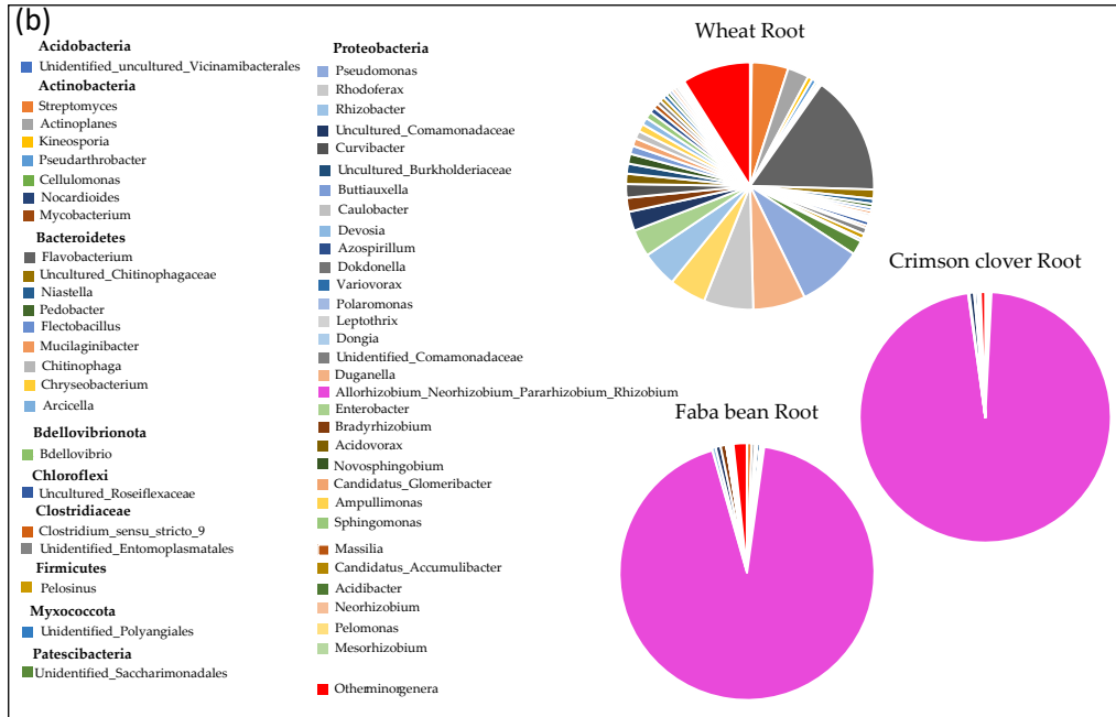
Figure 5. Relative abundance of root bacterial (a) phyla and (b) genera expressed as a percentage of total sequences obtained by Illumina sequencing for wheat, faba bean and crimson clover. Only genera showing significant differences among the roots of the three plant species are presented. Other minor genera correspond to sum of the genera with relative abundances < 0.2%.
