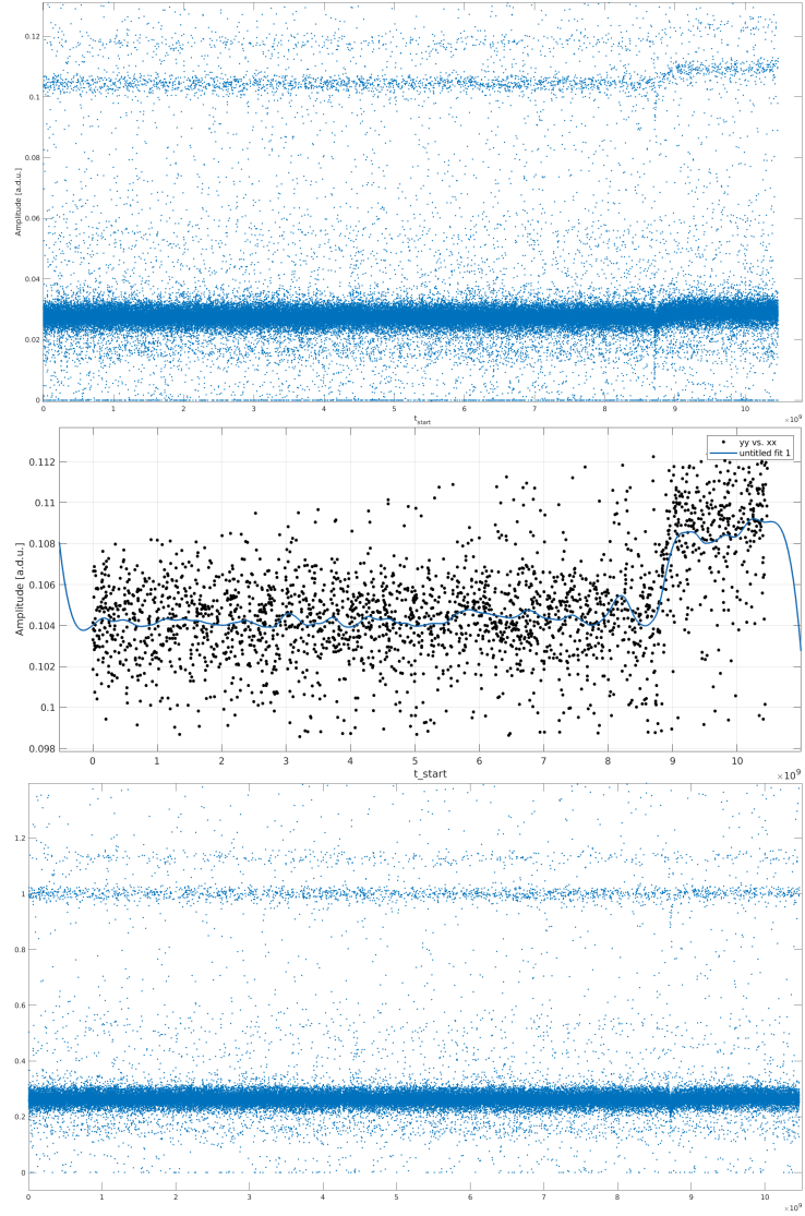
Figure 3.8: Top : above t_{start} = 8 \times 10^9 , a pulse height fluctuation is visible. It is due to a temperature drift of the heat sink. In order to not affect the resolution, it is important to correct it. Center : the pulse height variation is corrected by selecting a population of events well defined in energy and interpolating them with a spline function (blue line). In this case, the selected population belongs to the 22 keV energy line. Bottom : the pulse height is stabilized, thus the drift is no more visible, except for the first instant where the temperature variation is too rapid. This short time period can be removed from the data.
