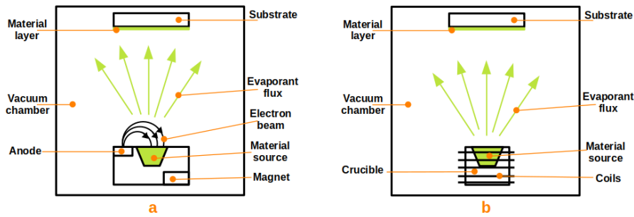
Figure B.1: Schematic drawing of PVD machines based on electron beam gun ( a ) and resistive heater ( b ).
