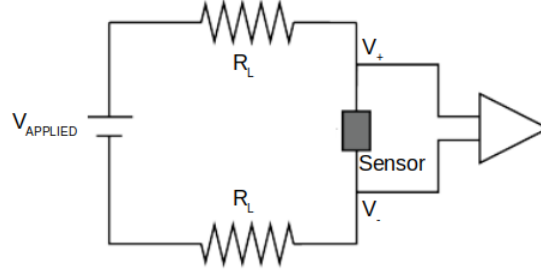
Figure 6.1: Scheme of the bias circuit for the NTD read-out.
