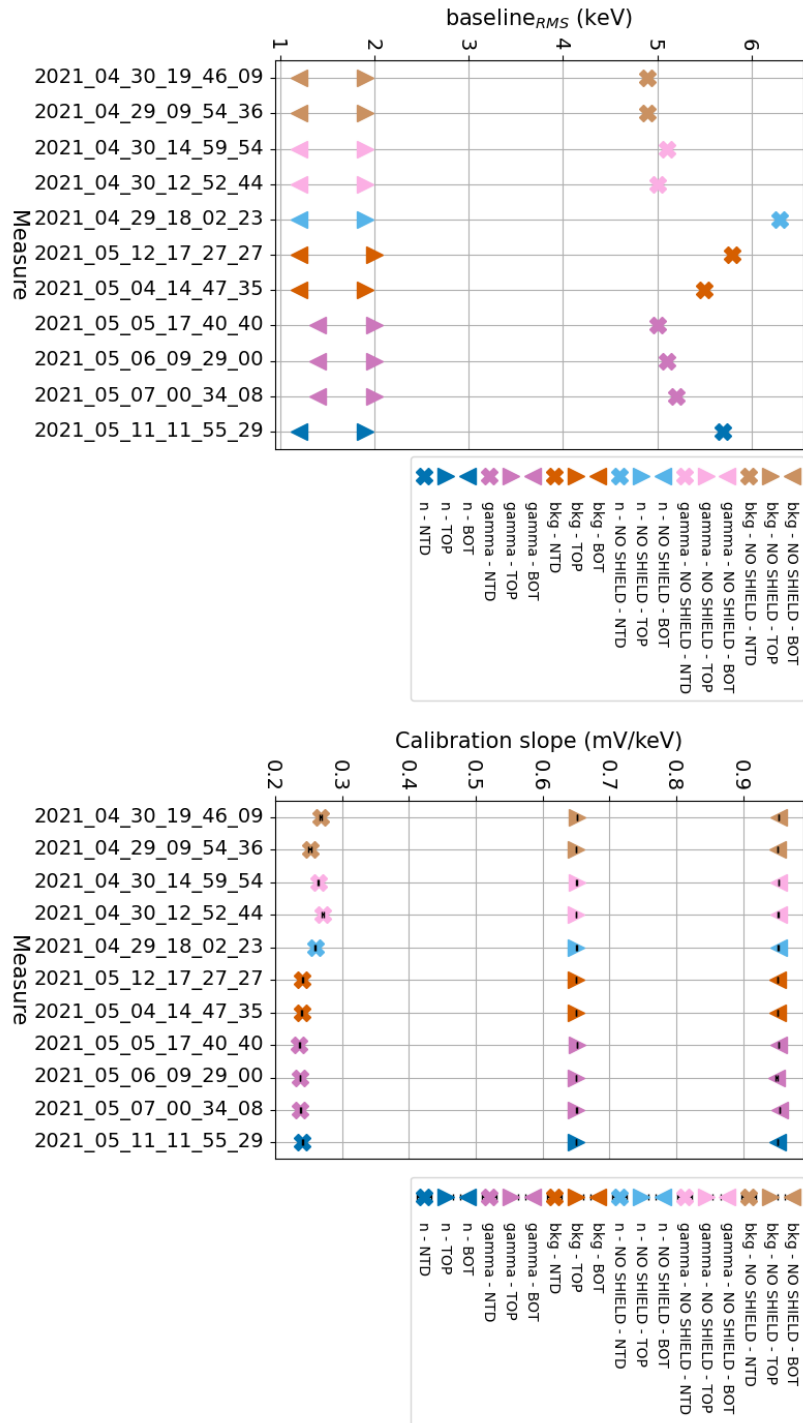
Figure 5.14: Baseline RMS ( top plot) and energy calibration parameter ( bottom plot) of Ge BOT ( \nabla ), Ge TOP ( \triangle ) and NTD ( \times ) in each measurement.
