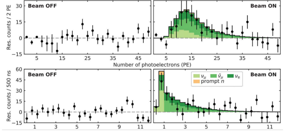
Figure 1.5: Observation of CEνNS by the COHERENT collaboration [19]. The plots show the differences in photon counts between the 12 \mu s after and before a beam trigger as a function of photon number ( top ) and arrival time ( bottom ). The "Beam OFF" data are accumulated during 153.5 live-days of SNS inactivity while the "Beam ON" during 308.1 live-days of neutrino production. An excess following the standard model CEνNS prediction (colored histograms on the right ) was observed for periods of neutrino production only at a significance of 6.7\sigma .
