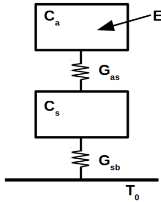
Figure 2.9: Scheme of a simplified cryogenic assuming to have an MMC sensor as the thermometer.
