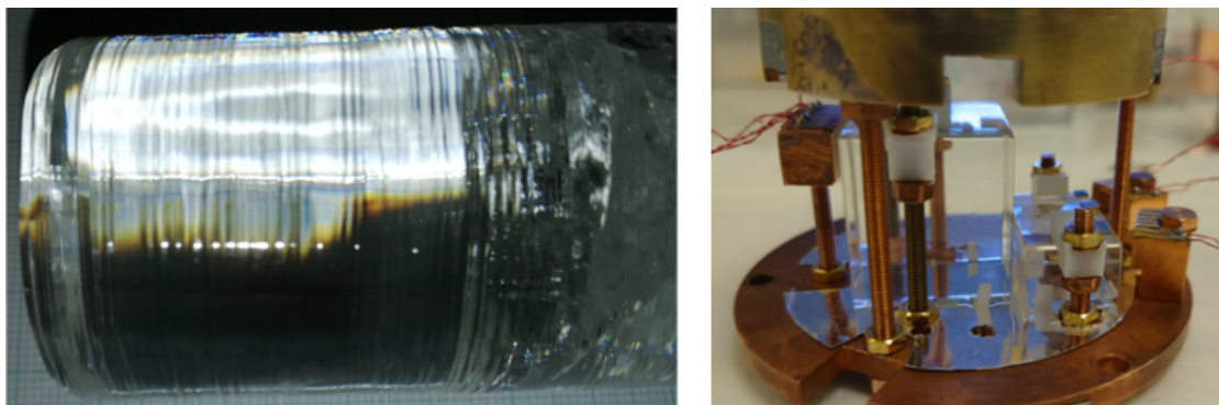
Figure 6.21: Left : \text{Li}_2\text{WO}_4 crystal ( \Phi=3.5 cm, h=3 cm) produced by the french partner. Right : two smaller elements ( 1.4\times2.5\times0.9\text{ cm}^3 and 2.5\times2.7\times2.5\text{ cm}^3 ) cut out from the Grenoble crystal and mounted as detector absorbers to test their performances.
