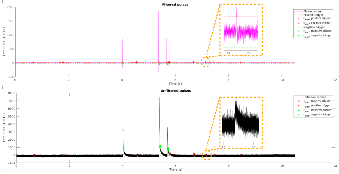
Figure 3.7: Bottom : example of 12 s window of the unfiltered data stream.
