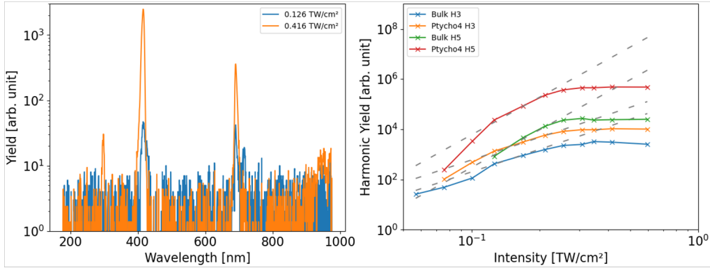
Figure 4.8: (a) Example spectra for two different intensities. (b) Intensity scaling for harmonic 3 and 5. The dashed lines denote a scaling of I^3 and I^5 , which are adjusted to the best matching part of each harmonic to guide the eye.
