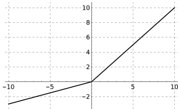
(a) Leaky ReLU function ( \alpha = 0.3 ).
