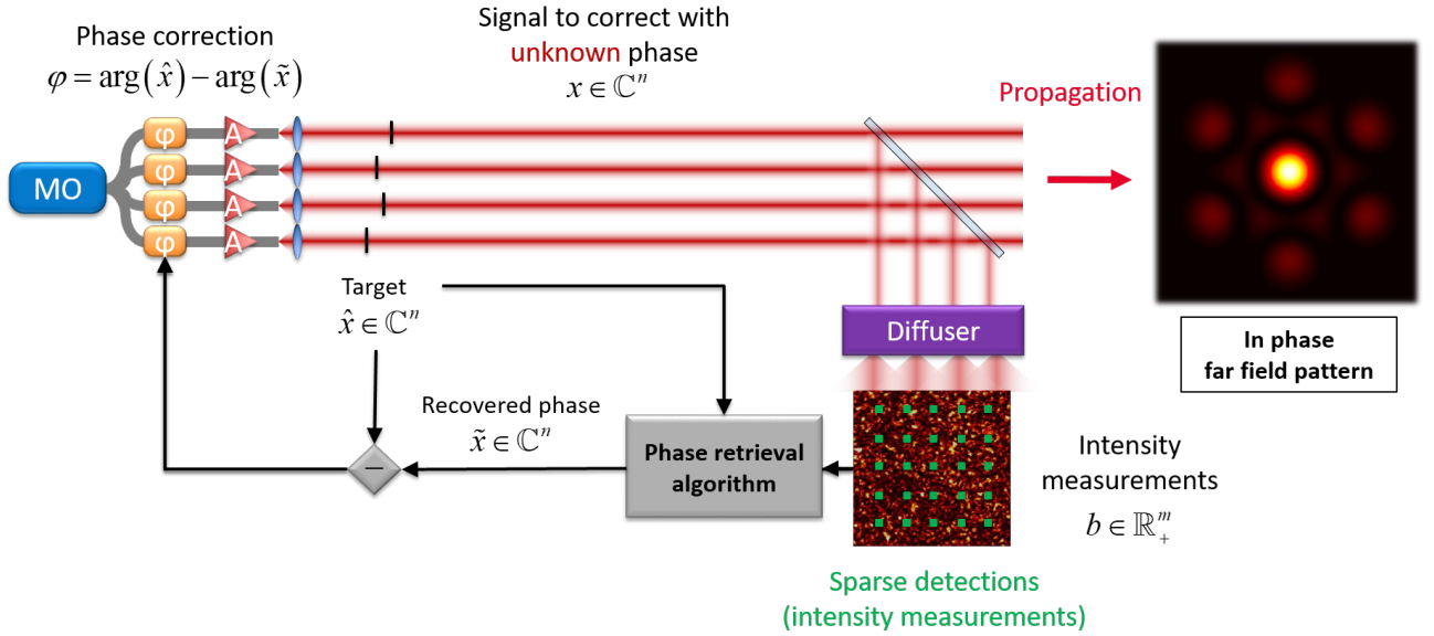
Figure 1.7: Opto-numerical algorithm [31].
