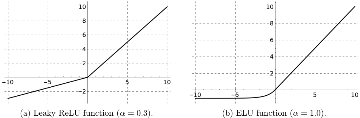
Figure 3.5: ReLU function modifications.
