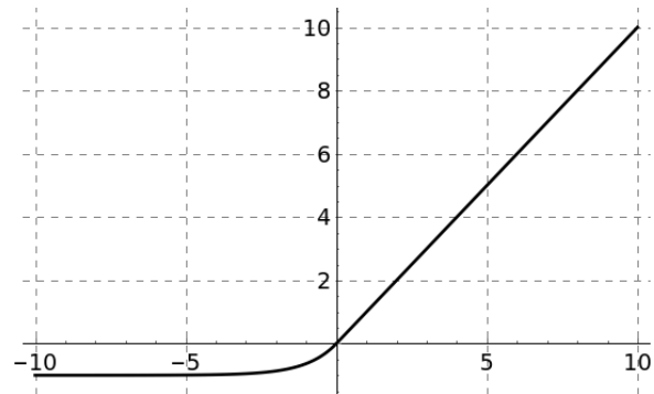
(b) ELU function ( \alpha = 1.0 ).
