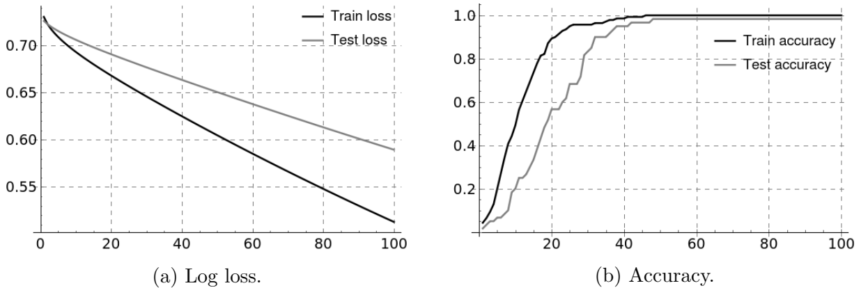
Figure 3.2: Learning process.
