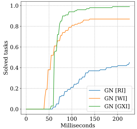
(b) Gauss-Newton (Algorithm 6)
