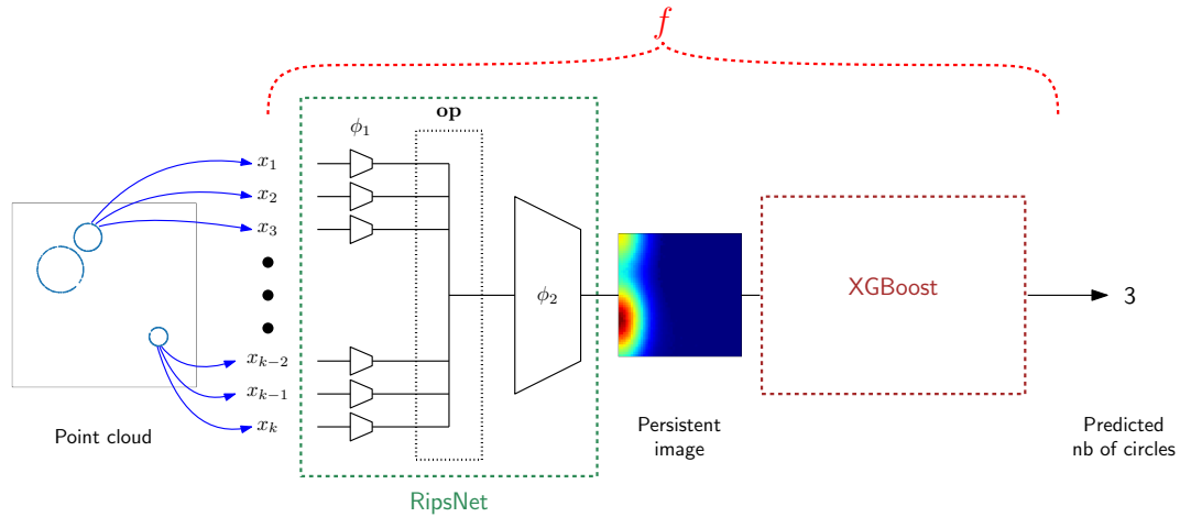
Figure 8.12: An illustration of the classification pipeline f = \text{XGboost} \circ \text{Ripsnet} designed to predict the number of circles in point cloud data.
