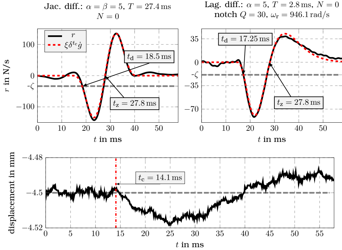
Figure 4.3: Collision detection using Jacobi and Laguerre diff. at a specific hovering position of the plate equal to y = -4.5 mm and a falling height of the ball equal to 15 cm: The detection time and the time instant where the residual r from (4.2) crosses the zero line after the maximum excitation are denoted by t_d and t_z , respectively. The estimated collision time is t_c .
