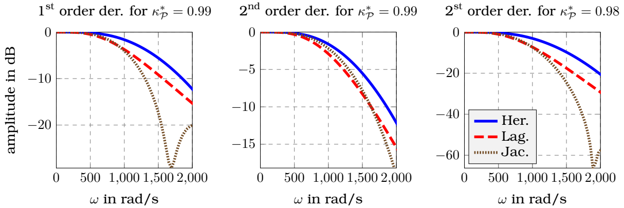
Figure 3.24: Amplitude spectra of the differentiations parametrised using the automatic tuning approach for the estimation of the first and second-order derivatives of the signal x from Example 3.8. The parameters of the diffs. are summarised in Tables 3.9 and 3.10.
