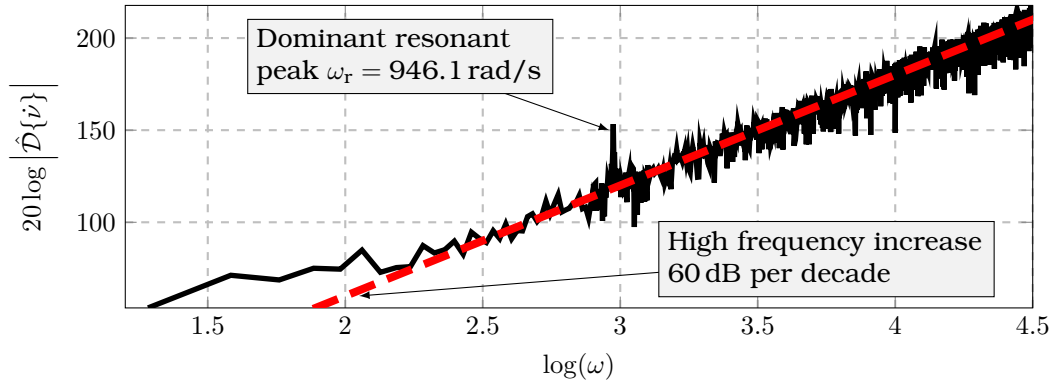
Figure 4.5: Estimated amplitude spectrum from (4.4) of the disturbance \dot{\nu} based on L_m = 2^{17} measurements of the vertical displacement at a hovering position y = -4.5 \text{ mm} .
