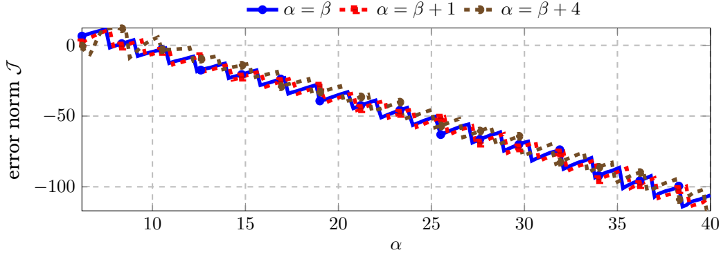
Figure 5.4: Error norm (3.12) for an Jac. diff. with N = 0 and cutoff frequency \omega_c = 500 \text{ rad/s} for different values of the parameters \alpha and \beta .
