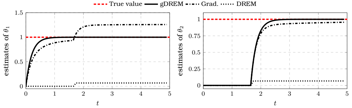
Figure 5.1: Time evolution of the parameter estimates for the system in (5.17) with \Gamma_{\text{gDREM}} = \Gamma_{\text{DREM}} = \Gamma_{\text{Grad}} = [5, 5] using three different approaches.
