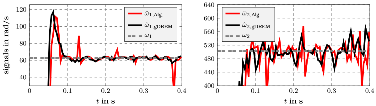
Figure 5.5: Time evolution of the estimates for the experimental case study 1. For the algebraic approach N_{eq} = 6 .
