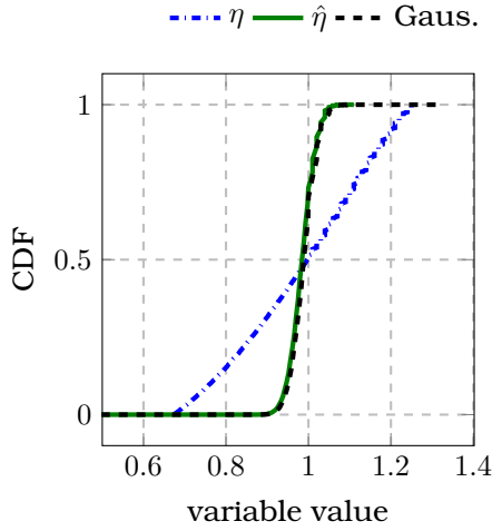
Figure 4.11: CDFs of a random variable \eta = \epsilon^5 + \sqrt{(\epsilon + 1)} with \epsilon drawn uniformly from [-0.5, 0.5] , the filtered variable \hat{\eta} = g_{0,T_g,\vartheta}^{(3,3)} \star \eta , and a normal distribution fitted to \hat{\eta} . The parameters of the differentiator are T_g = 0.045 , N = 0 , and \alpha = \beta = 3 .
