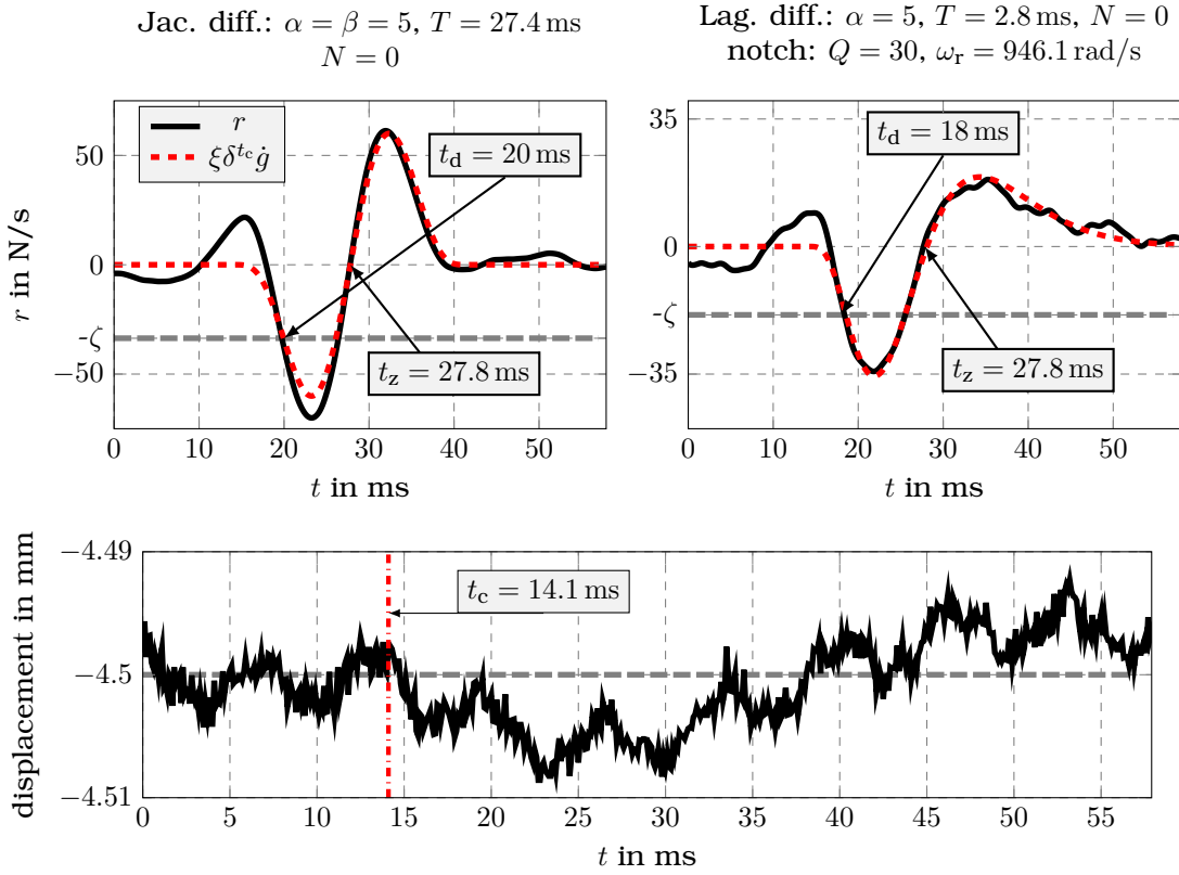
Figure 4.2: Collision detection using Jacobi and Laguerre diff. at a specific hovering position of the plate equal to y = -4.5 mm and a falling height of the ball equal to 3 cm: The detection time and the time instant where the residual r from (4.2) crosses the zero line after the maximum excitation are denoted by t_d and t_z , respectively. The estimated collision time is t_c .
