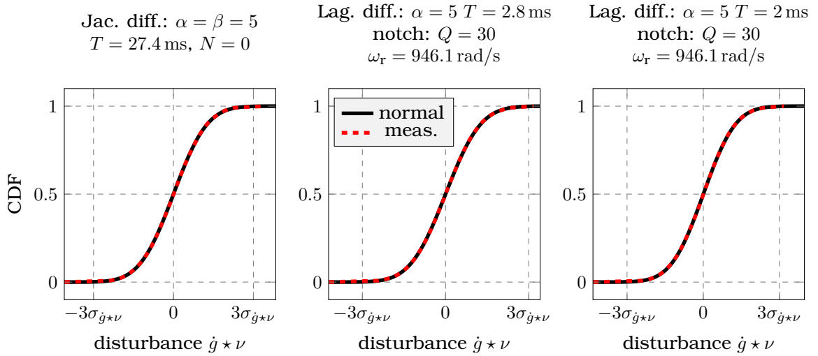
Figure 4.4: CDFs for the residuals in the collision-free case using measurements of the vertical displacement at a hovering position y = -4.5 \text{ mm} .
