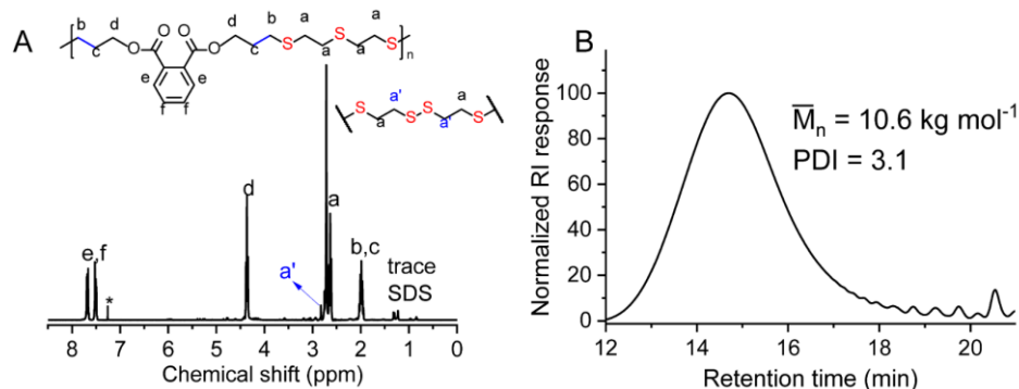
Figure V-1 ^1\text{H} -NMR ( \text{CDCl}_3 ) spectrum ( A ) and GPC trace ( B ) of dried poly(thioether)s resulting from photocatalytic emulsion thiol-ene polymerization of DAP-4 .
