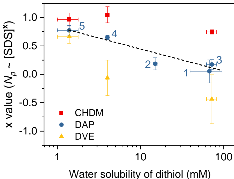
Figure IV-17 Dependence of exponents x of ( N_p \propto [SDS]^x ) on the water solubility of monomer.
