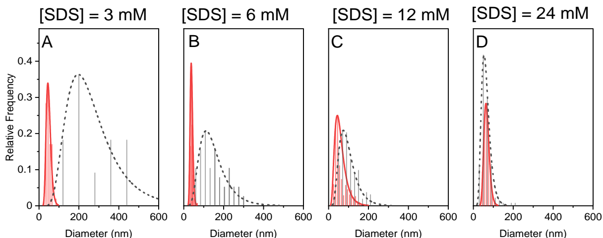
Figure III-11 Effect of initiator solubility on particle size distribution (derived from NS-TEM imaging) of a latex derived from a DAP-3 (with 50 mM DBHQ) miniemulsion (monomer content: 1 wt%) prepared at different surfactant concentrations: Dotted line : TPO as an initiator ; solid line : TPO-Li as an initiator.
