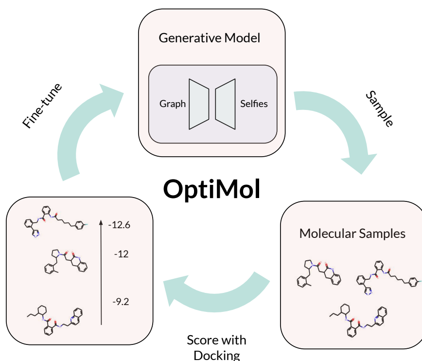
Figure 8.2 – OptiMol workflow: A prior generative model is trained on a broad chemical space and generates samples. We use docking to score these samples, and fine-tune the generative model on the samples weighted by their docking scores
