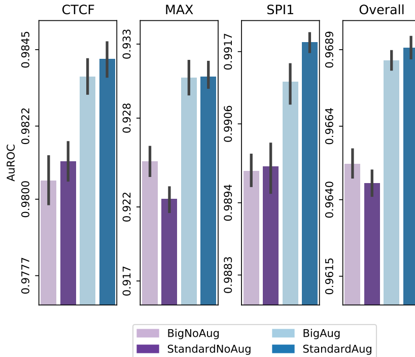
Supplementary Figure B.1 – Binary task performance of a standard, non-equivariant model trained with (“Aug”) or without (“NoAug”) data augmentation, and with more (“Big”) or less (“Standard”) channels.
