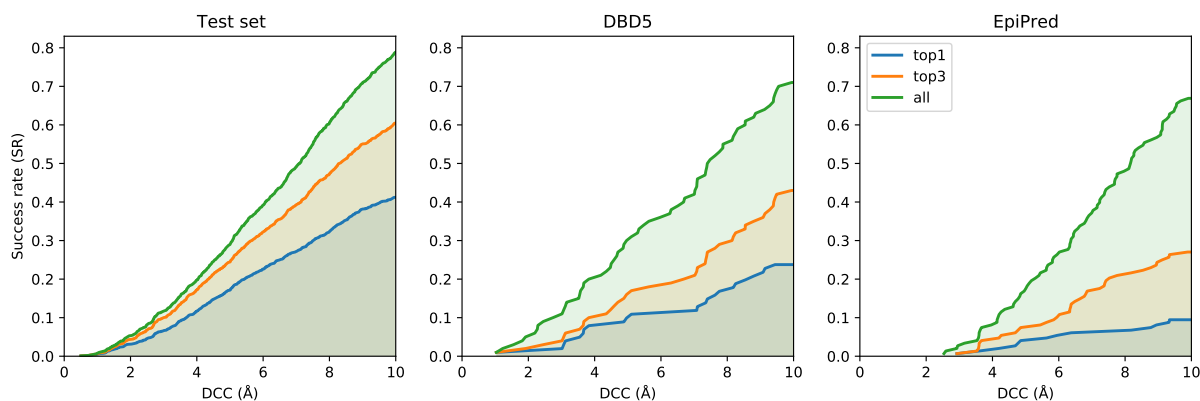
Figure 6.3 – DCC values for InDeep on the test set ( Left ), DBD5 ( Center ) and EpiPred ( Right ) data sets, when considering the best, top-3 or all pockets predicted.
