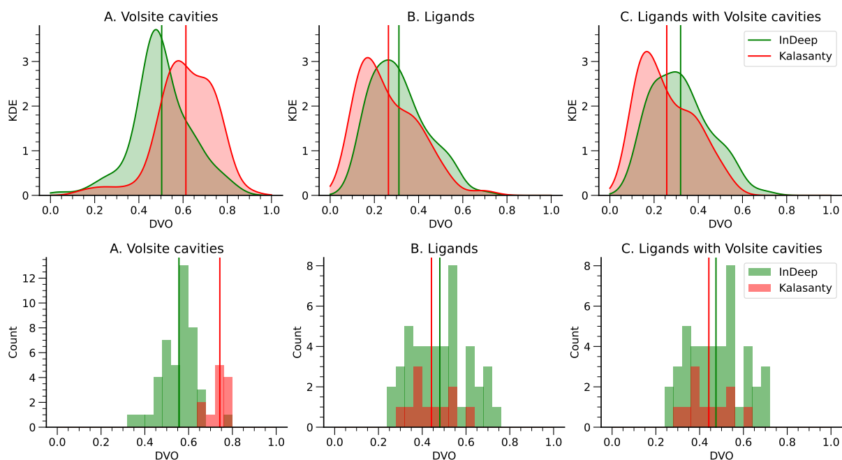
Supplementary Figure E.4 – Distributions of the DVO values for InDeep and Kalasanty on the Chen benchmark ( Top ) and on the test set filtered by TM-score ( Bottom ). We only plot the values for the systems for which the method has a successful DCC of less than 6 Å. The metrics are computed with the VolSite cavities associated with the ligand position given by the PDB ( A. ), the ligand position itself ( B. ) and the ligand position having a cavity detected by VolSite ( C. ).
