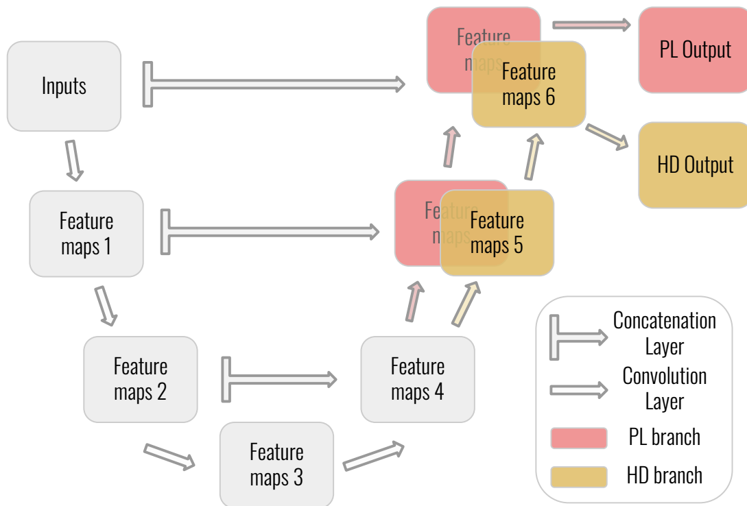
Figure 6.1 – Visual representation of InDeep’s architecture.
