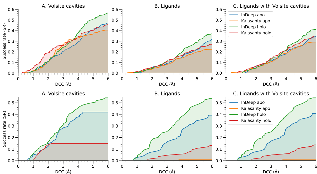
Figure 6.2 – Top : DCC evaluation for InDeep and Kalasanty on the Chen benchmark. We plot the Success Rate (SR), the fraction of systems for which we have a DCC value below a threshold, for different thresholds. Bottom : Performance on the test set filtered by TM-score. The plots are produced following the same procedure as the ones above on this new data set. The metrics are computed with the VolSite cavities associated with the ligand position given by the PDB (A.), the ligand position itself (B.) and the ligand position having a cavity detected by VolSite (C.).
