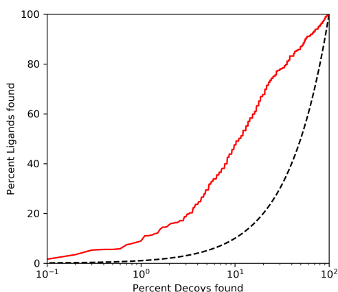
Figure 8.3 – Log-ROC curves for ExCAPE database DRD3 actives and decoys ( red ) and random sampling ( dashed line )
