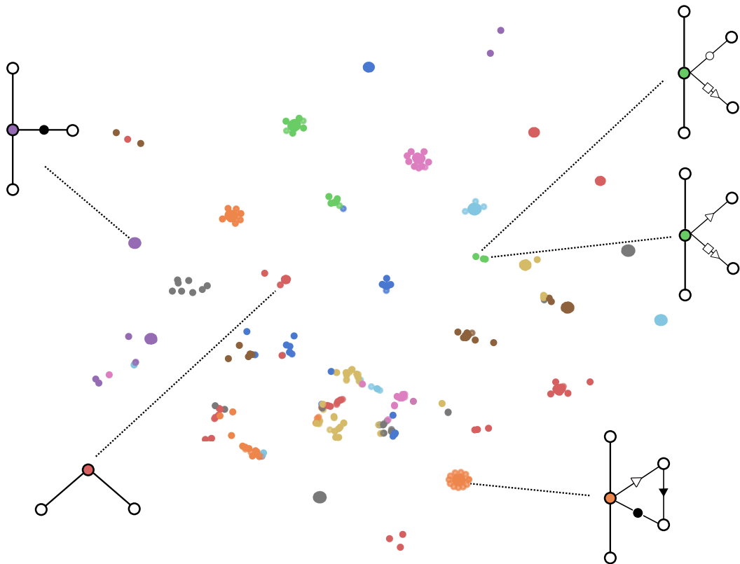
Figure 4.3 – t-SNE projection applied to embedding space. Drawn rooted subgraphs correspond to an example from the cluster connected by a dotted line. Point colors correspond to the nearest mixture model component.
