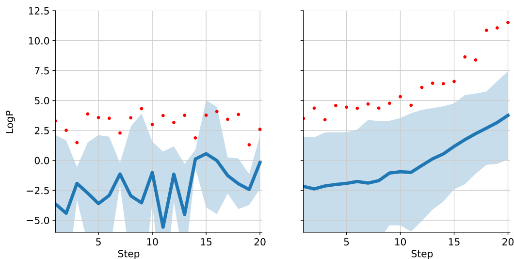
Figure 8.4 – Composite logP optimization results : the blue curve plots the mean and standard deviation of the clogP at each iteration and the red dots show the maximum score.
