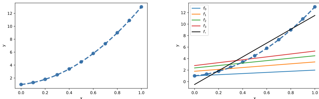
Figure A.1 – The dashed line represents the unknown function and the blue points are our observed data points. Left : The function h(x) = 10 * x^2 + 2 * x + 1 observed on a regular grid. Right : Visualization of the iterations of optimization ; the model is randomly initialized and converges towards the optimal solution.
