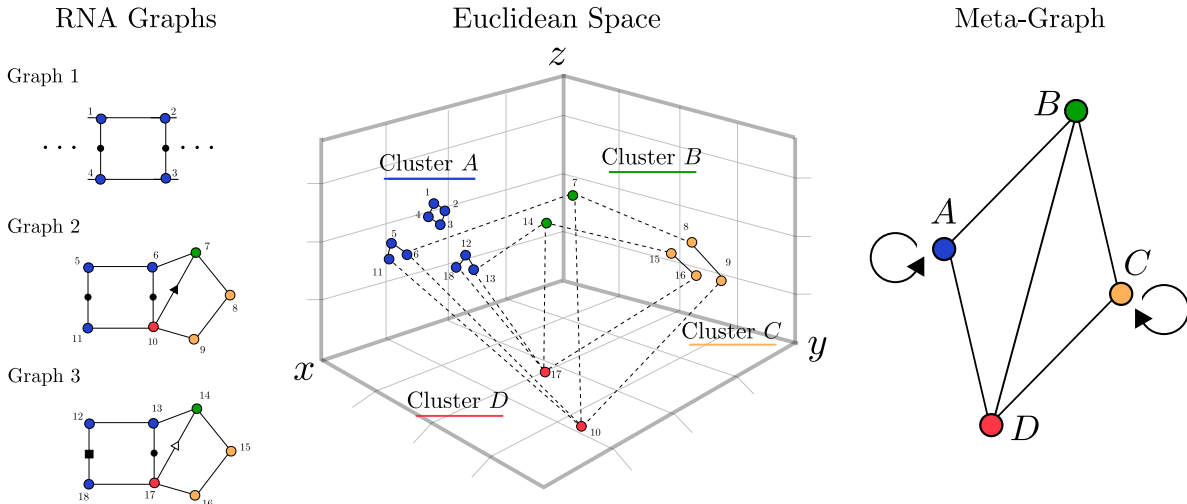
Figure 4.1 – Meta-graph creation : RNA graphs ( Left ) get aligned in the embeddings space ( Middle ) and represented as a meta-graph ( Right ). RNA nodes are grouped in meta-nodes through clustering, which reflects structural similarity. Meta-edges are then inferred from the source graphs connectivity
