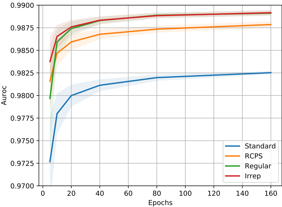
Supplementary Figure B.2 – AuROC performance of the four different models on the three binary classification problems CTCF, MAX and SPI1, as well as their average over the course of learning.
