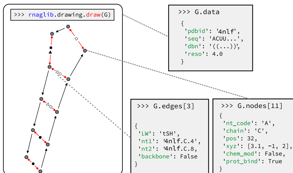
Figure 5.1 – 2.5D graph representation of the 23S ribosomal RNA Sarcin Ricin Loop (PDBID: 4NLF). Left panel shows the output of the drawing tool with default settings. Grey boxes are added later to depict a few of the attributes of the graph object, its nodes and its edges.
