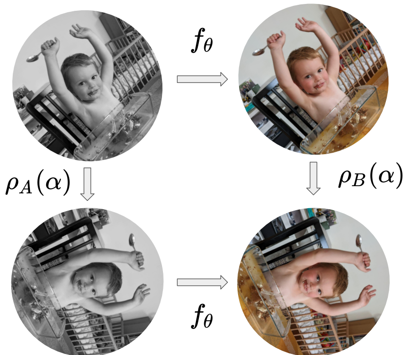
Figure 1.2 – Illustration of the concept of equivariance. If an equivariant colorizing function f_\theta is used, rotation of the input yields a consistent output
