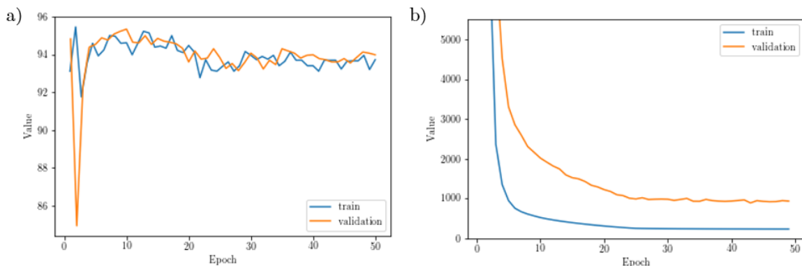
Supplementary Figure F.2 – Fraction of correctly reconstructed characters (a) and KL divergence term (b) during model training, for training and validation set
