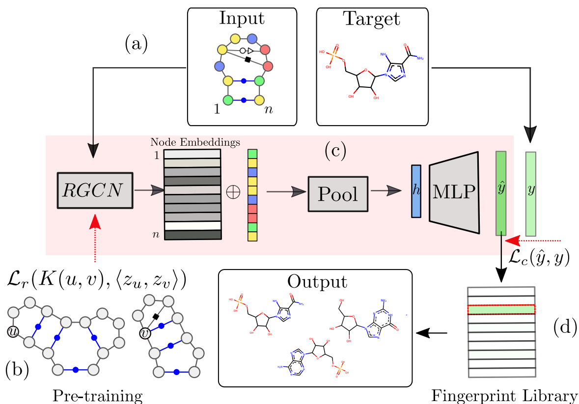
Figure 3.2 – Outline of the RNAmigos pipeline. A base pairing network is passed as input to RNAmigos. In training mode, it is paired with a native ligand (Target) from which a target fingerprint y is constructed. The embedding network (RGCN) produces a matrix of node embeddings of dimension n \times d where n is the number of nodes in the graph, and d is a fixed embedding size. This is followed by a pooling step which reduces node embeddings to a single graph-level vector. Finally, the graph representation is fed through a multi-layer perceptron (MLP) to produce a predicted fingerprint \hat{y} that minimizes the distance \mathcal{L}_c to the native fingerprint y . The fingerprint is then used to search for similar ligands to the prediction in a ligand screen and thus enriches the probability of identifying an active compound. The RGCN network is pre-trained using an unsupervised node embedding framework which allows us to leverage structural patterns from a large dataset of RNA structures. This network is trained to generate embeddings which minimize the distance ( \mathcal{L}_r ) between kernel similarity k(u, v) and embedding similarity \langle z_u, z_v \rangle
