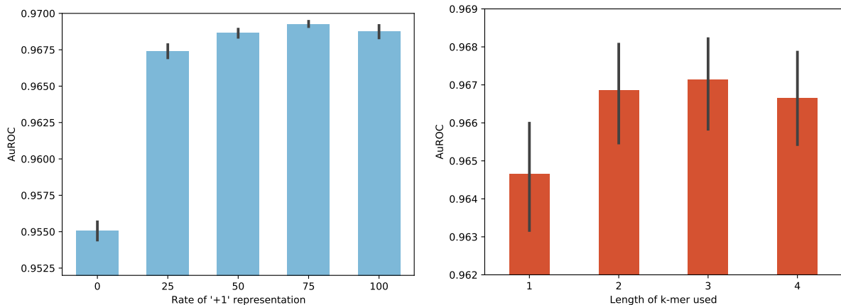
Figure 2.2 – Average AuROC performance across four TFs and 10 random seeds for the Irrep model as a function of a/(a+b) (left, also averaged over k values) and for the Irrep and Regular models as a function of k (right, also averaged over a/(a+b) values for Irrep).
