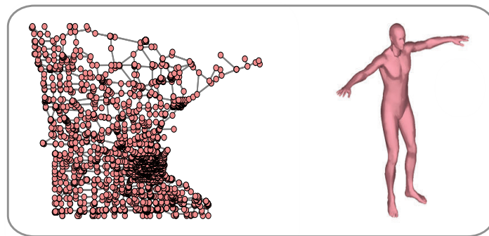
Figure 1.3 – Graph and Riemannian manifold examples. Left : The Minnesota road network where grey lines are the edges and represent roads while red circles are the nodes that represent road intersections. Right : Human represented as a coarse surface or manifold, sampled from the SCAPE database [Anguelov et al., 2005].
