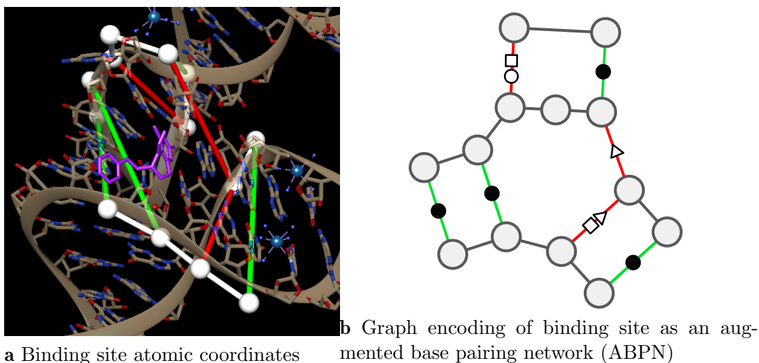
Figure 3.1 – RNA structure representation of the THF riboswitch binding site (PDB: 4LVV) as atomic coordinates using UCSF Chimera [Pettersen et al., 2004](left) and resulting augmented base pairing network (ABPN) (right). We superpose the ABPN in the 3D visualization. Nodes are drawn as white spheres, backbone connections are in white, and canonical and non-canonical base pairs are green and red tubes respectively. We color the edges simply to guide the eye to the corresponding base pairs but note that edge color has no special meaning to our graphs. We annotate the graph representation with the standard Leontis-Westhof nomenclature for pairing type symbols. In this case, the binding site has three canonical interactions denoted (●), and three non canonicals of types (□○, ▷, □▷).
