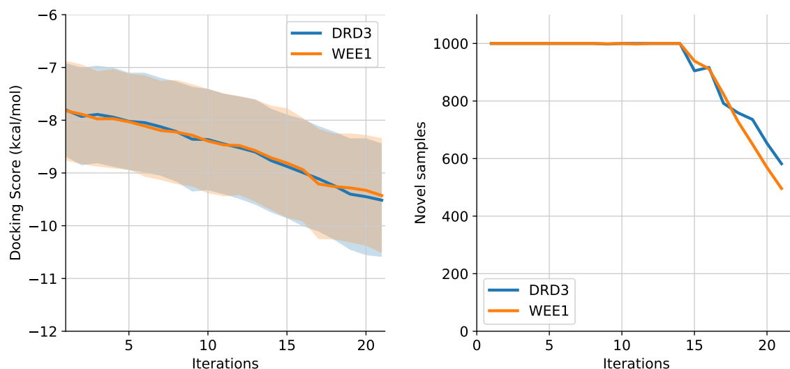
Figure 8.5 – OptiMol training results on DRD3 (blue) and WEE1 (coral). Left : The average and standard deviation of the docking scores obtained at each iteration. Right : The number of compounds never sampled before at each iteration.
