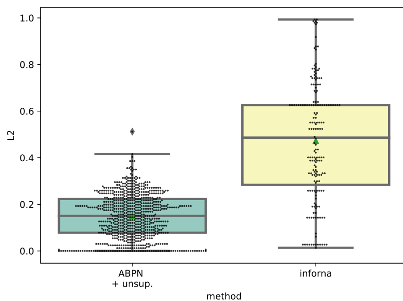
Supplementary Figure C.6 – L2 distance from the native ligand achieved with Infora
