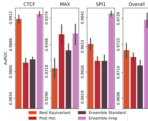
Figure 2.4 – AuROC performance on the three binary classification problems, for the Best Equivariant model, the post-hoc Standard model, and an ensemble of two Standard or Irrep models. Error bars correspond to an estimate of the standard error on 10 repeats with different random seeds.
