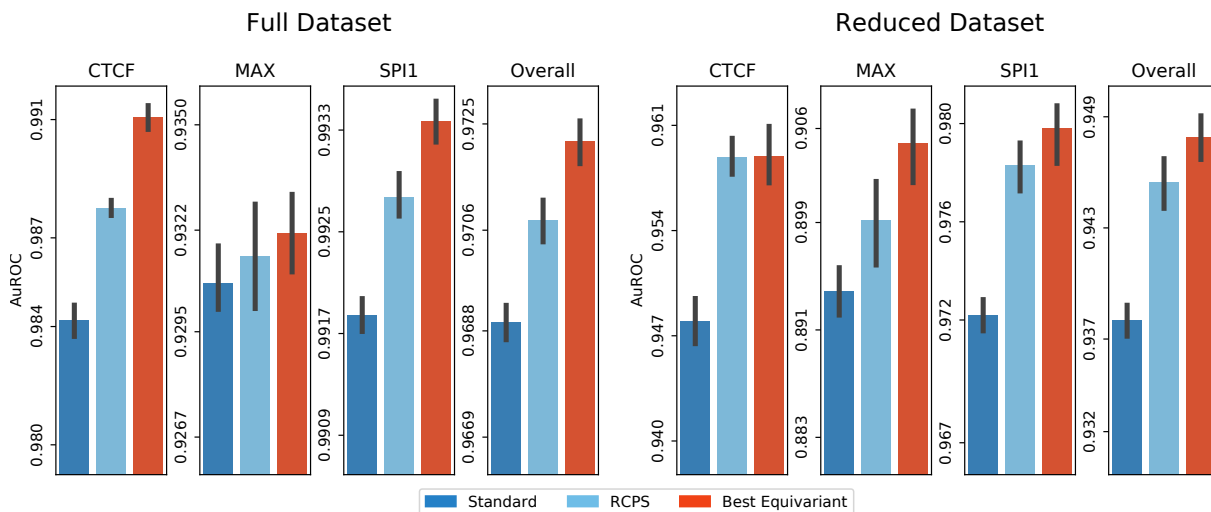
Figure 2.3 – AuROC performance of the three different models (Standard, RCPS and Best equivariant after hyperparameter selection on the validation set) on the three binary classification problems CTCF, MAX and SPI1, as well as their average. Error bars correspond to an estimate of the standard error on 10 repeats with different random seeds. The left plot is the performance on the full datasets, while the right plot shows the performance where models are trained on a subset of 1,000 sequences only (notice the differences of AuROC values on the vertical axis in both plots).
