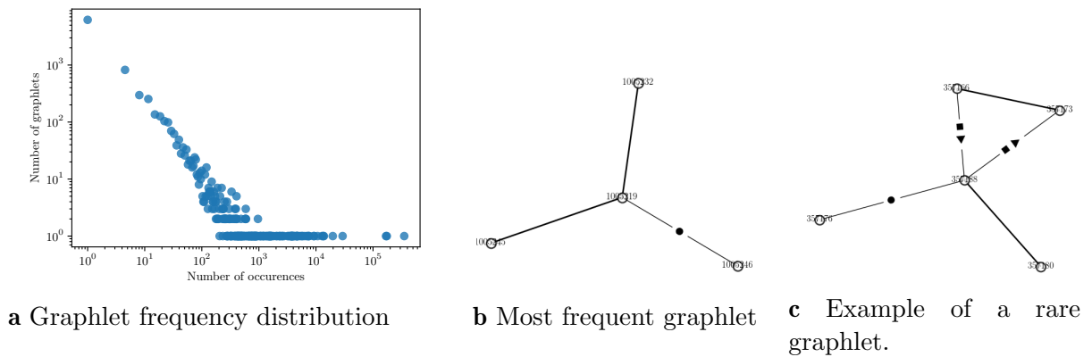
Supplementary Figure D.3 – Graphlet distribution and examples.
