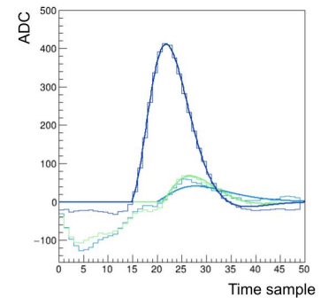
Figure 3.16: Example of waveform obtained involving noisy channels 13 and 31 from sector 0.
