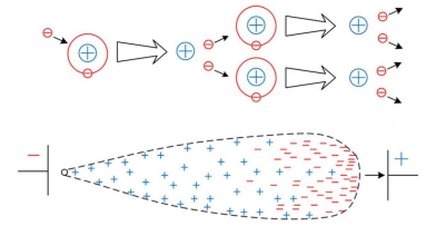
Figure 1.9: Schematic view of the formation of a Townsend avalanche. Taken from [6].
