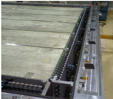
Figure 6.12: Photograph of one of the T2K FGDs.
