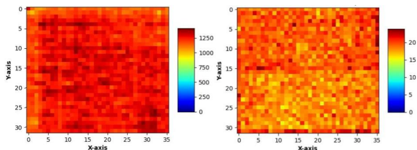
Figure 7.30: 2D map of the relative gain in ADC (left) and the energy resolution in % (right) after modification of the PCB bottom layer. To be compared with Fig 7.28.
