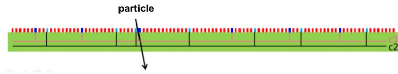
Figure 3.14: Sketch of the principle of genetic multiplexing illustrated by a particle which induces a signal on channel c_1 and c_2 . Taken from [43]
