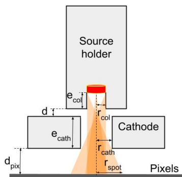
Figure 4.16: Schematic side view of the radioactive source collimation system.
