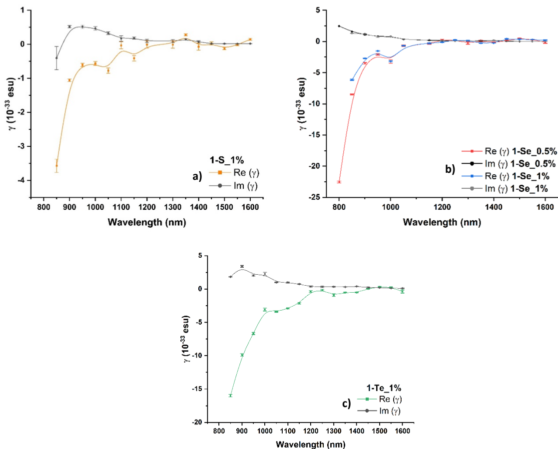
Figure 60. Spectra displaying the calculated real ( \text{Re} ) and imaginary ( \text{Im} ) parts of the hyperpolarisability, \gamma , derived from the Z-scan measurements for a) 1-S , b) 1-Se_0.5 and 1-Se_1 , and c) 1-Te .
