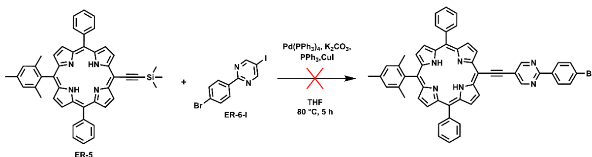
Figure 40. Unsuccessful strategy of the coupling of the acetylated porphyrin ( ER-5 ) and the iodinated para-substituted pyrimidine ( ER-6-I ).
