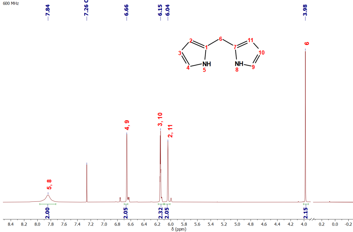
Figure 42. 1 H-NMR spectrum of dipyrromethane ER-2.
