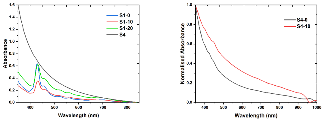
Figure 13. Left: Absorbance spectra of S1-0 , S1-10 , S1-20 , and S4 ( S1-0 : \lambda_{\text{max}} = 429 nm, S1-10 : \lambda_{\text{max}} = 431 nm, S1-20 : \lambda_{\text{max}} = 433 nm). Right: Normalised absorbance spectra of S4-0 and S4-10 .
