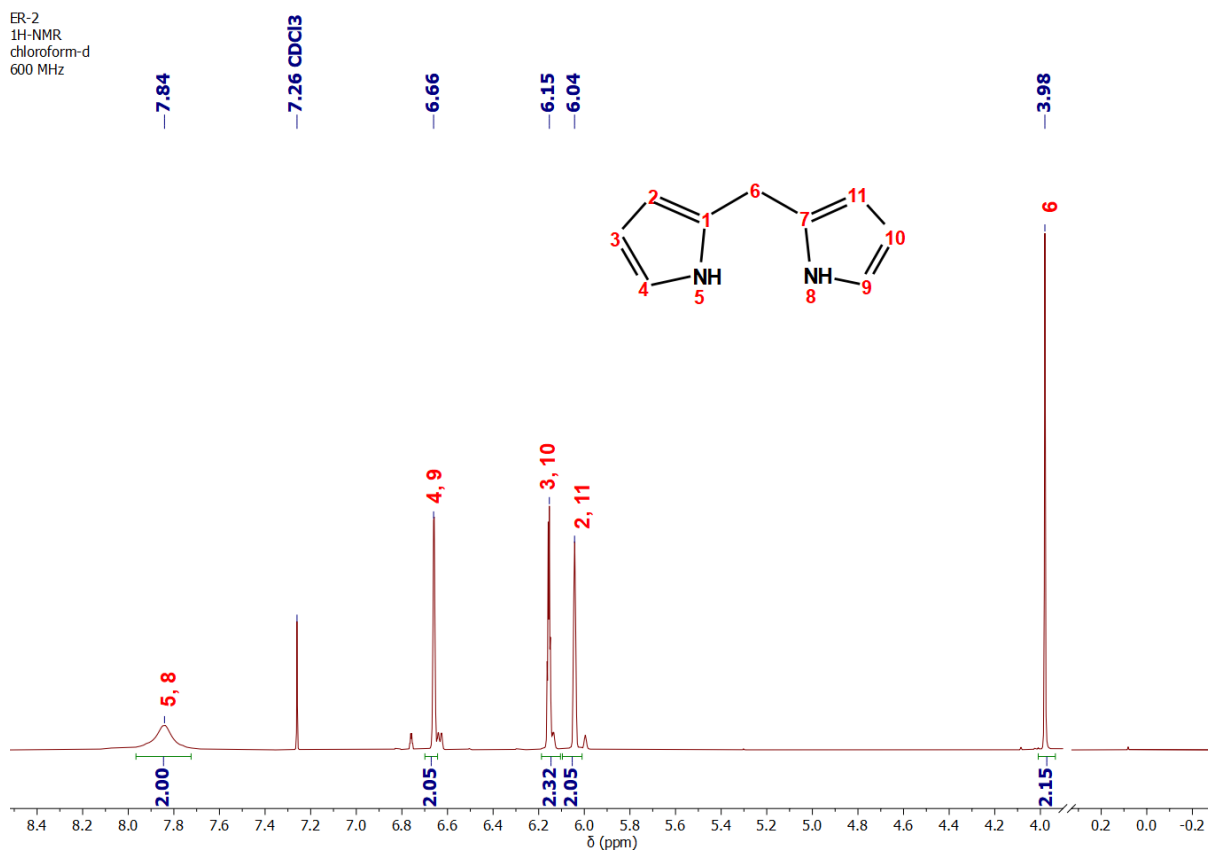
Figure 42. 1 H-NMR spectrum of dipyrrmethane ER-2.
