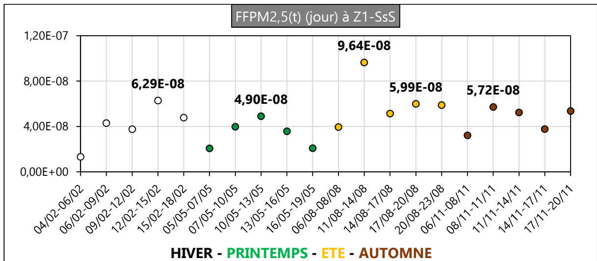
Figure III. 57 : \text{FF}_{\text{PM}_{2,5}}(t) (jour) en zone Z1-SsS en 2020
