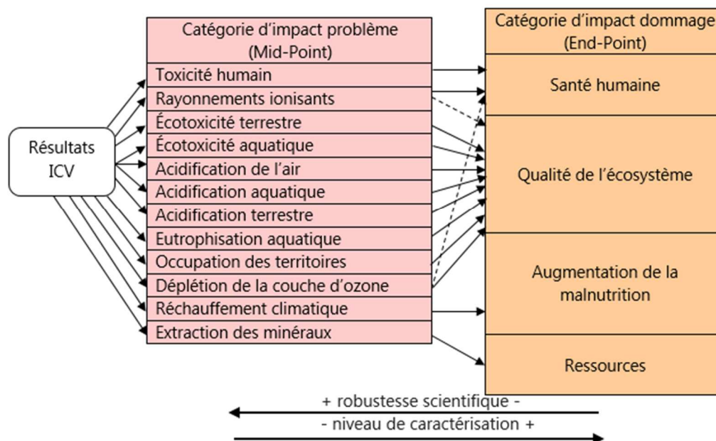
Figure I. 8 : Méthodes Midpoint/End-Point inspirée de [Jolliet et al., 2004]
