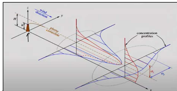
Figure I. 16 : Illustration de la distribution gaussienne d'un panache (Source: John M. Stockie, The mathematics of atmospheric dispersion modelling)
