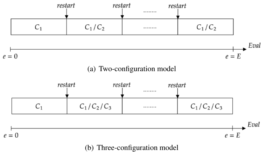
Figure 5.2: Roulette multi-configuration Model
