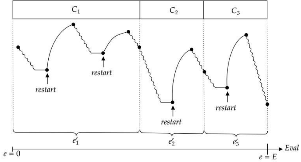
Figure 4.1: Sequential Multi-configuration ILS
