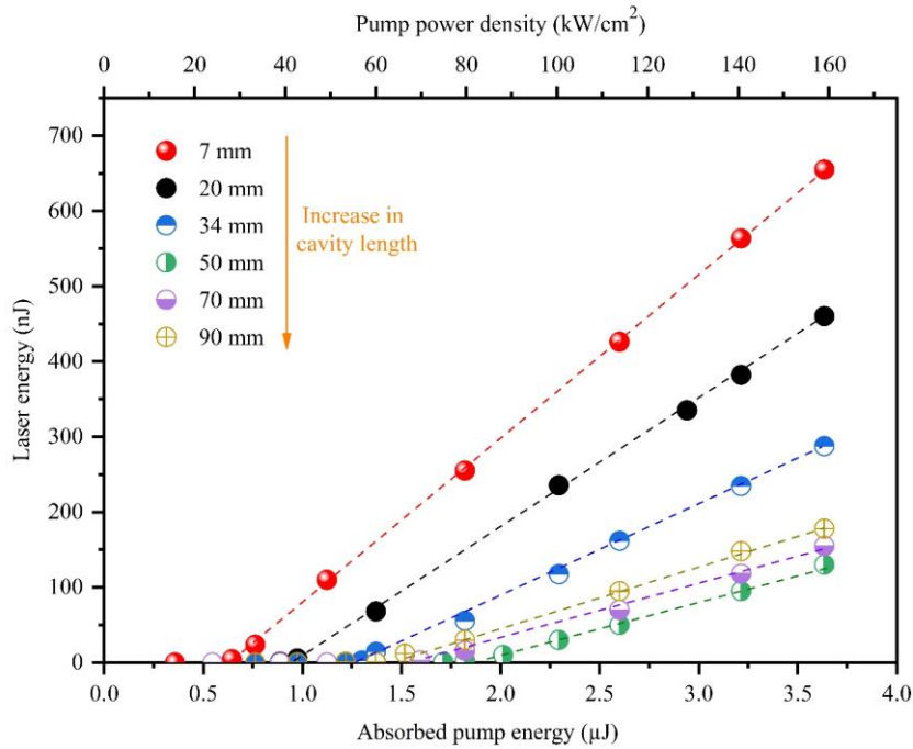
Figure 2.12: Laser energy (nJ) as a function of absorbed pump (200 ns) energy (μJ) (bottom x axis) and pump power density (kW/cm²) (top x axis) for different cavity lengths.
