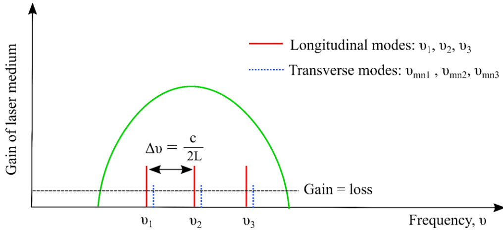
Figure 4.2: Three longitudinal modes of a resonant laser cavity are separated by free spectral range, \text{FSR} = \Delta\nu = \frac{c}{2L} . Lasing can be obtained at either of these frequencies which possess the highest gain over others.
