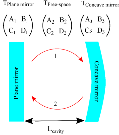
Figure 2.6: Transfer matrix calculation of a plano-concave laser cavity for one round trip. Each element inside cavity e.g., plane mirror, concave mirror, propagation in free space etc. is defined by 2x2 transfer matrix. Arrow 1 mentions that the ray travels through free space from plane mirror to concave mirror and bounces back towards plane mirror to complete single round trip which is shown by arrow 2.
