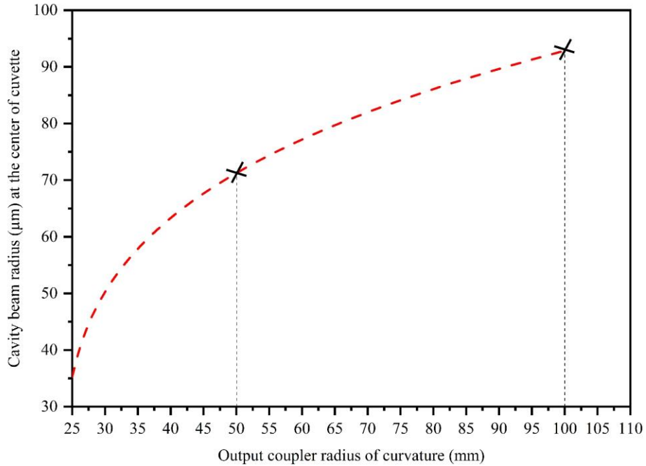
Figure 3.24: Cavity beam radius (μm) on cuvette in the case of a near hemispherical cavity configuration using 25 mm output coupler and also for the case when the output coupler radius of curvature was changed to 50 mm and 100 mm keeping cavity length fixed.
