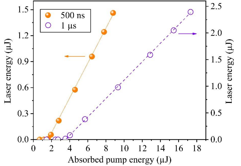
Figure 2.11: Left: Laser energy (μJ) for 500 ns pump, Right: Laser energy (μJ) for 1 μs pump as a function of absorbed pump energy (μJ).
