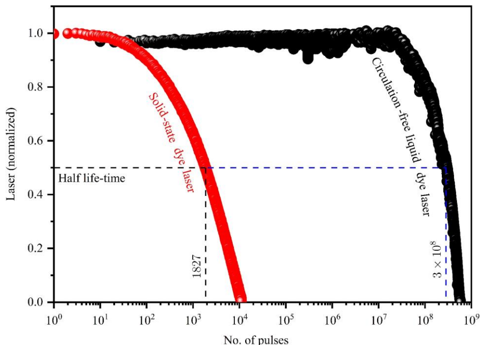
Figure 2.24: Photo-stability of circulation-free liquid dye laser (using 0.03 mL DCM solution in 1-mm light path cuvette) and solid-state dye laser (using 17- \mu m DCM film) at \sim 122 \text{ kW/cm}^2 pump (50-ns, 1 kHz) power density. The absorption of both liquid and solid-state samples was around 83% at 445 nm.
