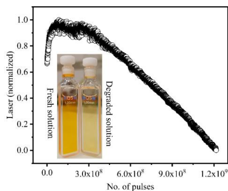
Figure 2.25: Laser photo-stability (in no. of pulses) using 0.3 mL dye solution (DCM in propanol-2 contained in circulation-free 1 mm cuvette) using 122 \text{ kW/cm}^2 pump (50 ns) at 1 kHz repetition rate.
