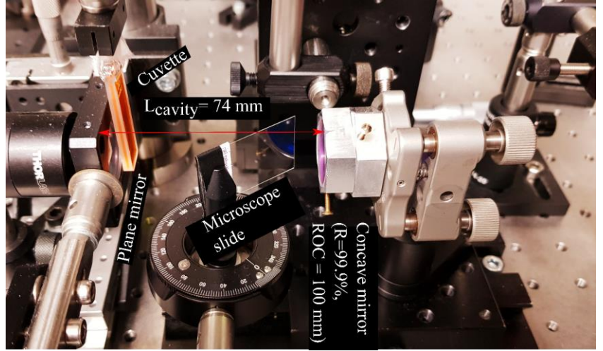
Figure 2.21: Increasing losses (in same amount) in a Plano-concave laser cavity by rotating thin (150 \mu m) microscope by known degree.
