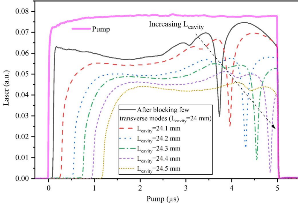
Figure 4.30: Temporal behavior of a multimode laser when increasing the cavity length by translating output coupler mirror.
