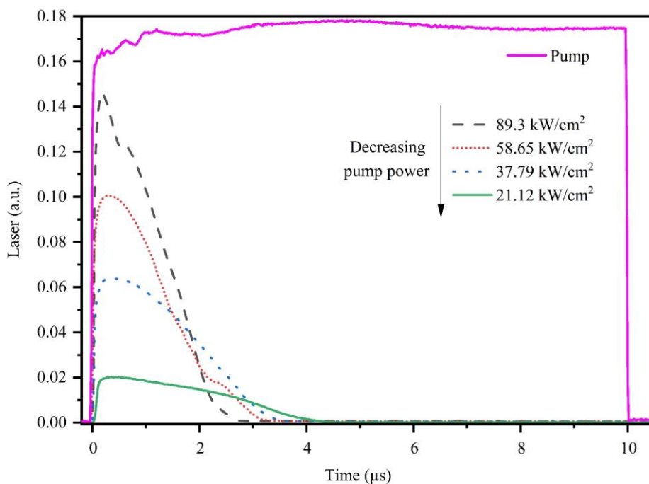
Figure 4.15: Laser temporal profile for different pump (10 \mu s) power densities ( \text{kW}/\text{cm}^2 ).
