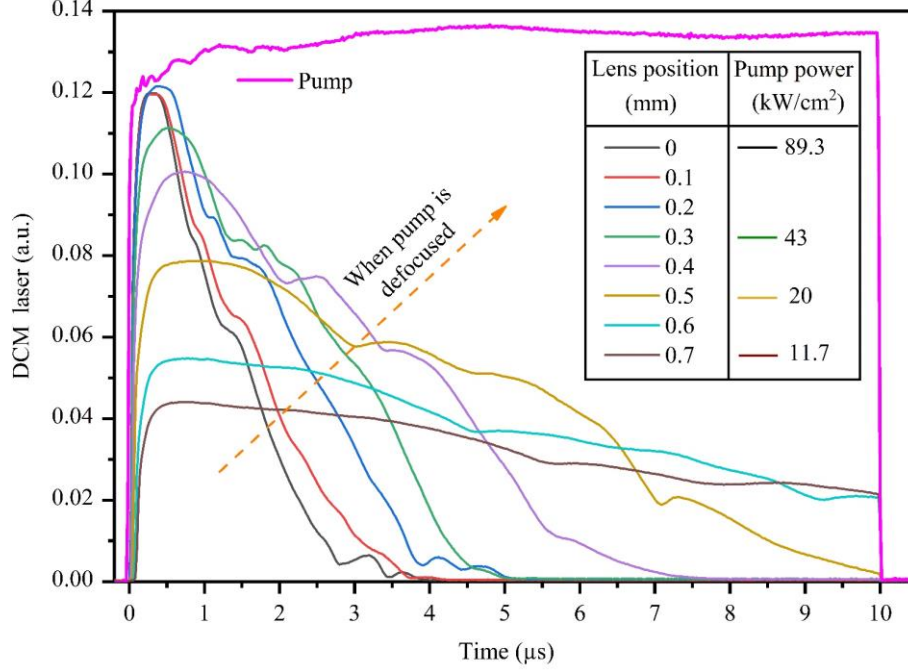
Figure 4.6: DCM laser pulse duration when 10\ \mu\text{s} long pump is focused on the cuvette. The lens position in this case is defined as 0 mm. Then the lens is moved backward direction (e.g., away from plane mirror) up to 0.7 mm with 0.1 mm step corresponding to a decrease in pump power density ( \text{kW}/\text{cm}^2 ). Laser pulse duration is also plotted for each lens displacement.
