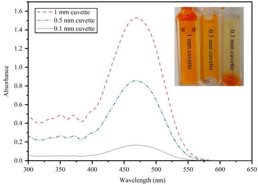
Figure 2.5: Absorbance (a.u.) of the highest concentration of gain medium (DCM in propanol-2) inside spectroscopic cuvettes of different path-lengths (0.1 mm, 0.5 mm and 1 mm).
