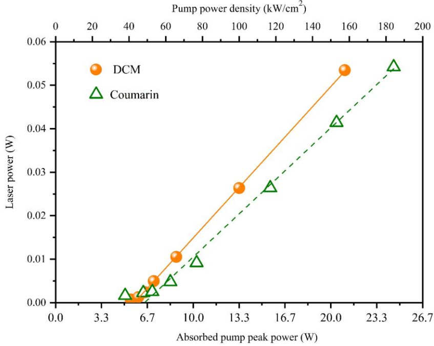
Figure 3.4 : Laser peak power (W) using DCM and Coumarin-540 dyes as a function of absorbed pump peak power (W) (bottom x-axis) and pump power density ( \text{kW}/\text{cm}^2 ) (top x-axis). Output coupler radius of curvature is 50 mm with reflectivity 99.9% at laser wavelength.
