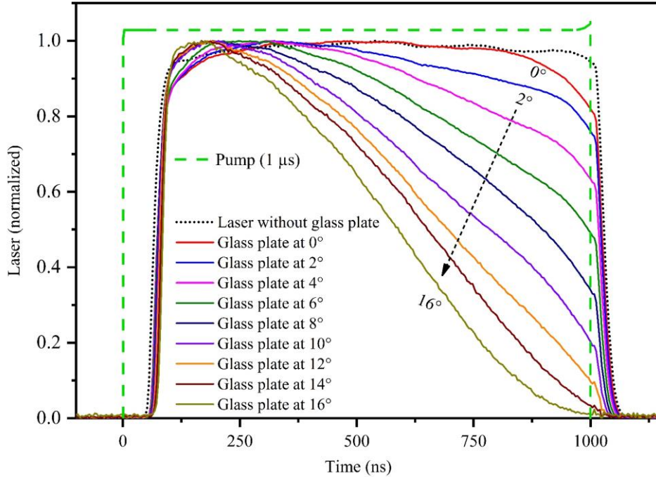
Figure 2.22: Laser temporal behavior by rotating a microscope slide (glass plate) inside laser cavity by known degrees. 1 \mu s (10 Hz), 120 kW/cm 2 pump power density was used for the experiment.
