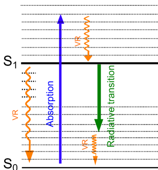
Figure 1.2: Schematic to explain vibrational relaxation from vibrational energy levels of each electronic state.
