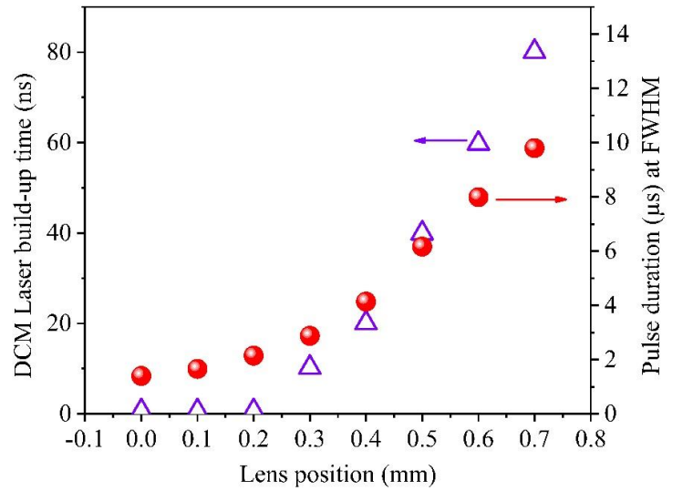
Figure 4.7 : Left: Laser build-up time, right: laser pulse duration at FWHM.
