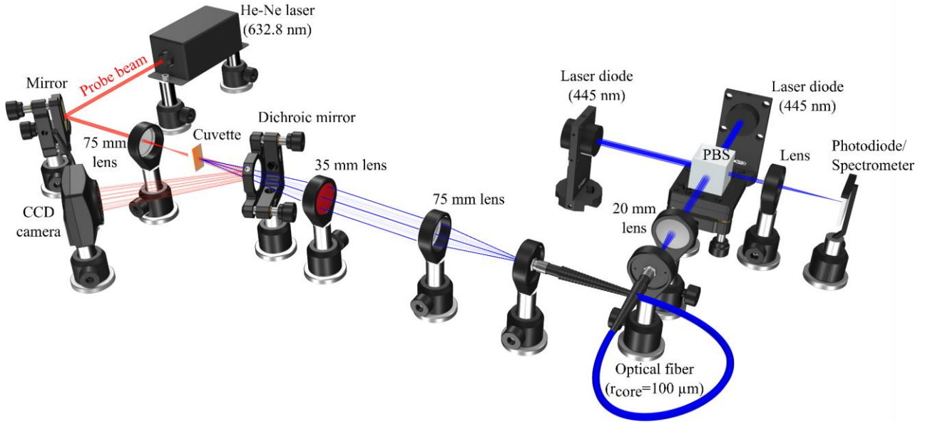
Figure 3.9: Schematic of pump-probe experiment performed by removing the cavity mirrors of laser experimental setup. He-Ne laser (at 632.8 nm) is chosen to probe the pump spot on the cuvette since DCM does not absorb at this wavelength. The pump and probe beam collinearly overlapped onto the liquid cuvette from opposite ends with spot sizes around 120 \mu\text{m} and 100 \mu\text{m} in diameters, respectively. A CCD camera was placed at 7.7 cm after the sample to monitor probe beam size when increasing the pump repetition rate at a fixed pump peak power \sim 77.4 \text{ kW}/\text{cm}^2 ( \sim 1.6 times the laser threshold).
