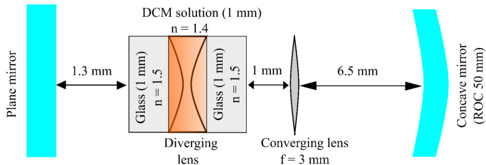
Figure 3.16: Design of a Plano-concave laser cavity by employing an extra converging lens ( f = 3 mm) to compensate thermal lens effect of the laser medium.
