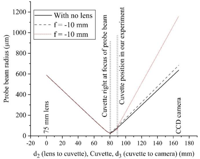
Figure 3.11: Here the cuvette contains a 10 mm (in absolute value) diverging lens. Probe beam divergence (after cuvette) remains almost insensitive to such diverging lens when the cuvette is placed right at the focus of probe beam. When the cuvette is placed one Rayleigh length after focus as used in our experiment (Figure 3.9, Figure 3.10, Figure 3.12), significant divergence of probe beam indicates the sensitivity of our measurement.
