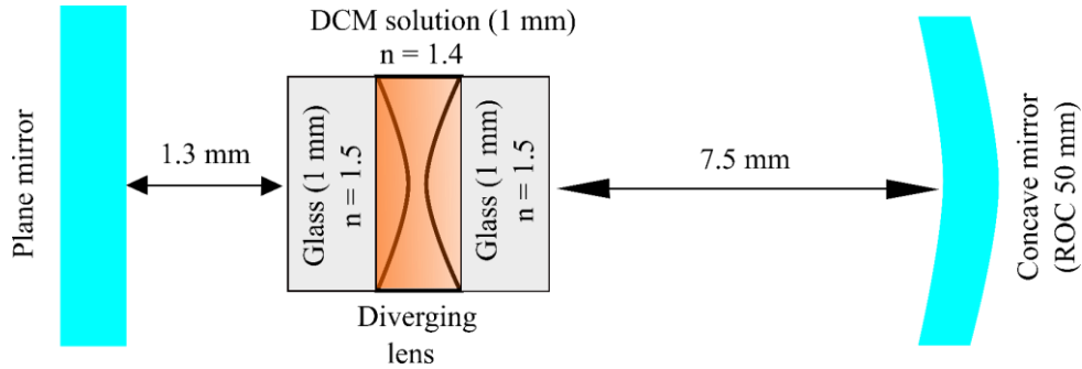
Figure 3.7: Schematic of Plano-concave cavity used for the cavity stability simulation as well as laser experiment. A diverging lens is placed inside cuvette to mimic pump induced thermal lens inside the laser cavity.
