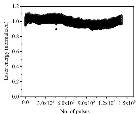
Figure 2.28: Photostability of a liquid dye laser at 113 \text{ kW/cm}^2 pump (1- \mu\text{s} , 50 Hz) power.
