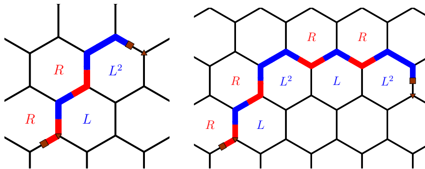
Figure 3.13: Paths encoded by RLRLLL & (RLRLLL)^2 in the hexagonal graph \mathcal{H} .
