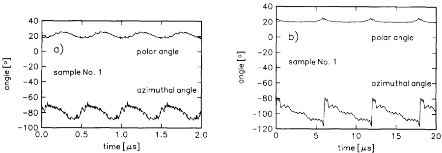
Figure 2.13: Real-time variations of the polar angle \theta(t) and azimuthal angle \varphi(t) at instability conditions. Excitation frequency f_{ex} = 1420 \text{ MHz} . [24].
