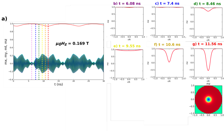
Figure 5.11: a) Time evolution of average components of magnetization for the 700 nm disk, at \mu_0 H_z = 0.169 T during 30 ns (zoom of Figure 5.7 e). b-g) Spatial profile of the longitudinal normalized magnetization at different times of the dynamics corresponding to the different colored dashed lines of Figure a. The 2D profile is shown for the last case.
