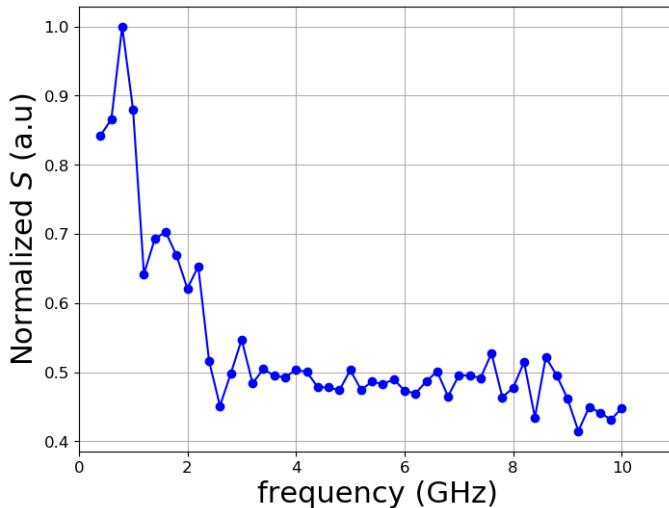
Figure C.1: Evolution of the normalized calibration parameter between power and microwave field as a function of frequency.
