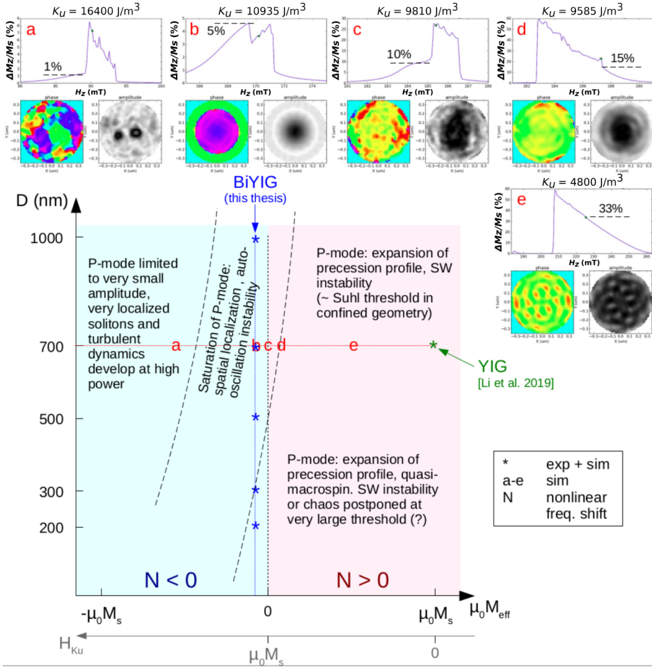
Figure 5.25: Draft of the phase diagram in parameter space ( M_{eff} , Diameter) equivalent to ( K_u , Diameter), with the perpendicular magnetic anisotropy constant K_u and the effective magnetization M_{eff} increasing in opposite directions as shown on the x-axis. a-e) Simulated resonance lines of the 700 nm disk at f = 5 GHz and \mu_0 h_{rf} = 1.0 mT, for a perpendicular static field, for different values of the effective magnetization M_{eff} , ranging from highly negative to highly positive as shown by the corresponding points a) to e) on the phase diagram. In each case, the large amplitude branch is shown, the maximum amplitude of the signal \Delta M_z / M_s reached before the onset of instabilities is indicated and a typical precession profile (phase and amplitude) in the instabilities regime is shown below the resonance line.
