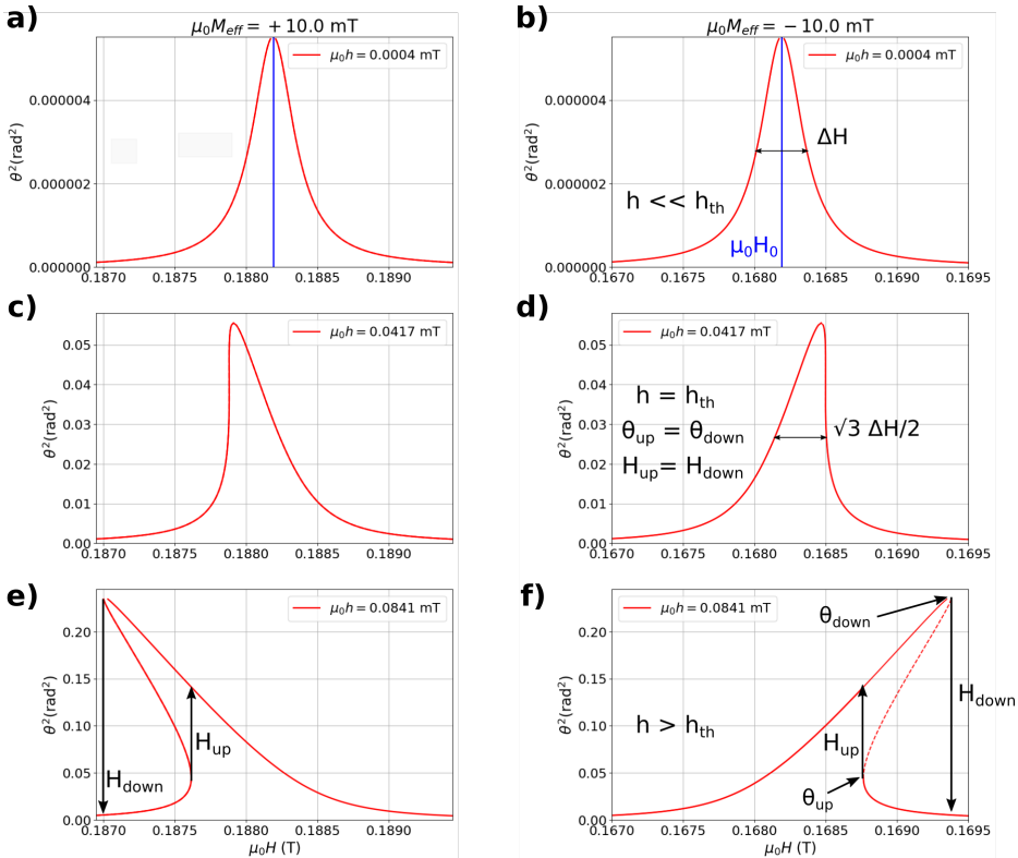
Figure 2.8: The calculated \theta^2 for a FMR at f = 5 GHz, at three values of h , h = 0.01h_{th} , h = h_{th} and h = 2h_{th} for M_{eff} > 0 (a-c-e) and for M_{eff} < 0 (b-d-f). The parameters used are \mu_0 M_{eff} = \pm 10 mT, \alpha = 0.001 , \gamma/2\pi = 28 GHz/T.
