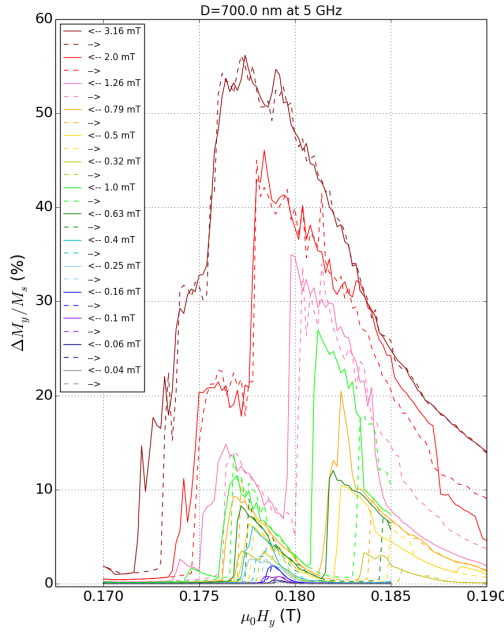
Figure 6.6: Evolution of the simulated spectrum of the 700 nm disk at f = 5 GHz as a function of the excitation field.
