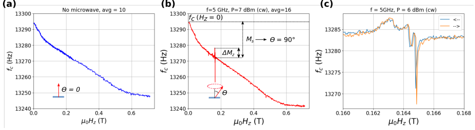
Figure 5.16: Variation of the cantilever frequency when the probe is above the 700 nm disk B4 a) without microwave and b) with microwave. The insets show a zoom on the resonance signal and the procedure used for a direct calibration of the signal in mean precession angle. c) Resonance signal for both directions of field sweep: absence of hysteresis cycle.
