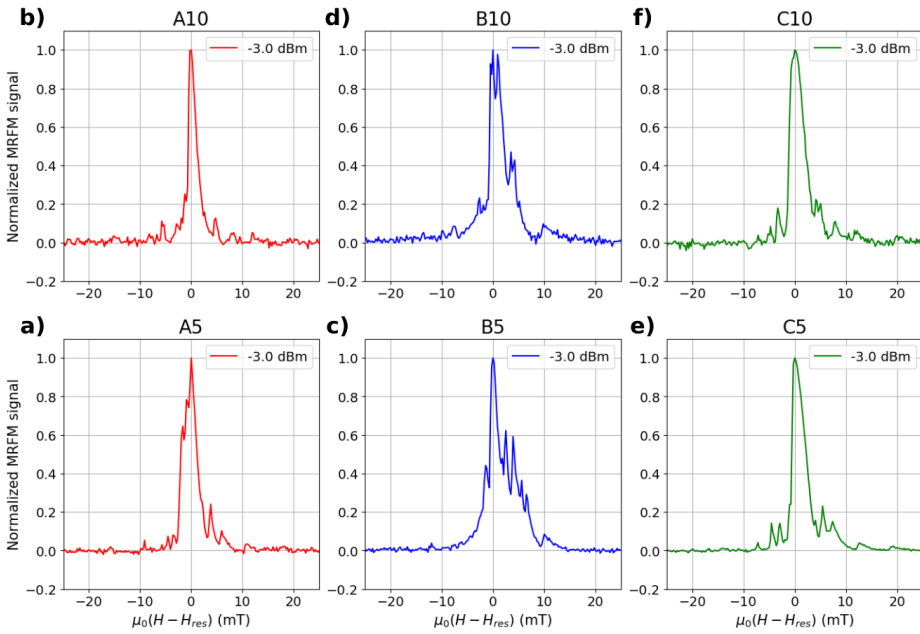
Figure I.6: MRFM spectra of the 1000 nm diameter disks at f = 5 GHz.
