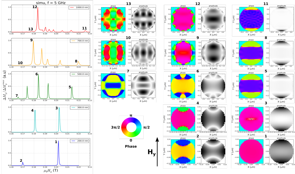
Figure 6.2: Normalized simulated spectrum at f = 5 GHz of the different disks sizes arranged in row by decreasing lateral size. The 2D profiles (phase and amplitude : dark = high amplitude, white = zero amplitude) of the modes corresponding to the numbered peaks on the spectra are shown on the right. The field is applied along the y axis.
