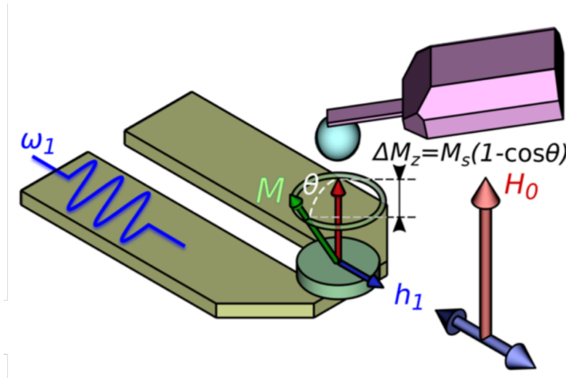
Figure 3.1: Schematics of the experiment. A microwave field \mathbf{h}_1 of pulsation \omega_1 drives the magnetization \mathbf{M} of a nanodisk into FMR, opening a precession angle \theta around the perpendicularly applied field \mathbf{H}_0 . The associated variation in the longitudinal component of the magnetization, \Delta M_z , is mechanically detected by the cantilever of a magnetic resonance force microscope.
