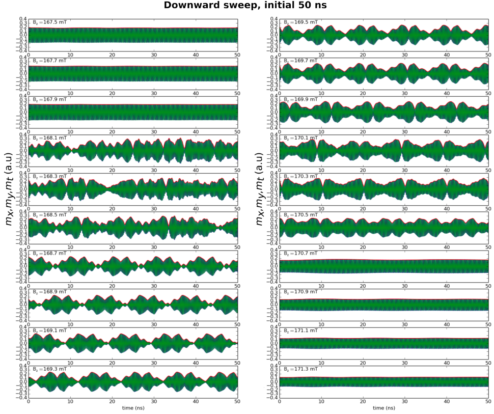
Figure E.2: Zoom on the first 50 ns in time evolution of the components m_x , m_y and m_t of the magnetization at different fields trough the resonance line for the 700 nm disk, each field having been simulated 500 ns. The simulation was done with a downward sweep of the field. For each field, the initial state is the final state of the previous field.
