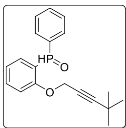
(2-((4,4-dimethylpent-2-yn-1-yl)oxy)phenyl)(phenyl)phosphine oxide
