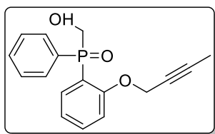
(2-(but-2-yn-1-yloxy)phenyl)(hydroxymethyl)(phenyl)phosphine oxide
