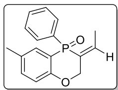
( Z )-3-ethylidene-6-methyl-4-phenyl-2,3-dihydrobenzo[ b ][1,4]oxaphosphinine 4-oxide Chemical Formula: C 17 H 17 O 2 P Molecular Weight: 284.0966 g/mol Yd= 69%
