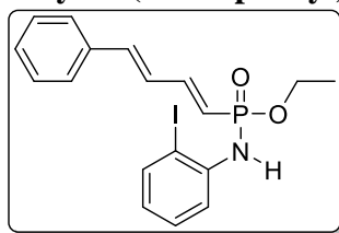
ethyl N -(2-iodophenyl)- P -((1 E ,3 E )-4-phenylbuta-1,3-dien-1-yl)phosphonamidate
