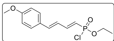
ethyl ((1E,3E)-4-(4-methoxyphenyl)buta-1,3-dien-1-yl)phosphonochloridate Chemical Formula : C 13 H 16 ClO 3 P Molecular Weight: 286.0526 g/mol Yd= 95%
