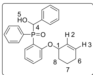
(2-(cyclohex-2-en-1-yloxy)phenyl)(hydroxy(phenyl)methyl)(phenyl)phosphine oxide Chemical Formula: \text{C}_{25}\text{H}_{25}\text{O}_3\text{P} Molecular Weight: 404.1541 g/mol Yd= 68%
