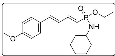
ethyl N -cyclohexyl- P -((1 E ,3 E )-4-(4-methoxyphenyl)buta-1,3-dien-1-yl)phosphoramidate Chemical formula= C 19 H 28 NO 3 P Molecular Weight= 349.1807 g/mol Yd= 50%
