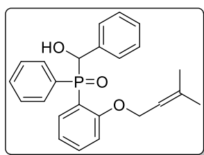
(hydroxy(phenyl)methyl)(2-((3-methylbut-2-en-1-yl)oxy)phenyl)(phenyl)phosphine oxide Chemical Formula: \text{C}_{24}\text{H}_{25}\text{O}_3\text{P} Molecular Weight: 392.1541 g/mol Yd= 75%
