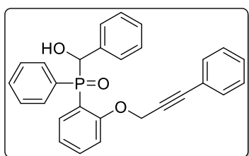
(hydroxy(phenyl)methyl)(phenyl)(2-((3-phenylprop-2-yn-1-yl)oxy)phenyl)phosphine oxide
