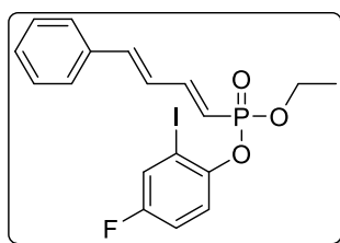
ethyl (4-fluoro-2-iodophenyl) ((1E,3E)-4-phenylbuta-1,3-dien-1-yl)phosphonate
