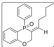
(Z)-3-pentylidene-4-phenyl-2,3-dihydrobenzo[b][1,4]oxaphosphinine 4-oxide
