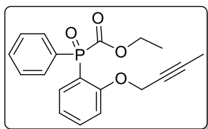
ethyl ((2-(but-2-yn-1-yloxy)phenyl)(phenyl)phosphoryl)formate
