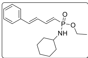
ethyl N -cyclohexyl- P -((1 E ,3 E )-4-phenylbuta-1,3-dien-1-yl)phosphoramidate Chemical formula= C 18 H 26 NO 2 P Molecular Weight= 319.1701 g/mol Yd= 72%
