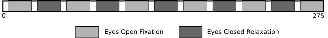
Figure 7.2: Each recording lasts 275 seconds, it alternates between 20 seconds of Eyes Open Fixation (EOF) (6 times), and 20 seconds of Eyes Closed Relaxation (ECR)(5 times) or 20 seconds of Mental Calculus, interleaved with 5 seconds of rest. ECR condition ends with a sound, to inform the participant that he/she has to open his/her eyes.
