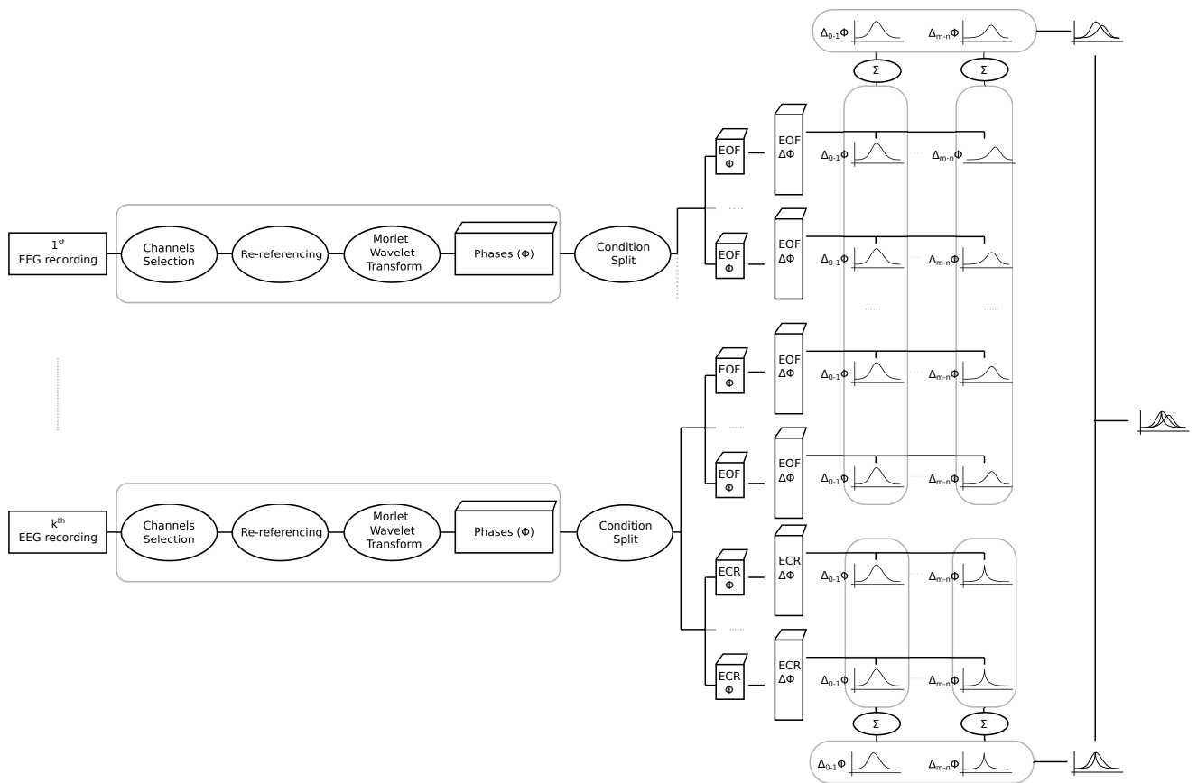
Figure 7.3: The pipeline is presented for a given subject with k recordings. The phase differences are computed on each EEG recording separately and the phase difference histograms are merged in the final steps. For each recording, the channels of interest are selected (O1-P3-C3-F3-Fp1 for instance), these channels are re-referenced (to M1 or M2 for instance), their Morlet wavelet transform is computed with a number of cycles equal to 12 to retrieve the instantaneous phase as a function of time. The phases are split according to whether they occur during the EOF or ECR condition. The phase differences are computed for each pair of channels of the selection with the first one (O1-P3, O1-C3, O1-P3, O1-F3, O1-Fp1), and their histograms are evaluated. All the histograms of a given condition and given pair of electrode are merged together to aggregate all the information. Finally, the EOF and ECR condition are compared.
