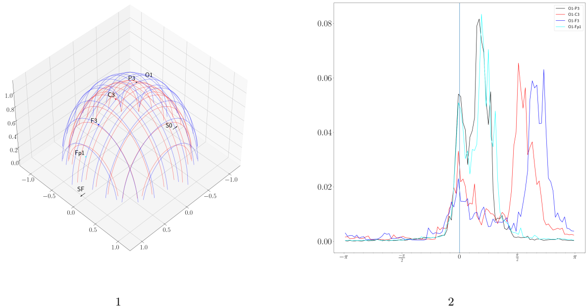
Figure 7.15: Geometry of the traveling wave simulation (1), and associated phase distributions (2). Sources are represented as arrows (SF: Source Frontal, SO: Source Occipital), on the inner red hemisphere. The sources are two sinusoidal waves oscillating at 10 Hz, with added gaussian noise. They are phase shifted from one another by \pi . Electrodes are represented as spheres of different colors (O1, P3, C3, F3, Fp1), on the outer blue hemisphere. Electrodes are placed along the anteroposterior axis, and shifted by \pi/12 with respect to 7.7 toward the nose. The histograms are obtained exactly as in 7.5.
