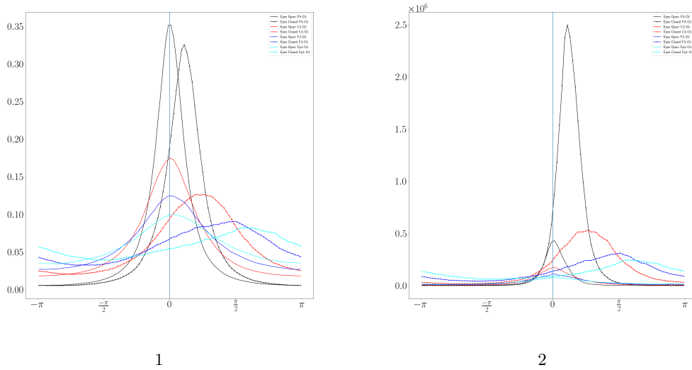
Figure 7.11: 1) Phase difference distributions based on phase difference occurrence only. 2) Phase difference distributions weighted by the amplitude product.
