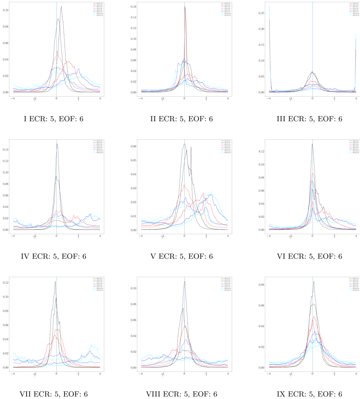
Figure 7.16: Left anteroposterior axis (O1-P3-C3-F3-Fp1). Phase difference distributions retrieved from 9 subjects. Each histogram is computed either over 6 * 20 seconds of EOF, 5*20 seconds of ECR. The channels are referenced at M2.
