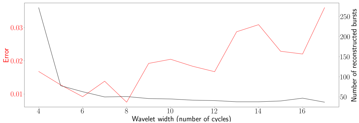
Figure 5.6: Reconstruction error and number of reconstructed bursts with respect to wavelet width, results obtained on an arbitrary 20s segment of EEG during an Eye Closed Relaxation condition (Fp1 electrode referenced at M2).
