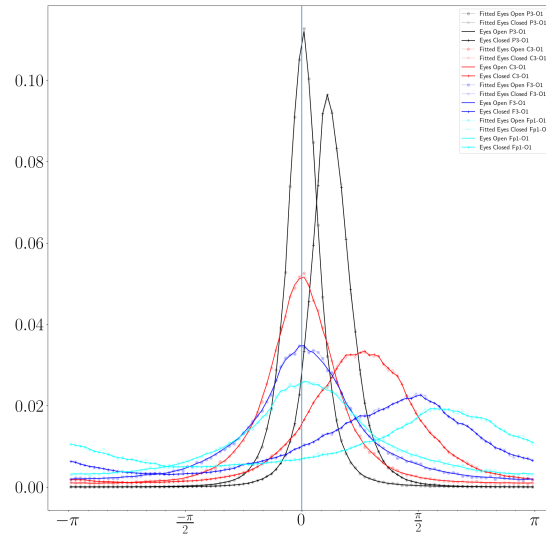
Figure 7.12: Flattened polar empirical probability distribution of phase difference distributions for all periods of either EOF or ECR, accompanied by draws (N=1000) from these empirical probability distributions. The draws are in turn used to obtain the \kappa and \mu parameters of the von Mises distribution by fitting.
