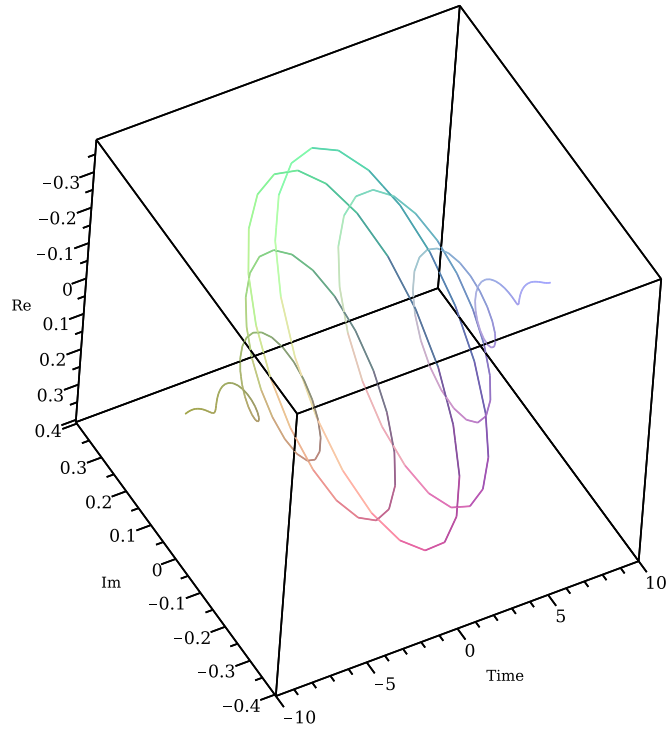
Figure 3.1: Morlet Wavelet w(t) = \frac{\sqrt{2\pi\nu_w}e^{-\frac{\Omega_w^2}{2}}}{\Omega_w} e^{i2\pi\nu_w t} e^{-\frac{2t^2\pi^2\nu_w^2}{\Omega_w^2}} . Time: t . \Im(w(t)) and \Re(w(t)) are represented as a function of time. It oscillates at 3 Hz in the complex plane ( \nu_w = 3 ), with a width( \Omega_w ) of 10.
